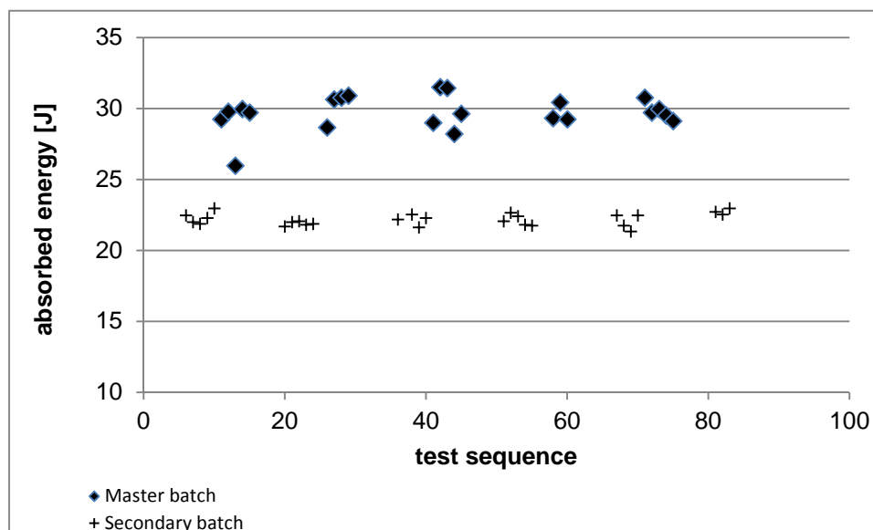
Figure 3: Absorbed energy values of 26 test pieces of ERM ® -FA013bp, compared with 22 test pieces of ERM ® -FA013ba; data are displayed in the actual test sequence.
