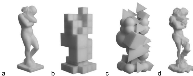
Figure 3. Steps of faceting the given sculpture: a) initial shape (scanned model "Eve", Three D Scans repository, http://threedscans.com ); b) corresponding octree; c) associated primitive solids; d) rotated and scaled facets combined with manipulated initial mesh.
