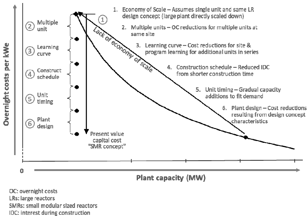
Figure 3: Generic view of factors affecting comparative costs of small modular reactors (SMRs) and large reactors (LRs). Source: IAEA, 2013
