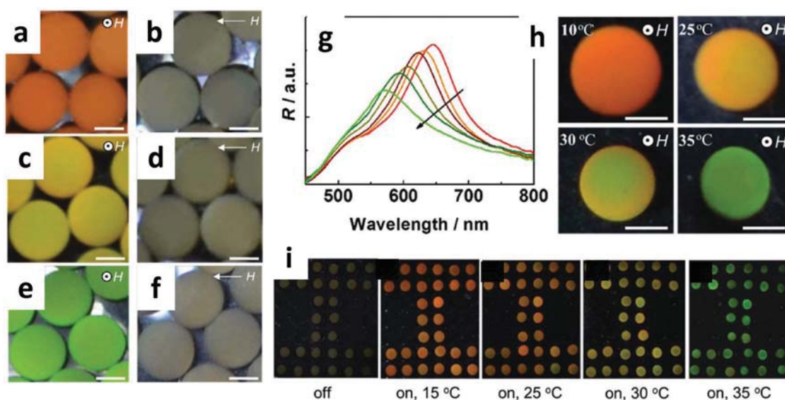
Figure 12. Digital photos of the \text{Fe}_3\text{O}_4@PVP\text{-PNIPAM} balls polymerized under magnetic field of a,b) 105 G s, c,d) 175 G s, and e,f) 340 G s, respectively, at magnetically switching a,c,e) “on” and b,d,f) “off” states. All the scale bars are 1 mm. g) Reflection spectra of the same balls polymerized under a 105 G s magnetic field along the arrow when the temperature is increased from 10 to 35 °C with a step of 5 °C. h) The typical digital photos at different temperatures. All scale bars are 1 mm. i) Digital photos of a bead pattern filled with the same balls formed under 105 G s at “off”/“on” states by rotating the external magnetic field between 0° and 90° at various temperatures. Reproduced with permission. [43] Copyright 2017, Royal Society of Chemistry.
