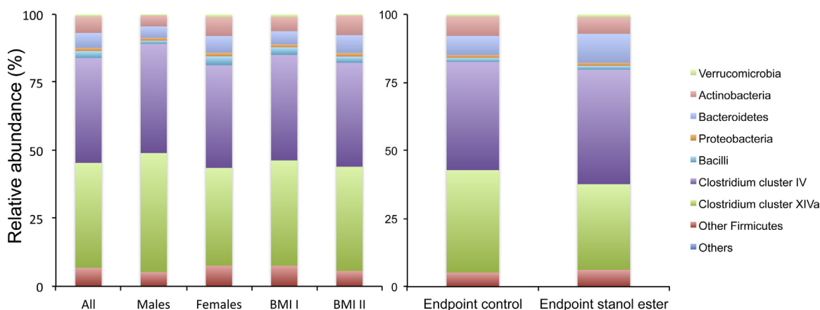
Fig. 2. No difference in relative abundances of microbial phyla at baseline and after consumption of control or plant stanol ester enriched margarine. Data is presented for all subjects and for gender and BMI category (BMI I: \leq 25 and BMI II: >25 kg/m 2 ) at baseline (left) and at the end of both intervention periods (right).
