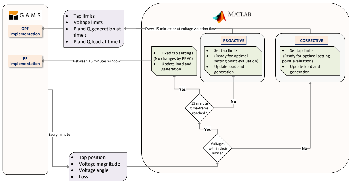
Figure 2: PPVC implementation using MATLAB and GAMS
