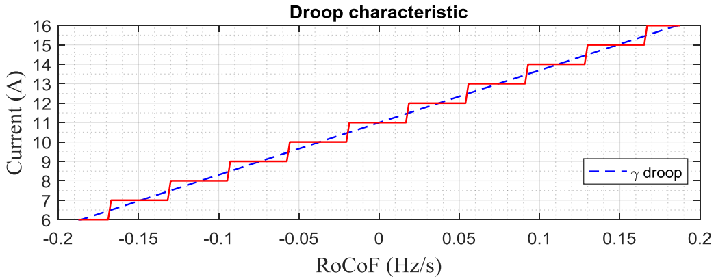
Figure 7: IRPC droop
