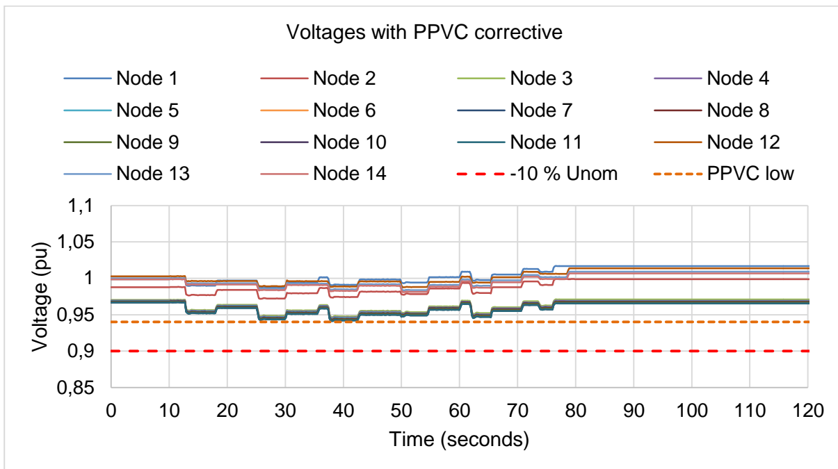
Figure 22: PPVC corrective simulation results
