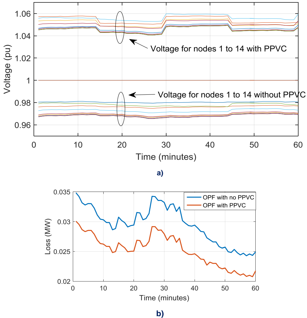
Figure 5: Effects of the implementation of PPVC on the voltage levels (a) and network losses (b)
