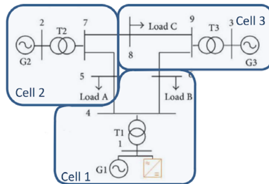
Fig. 1. IEEE 9-Bus system and cells
