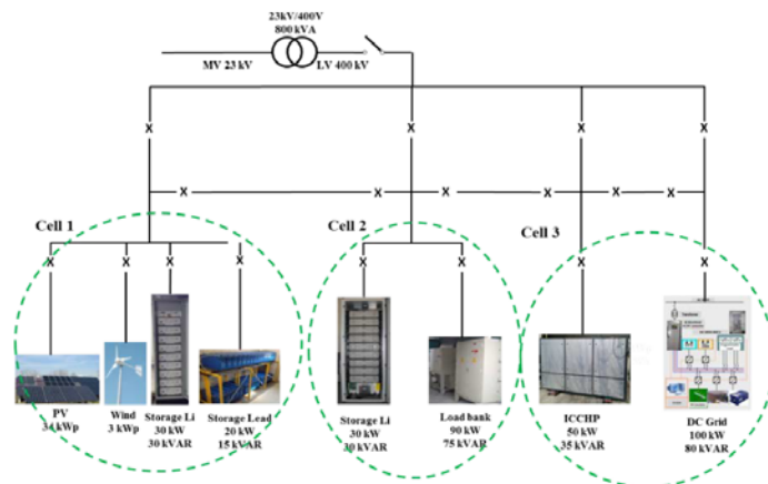
Fig. 1 - RSE DERTF lab
