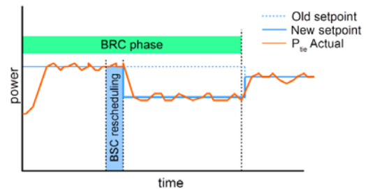
Fig. 1. Corrective tie-line setpoint adjustment
