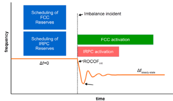
Fig. 1. Combined IRPC and FCC response
