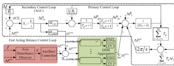
Fig. 4. BRC- Enhanced Load Frequency Control
