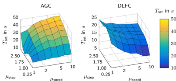
Fig. 3: Performance AGC vs. DLFC (lower is better).
