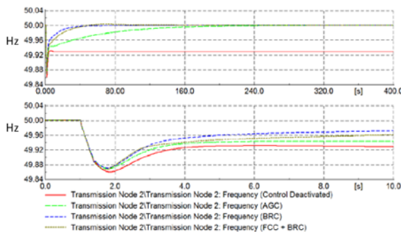
Fig. 4. FCC/BRC impact on frequency response.
