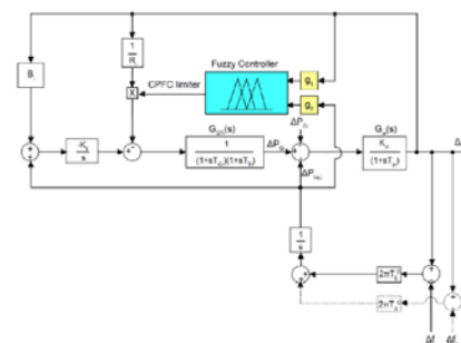
Fig. 2. Frequency Containment Control.
