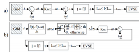
Fig. 1. (a) FCC control diagram, (b) IRPC control diagram
