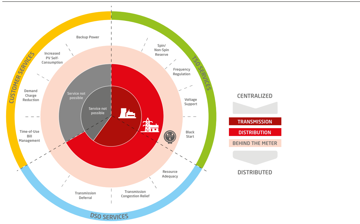
Figure 6. Battery energy storage can provide different services to three stakeholder groups (TSO, DSO and customers) depending on the connection point of the storage unit: in the transmission grid, in the distribution grid, or behind the meter. After [17].
