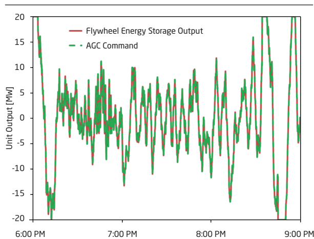
Figure 3. The reaction of a flywheel (MW input/output) in response to signals from the automatic generation control. It can be seen that, within the accuracy of the graph (note the axis scaling), the flywheel follows the signals completely. Source: Beacon Power.
