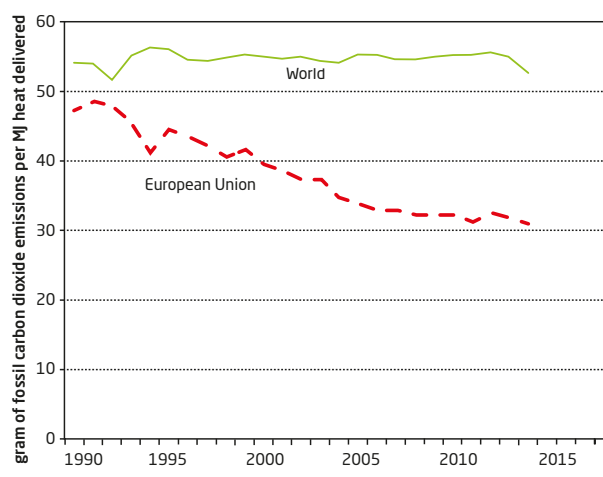
Figure 1. Estimated specific carbon dioxide emissions 1990-2014 from all district heating systems in the world and in the current European Union. [1].
