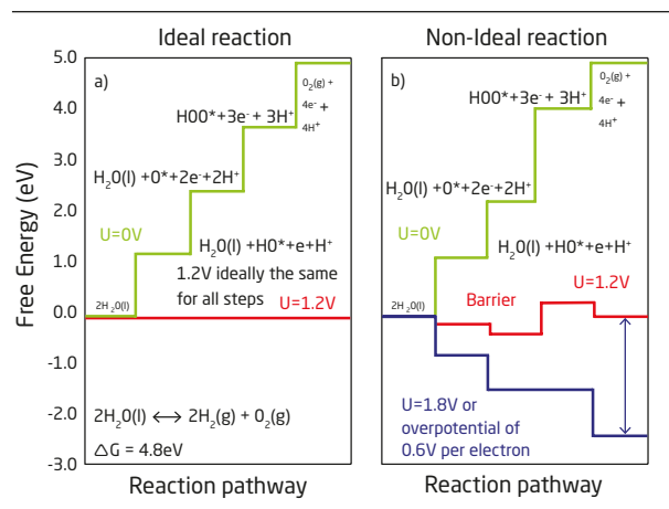
Figure 3. Schematic free energy diagram for water splitting. a) displays the ideal case where all intermediates are bond equally strong, while b) shows a more realistic case where an overpotential of 0.6 V occurs due to a too strong bonding of atomic oxygen. Reproduced from ref [6]).
