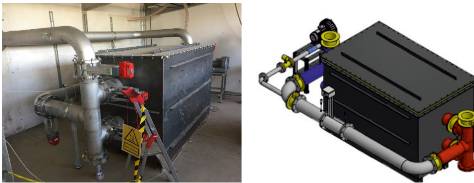
Figure 9. Photo and drawing of test facility for High Temperature Thermal Energy Storage at DTU. The facility contains a 1.5m 3 rock bed.
