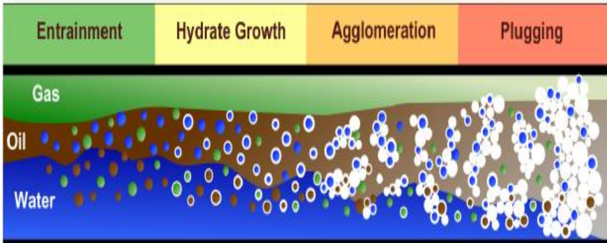
Figure 1. A conceptual model for hydrate formation (Source: Turner [8])
