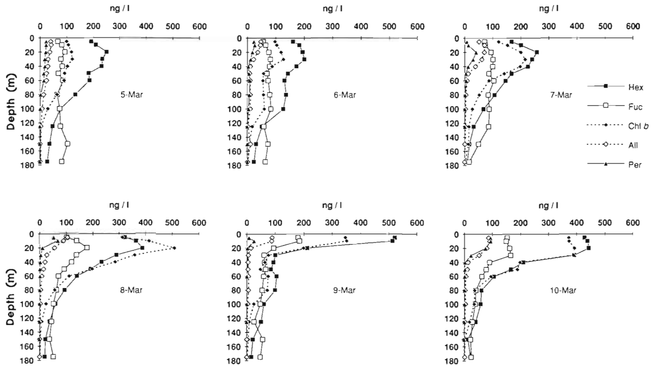
Fig. 8. Profiles of the concentrations of 5 selected pigments in the upper 180 m for 5 to 10 March. Hex: 19'-hexanoyloxyfucoxanthin, Fuc: fucoxanthin; Chl b : chlorophyll b ; All: alloxanthin; Per: peridinin
