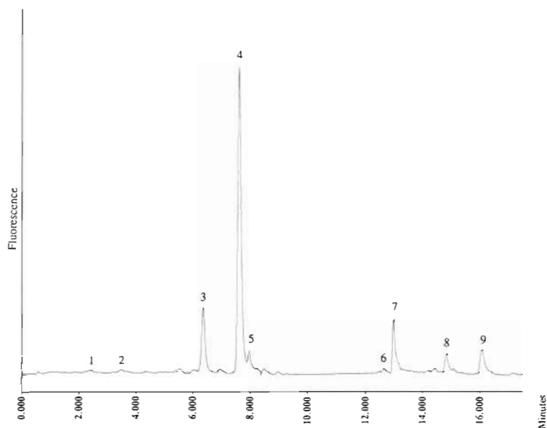
Fig. 3. HPLC fluorescence chromatogram of a 100 m trap sample collected over 6 and 7 March. Pigment identities are: (1) chlorophyllide a_1 , (2) chl c_1c_2 , (3) phaeophorbide a_1 , (4) phaeophorbide a_2 , (5) unknown, (6) chl a allomer, (7) chl a , (8) phaeophytin a_1 , (9) phaeophytin a_2
