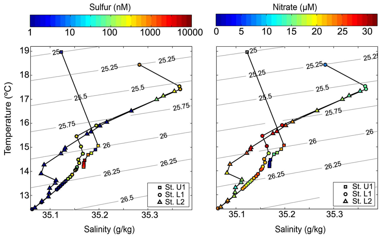
Supplementary Figure 2: Elemental sulfur and nitrate concentrations as a function of temperature-salinity for Stations U1, L1 and L2. Densities ( \text{kg m}^{-3} ) are indicated by the light gray isopycnals.
