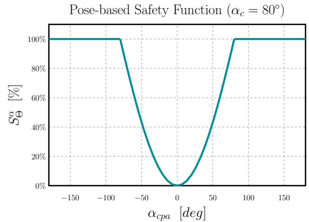
Fig. 7. COLREGS pose-based safety functions can be used to give preference to passing contacts with relative bearing and contact angle that are least likely to increase risk of collision. This safety function shows S_\Theta^\alpha that favors beam and stern contact angles at CPA ( \alpha_{\text{cpa}} ) using Equation (5). Here, a cutoff angle \alpha_c = 80^\circ gives equal preference to beam and stern aspects. Pointing the bow ( 0^\circ ) results in a pose-based safety score of S_\Theta = 0 .
