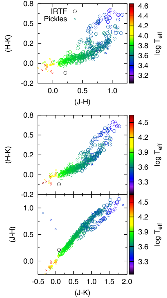
Fig. 16. Colour–colour diagrams of the stars in the IRTF spectral library, compared with the Pickles library (which is assumed to have solar metallicity).
