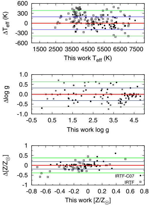
Fig. 14. Residuals from the comparison between the stellar atmospheric parameters for the stars in the IRTF spectral library and those compiled by Cesetti et al. (2013; present work – Cesetti) . The circles represent the values for the IRTF stars with C07 stellar parameters and the squares the IRTF stars for which we determined their parameters. The red line is the one-to-one correlation. The blue and green lines mark the 1\sigma and 2\sigma confidence intervals, respectively.
