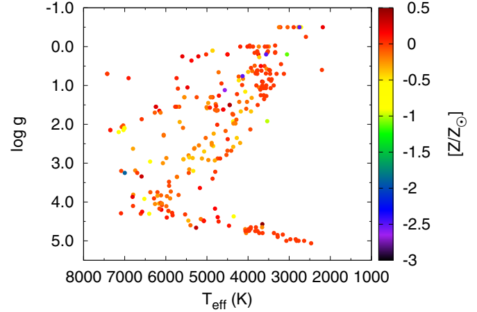
Fig. 12. Stellar atmospheric parameters for the stars of the IRTF spectral library. This shows the parameter coverage of this library for stellar population models. L- and T-type dwarfs were not included.
