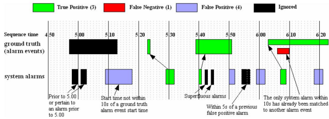
Fig. 5. Iilids Event Detection evaluation
