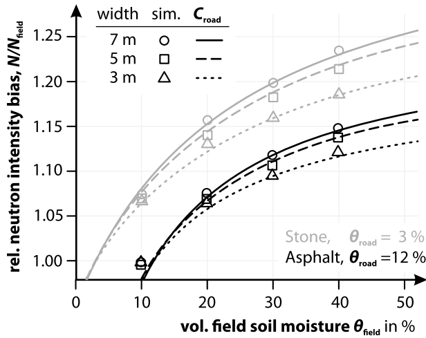
Figure 4. URANOS simulations (symbols) and fitted correction functions C_{road}(\theta_{field}, \theta_{road}, w, r) (lines) representing the neutron bias on roads of various widths through fields of different soil moisture. Shown for stone roads (grey) and asphalt roads (black). The quality of fit is in the range of \pm 0.01 except for rare cases with \theta_{field} < \theta_{road} .
