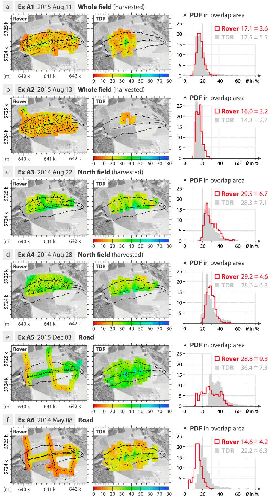
Figure 7. Comparison of CRNS Rover and TDR campaigns in the Schäferfirtal using interpolated data, and the probability density functions (PDF) of soil moisture in their overlapping area. See also the corresponding scatterplots in the supporting information.
