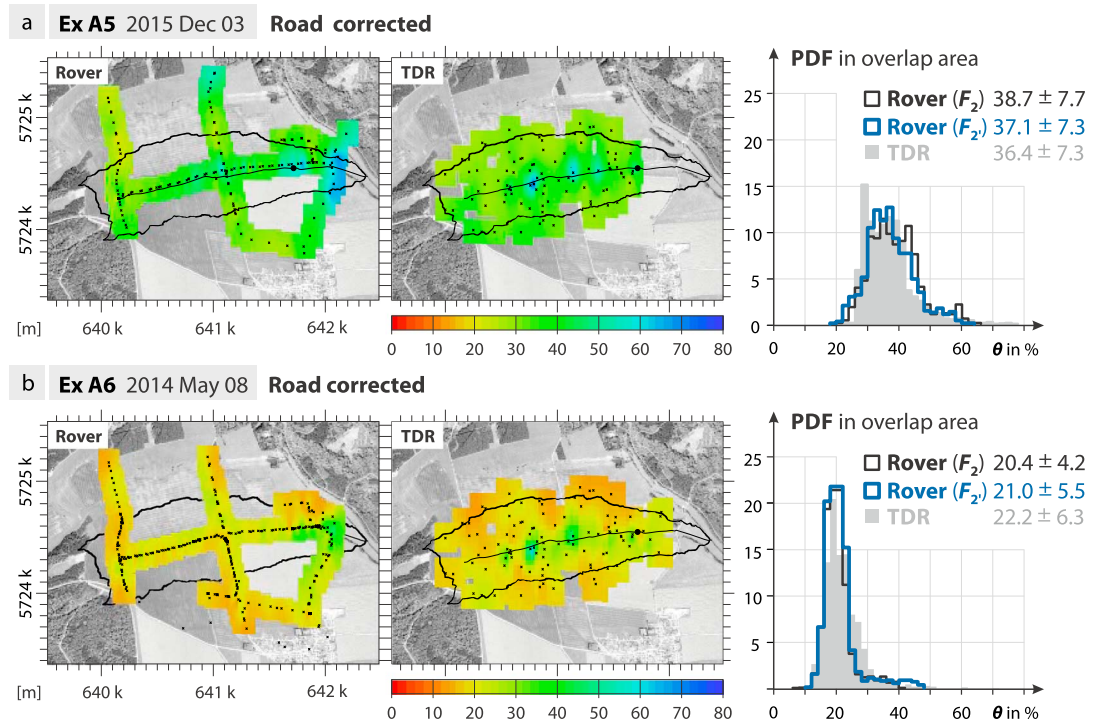
Figure 8. Application of the road correction approach on the road-only surveys in the Schäfertal (compare Figures 7e and 7f). Patterns of (left) the rover agree well with those from (middle) TDR in terms of (right) the probability density function in the overlap area of both interpolated grids, their mean, and standard deviation. The correction is tested with two approaches of the moisture term: (1) F_2(\theta_{\text{field}} = \langle \theta_{\text{TDR}} \rangle) (equation (5)) using the average of the TDR data (black line) and (2) F_2'(\theta(N)) (equation (6)) using uncorrected neutron counts as a proxy (blue line). Kriging results using the former approach were almost identical to those using the latter approach, so that only the latter is shown in the left plot. Corresponding scatterplots are presented in the supporting information.
