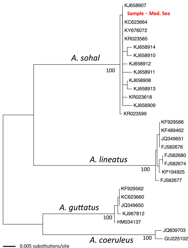
Figure 3. Phylogenetic relationships of Acanthurus sequences. The Neighbour-Joining method was used to identify the phylogenetic relationships of the putative A. sohal sample (in red, noted as sample – Med Sea) and sequences obtained from GenBank. Tree labels correspond to Genbank Accession numbers. Numbers by the nodes correspond to bootstrap support, and species names of GenBank sequences are presented above the corresponding branches.
