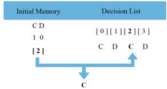
Figure 2: Initial Memory and the Decision List During a single iteration of Prisoner's Dilemma, a player chooses to cooperate (C) or defect (D) based on its decision list. Defect is represented with a 0 and cooperate with a 1. In this example, the initial memory is CD, which is represented as the binary number 10 (i.e. 2, in decimal). This points to index 2 in the decision list, which contains a C, so this player will cooperate in this iteration.
