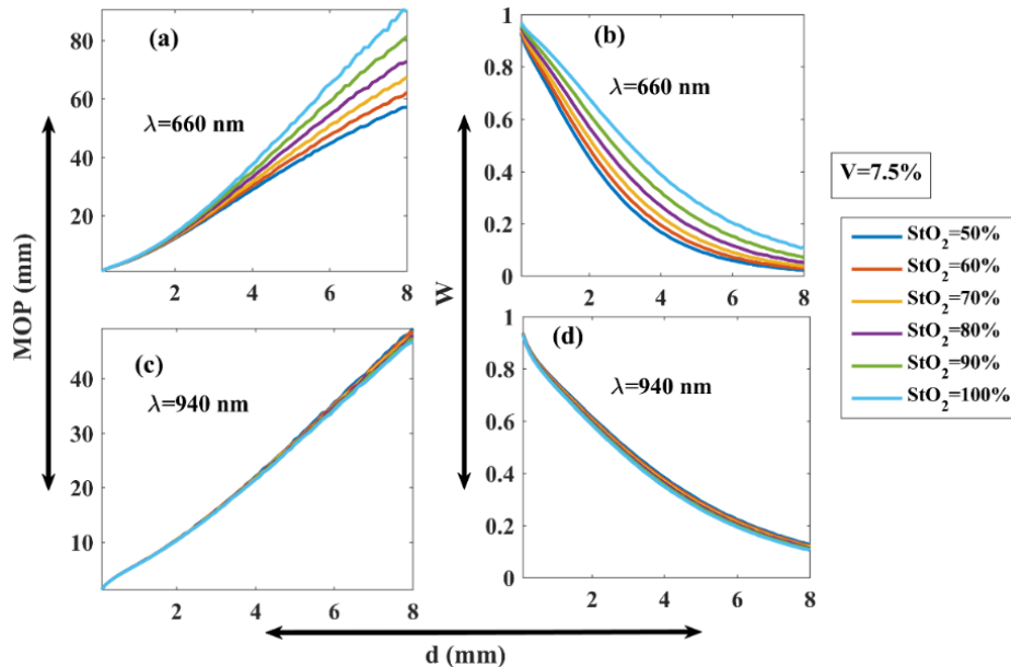
Figure 7. Mean optical path ( MOP ) and relative reflectance ( W ) of photon packets as functions of source-detector separation ( d ) are shown at a fixed V = 7.5\% for StO_2 = 50\text{-}100\% respectively for \lambda = 660\text{ nm} in (a) and (b); and for \lambda = 940\text{ nm} in (c) and (d) respectively.
