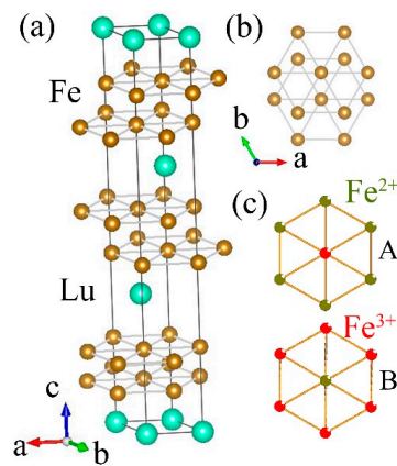
Figure 1. (a) The crystal structure of LuFe 2 O 4 . (b) Two adjacent triangular FeO 5 layers shifted by \sqrt{3}/3 a within the ( ab ) plane. (c) The Fe 2+ - (A) and Fe 3+ -rich (B) monolayer charge models. Oxygen ions are omitted for clarity.
