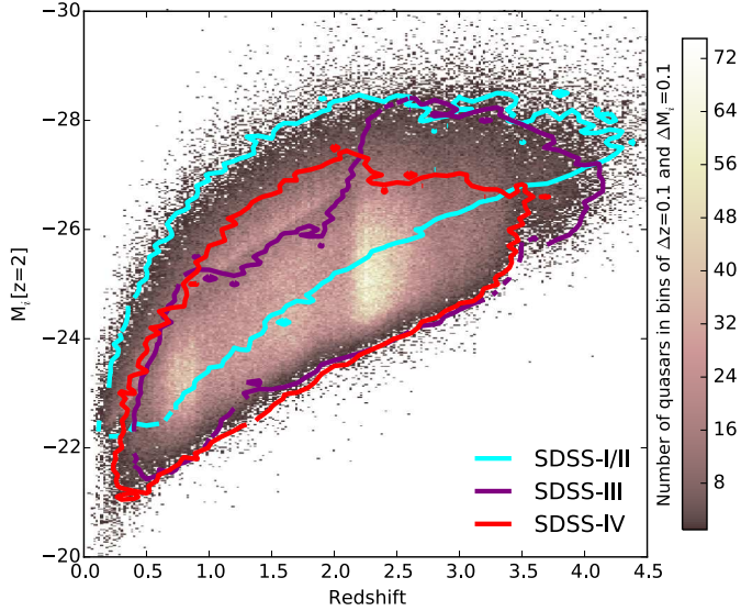
Fig. 7. Density map of the DR14Q quasars in the L-z plane. The color map indicates the number of DR14Q quasars in bins of \Delta z = 0.1 and \Delta M_i [z = 2] = 0.1 . Colored contours correspond to the envelope in the L-z plane for each iteration of SDSS. The absolute magnitudes assume H_0 = 70 \text{ km s}^{-1} \text{ Mpc}^{-1} and the K-correction is given by Richards et al. (2006), who define K(z = 2) = 0 .
