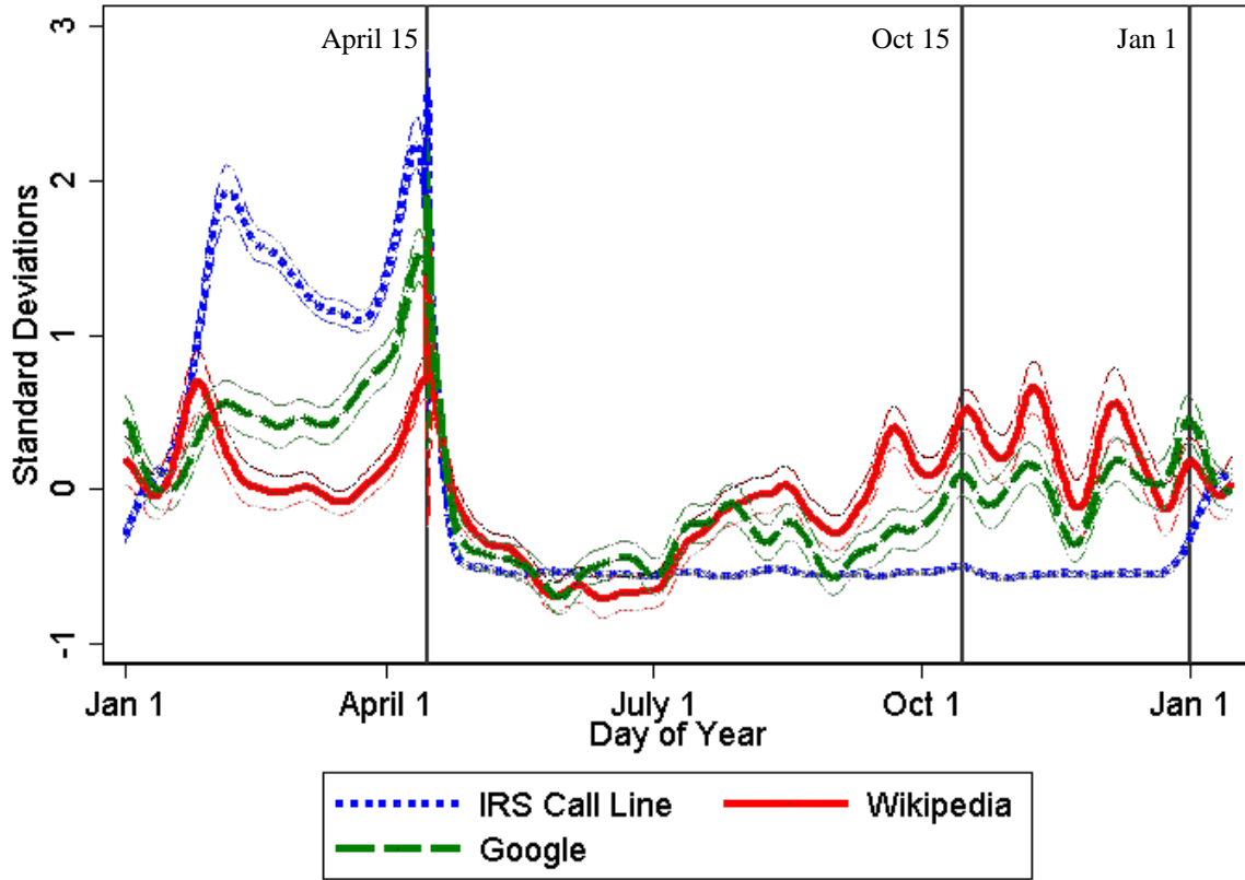
FIGURE 2: YEARLY SEASONALITY
