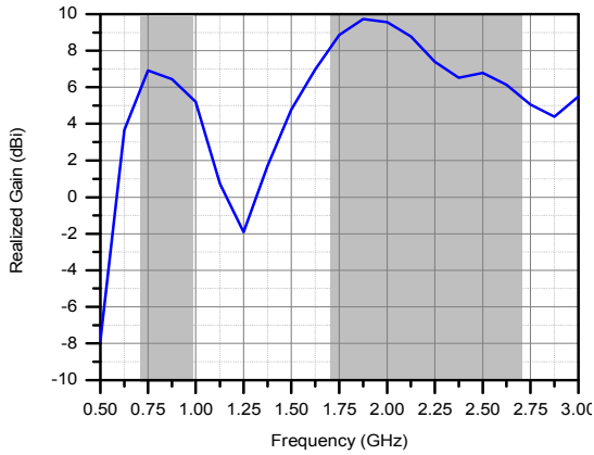
Fig 5. Realized gain of the proposed antenna
