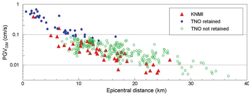
Fig. 3. Geometric mean horizontal PGV values from the KNMI and TNO accelerographs from the M_L 3.1 2015 Hellum earthquake, showing the censoring effect of the trigger threshold on the household instruments. The green dots are PGV values reported as part of the ‘heartbeat’ monitoring that transmits the highest velocity value recorded in each minute; the time-histories corresponding to these records are not retained.
