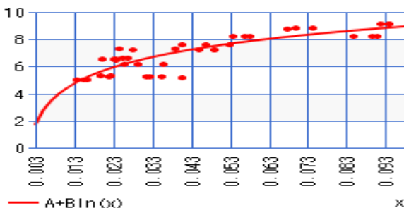
Fig. 7. Logarithmic regression.
