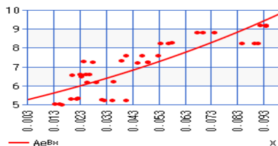
Fig. 8. e-Exponential Regression .
