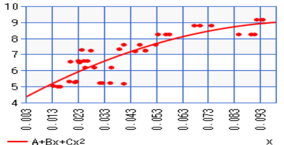
Fig. 9. Quadratic regression.
