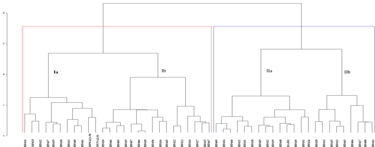
Fig. 2. Clustering of genotypes based on Agglomerative clustering method.
