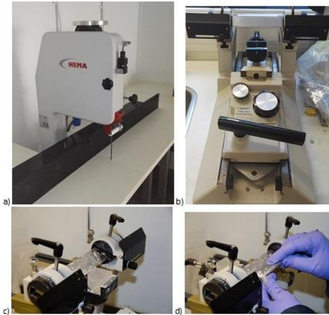
Figure 3.04: Photos taken of the cold room sampling set-up. From top left: (a) the band saw; (b) a front profile of the microtome system; (c) a section of ice held in the mantle system of the microtome during sampling; (d) Collecting a discretely-cut sample on the microtome blade using a sterile pipette tip.
