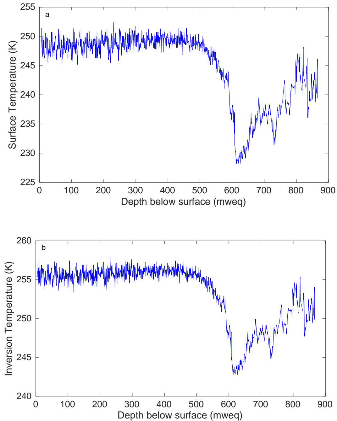
Figure A1.03: (a) Surface Temperature reconstruction using eq. 2.03 (stable water isotope profile measured prior to this project); (b) Inversion Temperature for the BI ice core reconstruction using eq. 2.04 (stable water isotope profile measured prior to this project).
