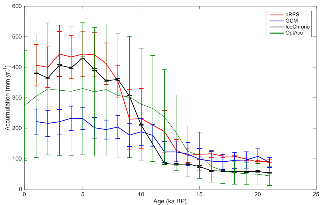
Figure 4.17: Accumulation estimates for each millennium for comparison with GCM estimates. Crosses at each modelled data point represent the associated uncertainty for each estimate. The results present the freely-calculated IceChrono and the Clausius-Clapeyron-derived OptAcc approaches.
