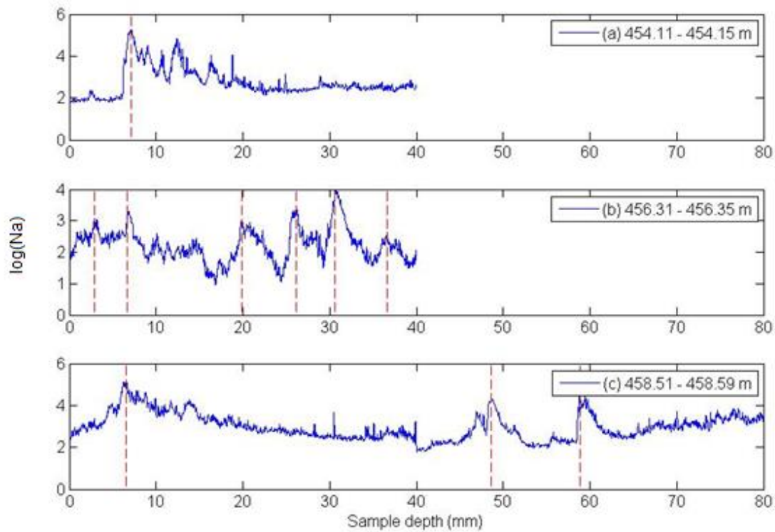
Figure 5.03a – c: LA ICP-MS profiles for three sections of sample from 454 – 459 m; semi logarithmic plots show the \log(\text{Na}^+) on a common depth scale with red dashed lines delineating a seasonal peak.
