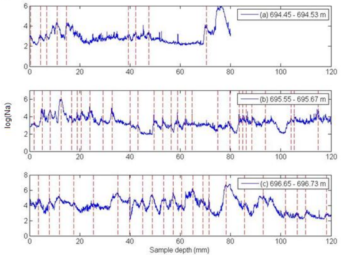
Figure 5.04a – c: LA ICP-MS profiles for three sections of ice from 694-697 m; semi logarithmic plots show the \log(\text{Na}^+) on a common depth scale with red dashed lines delineating a seasonal peak.
