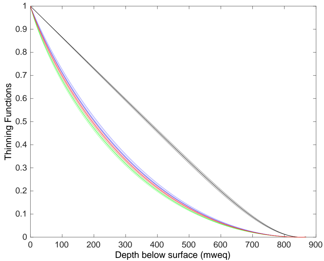
Figure A1.17: Reconstructed thinning functions for the BI ice core using the Direct Search model. Each scenario uses a different initial accumulation profile: red: Clausius-Clapeyron; blue: Simple Exponential; green: Arrhenius; black: IceChrono. Each scenario has an associated uncertainty presented in a pale shade of the presented colour.
