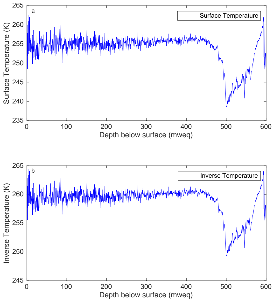
Figure 4.02: (a) Reconstructed surface temperature using eq. 2.03 using the stable water isotope profile obtained prior to this research project (section 2.5.1); (b) Reconstructed temperature at the inversion layer with respect to depth below the surface (mweq) using eq. 2.04 using the stable water isotope profile obtained prior to this research project (section 2.5.1). In both plots, a higher temperature at ~580 mweq that steadily decreases towards 500 mweq likely relates to the cooling from the last interglacial to the last glacial period. Furthermore, a sharp increase in temperature from ~500 mweq to 400 mweq is likely to be the transition from the Last Glacial Maximum (LGM) to the Holocene.
