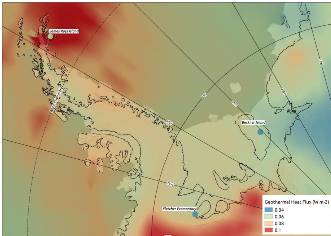
Figure 8.05: Mean GHF values calculated from three sources compared with the measured GHF values at each ice-core site with the locations of the three deep boreholes overlaid, demonstrating the contrast between modelled and derived GHF values. Site locations are denoted using the same colour scheme as used in the map.
