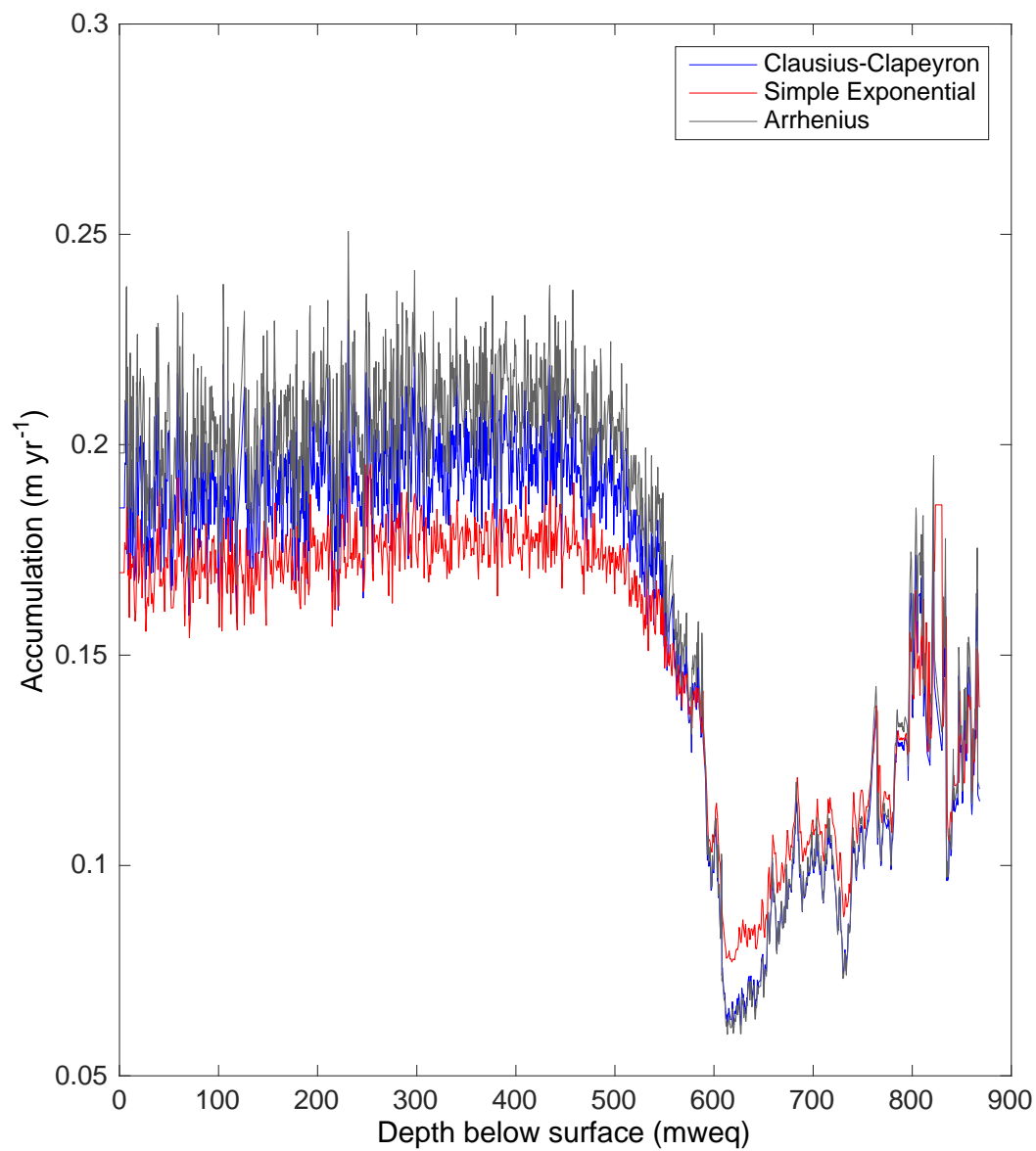
Figure A1.05: Accumulation reconstructions for the BI ice core. Accumulation reconstructions use stable water isotope profiles obtained separate to this research project.
