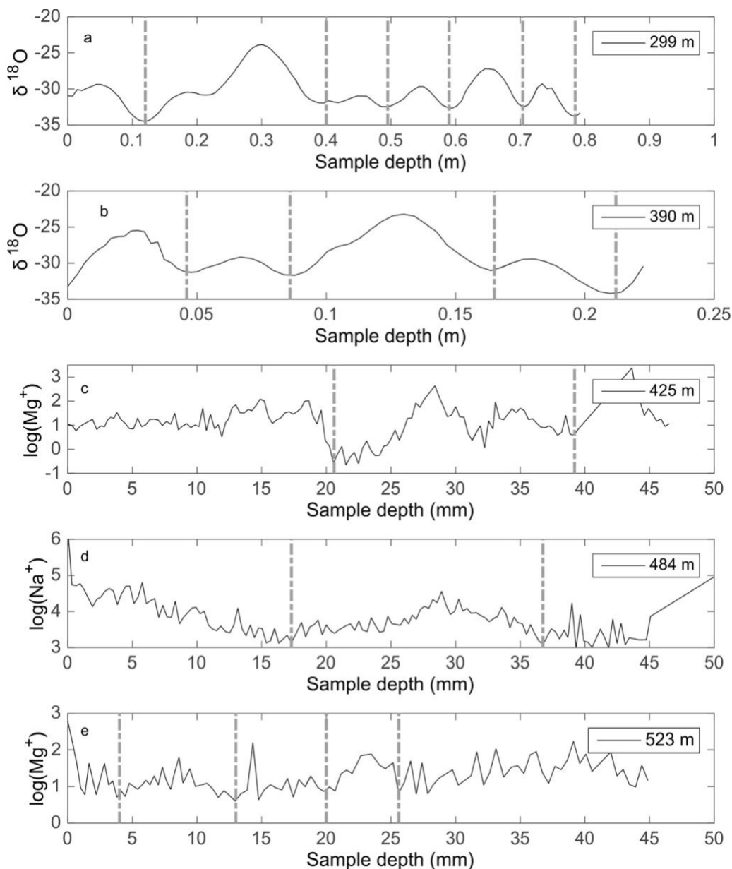
Figure 6.01: Sub-annual measurements on the Fletcher Promontory ice core. A-B: stable water isotope measurements with respect to depth in metres (snow); C-E: ion profiles with respect to depth in millimetres (snow). Dashed lines delineate assumed annual peaks in deposition. Measurements in plots (a-b) were obtained separate to this study by Amy Pike. Measurements in plots (c-e) were obtained by this study using discrete sampling techniques.
