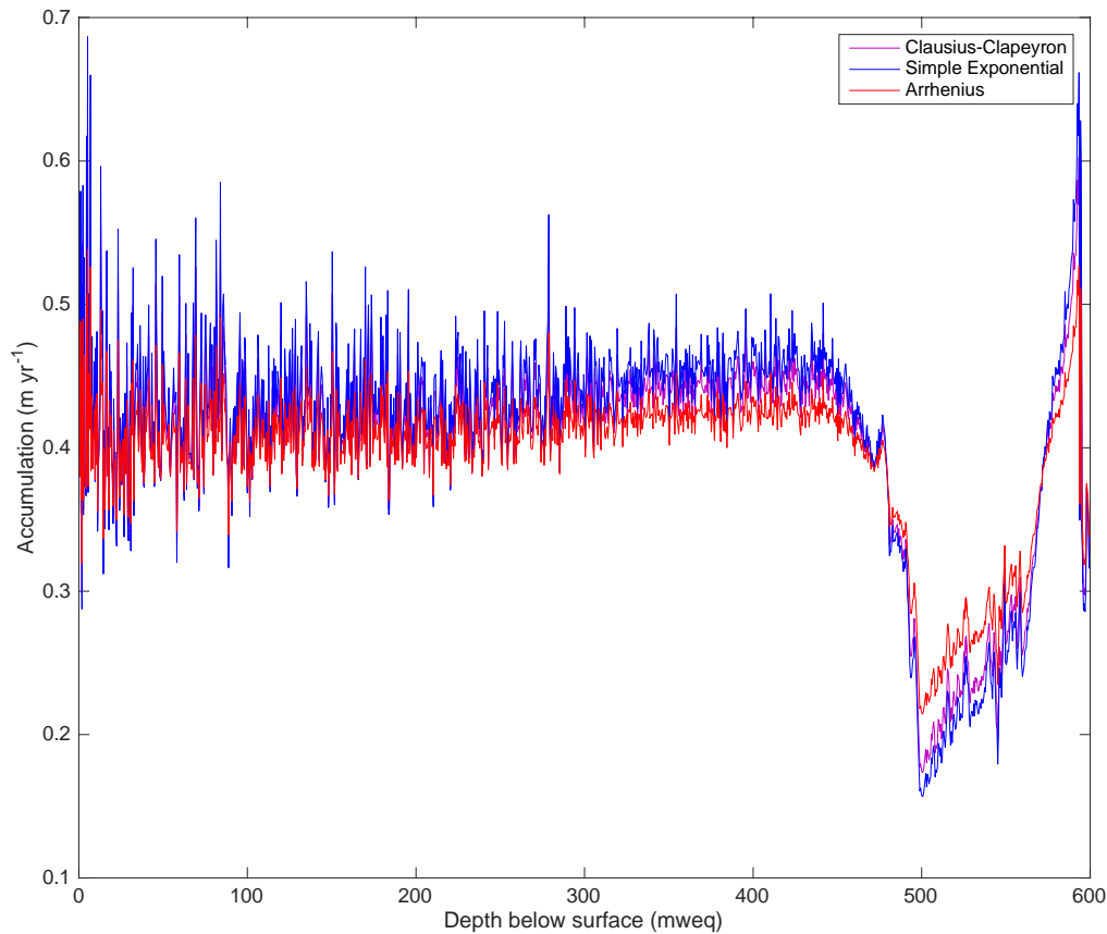
Figure 4.03: Accumulation reconstructions using empirical relationships using the stable water isotope profile obtained prior to this research project.
