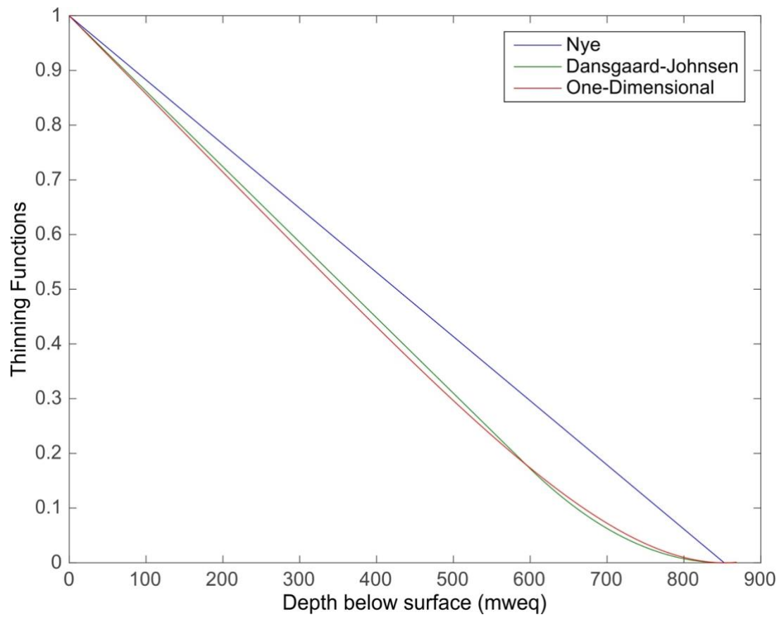
Figure A1.07: Thinning Functions for the BI ice core.
