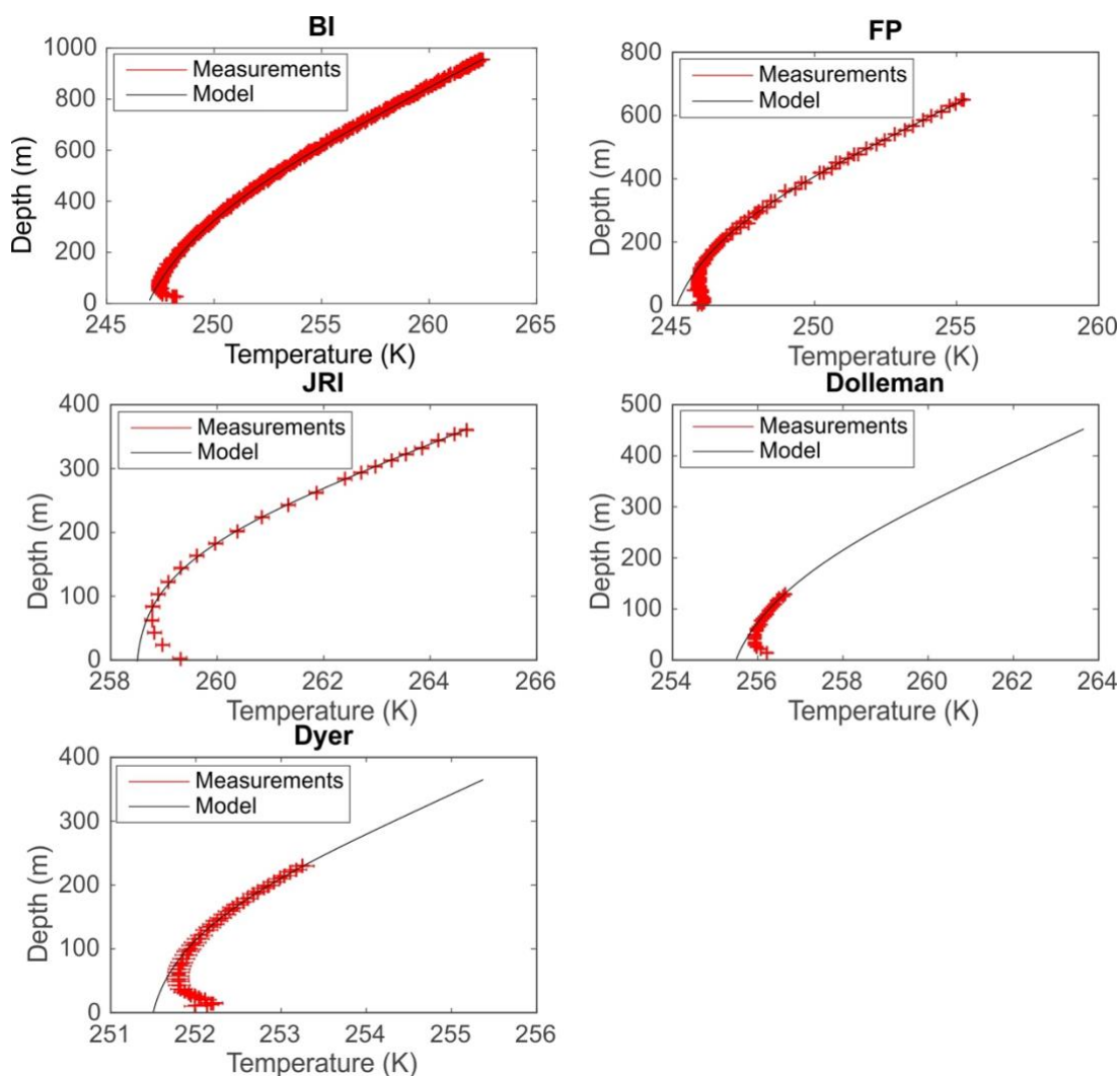
Figure 8.06: Borehole temperature reconstructions (black line) for each borehole site, with measured borehole profiles in red crosses. Measured borehole temperature profiles provided by Rob Mulvaney (pers. comm.).
