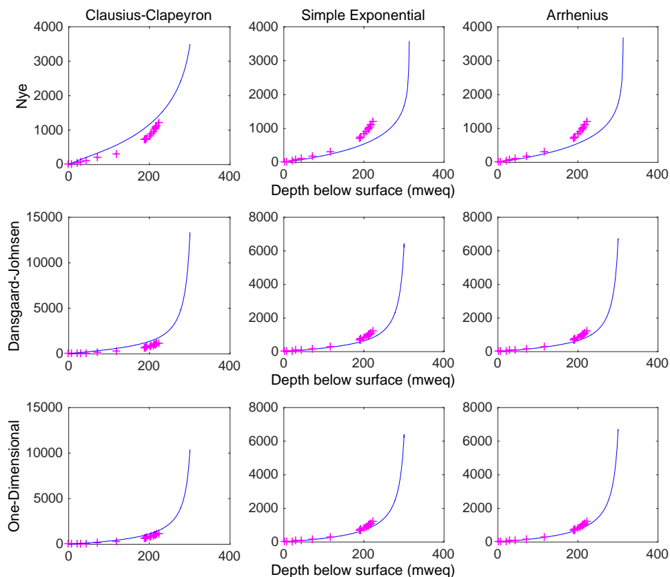
Figure A1.10: Age-Depth Combinations using all forward accumulation and thinning reconstructions for the JRI ice core. Figure laid out as a table.
