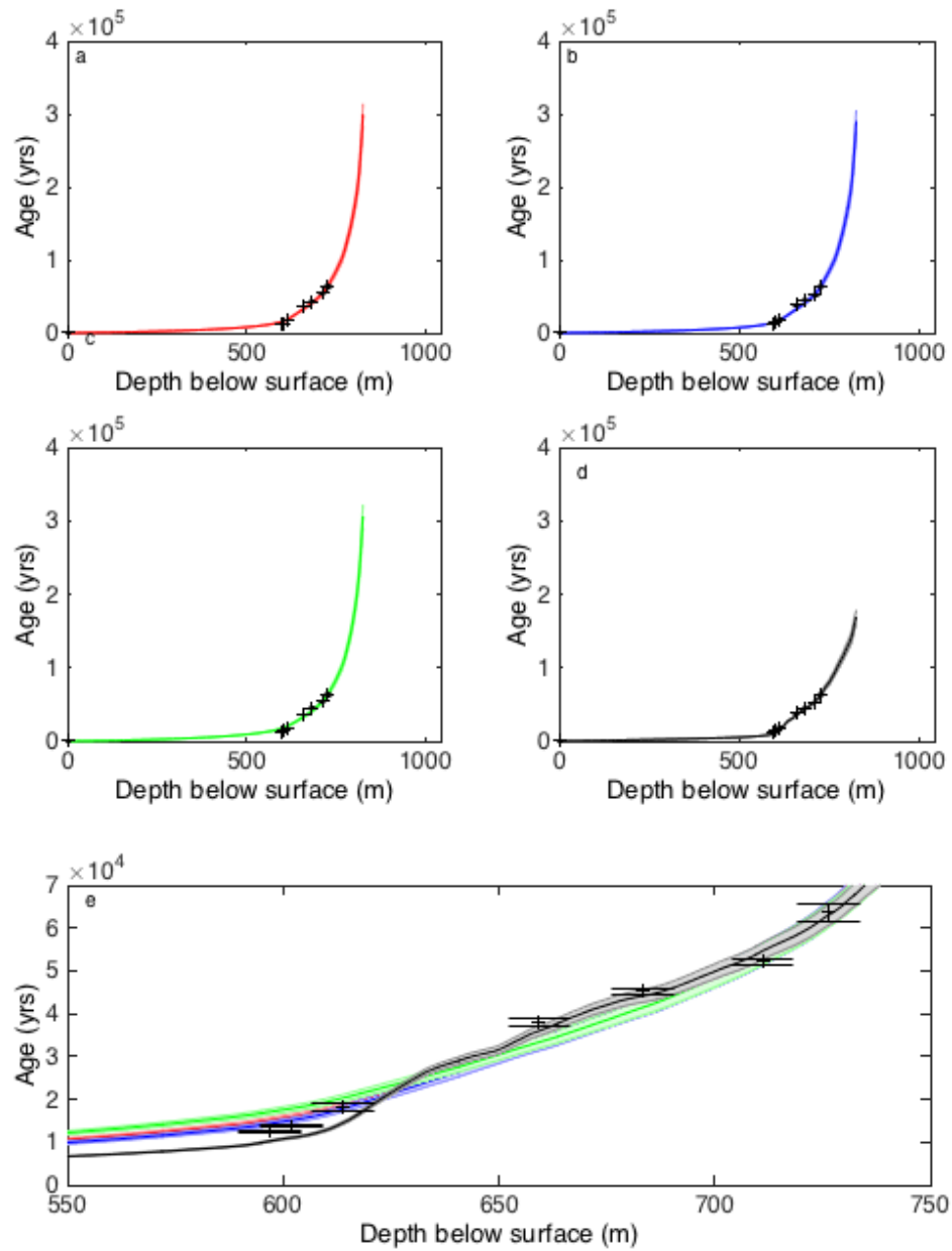
Figure A1.18: Age-Depth reconstructions for the BI ice core using the Direct Search model. Each scenario uses a different initial accumulation profile: red: Clausius-Clapeyron; blue: Simple Exponential; green: Arrhenius; black: IceChrono. Each scenario has an associated uncertainty presented in a pale shade of the presented colour; known-age horizons and the associated uncertainty are presented as black crosses.
