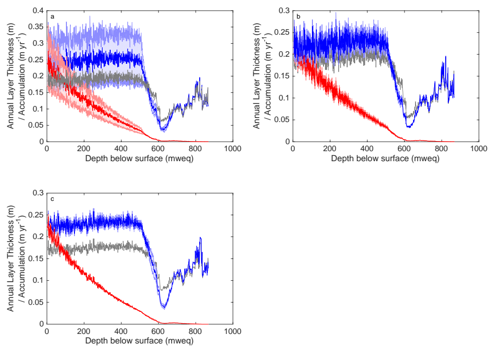
Figure A1.21: Original (red with the confidence interval in pale red) and present-day annual layer thickness (blue with the confidence interval in pale blue) reconstructions using different initial accumulation profiles and perturbed using the Optimised Accumulation and Thinning model for BI. Initial accumulation history (grey) from top left: (a) Clausius-Clapeyron, (b) Simple Exponential, and (c) Arrhenius.
