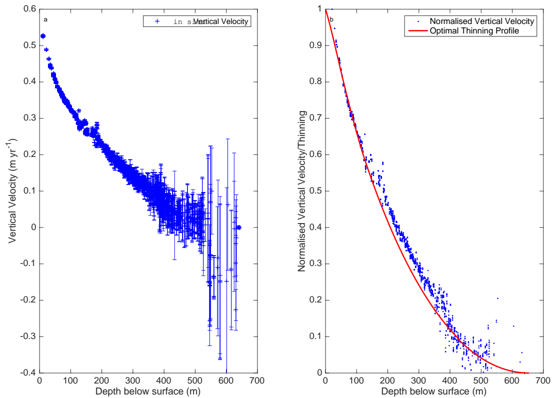
Figure 6.14: (a) Vertical velocity measurements with the associated error margin using pRES at the FP ice core site. Data courtesy of J. Kingslake; (b) Normalised pRES measurements (blue) and the optimal thinning profile calculated using the OptAcc model (red).
