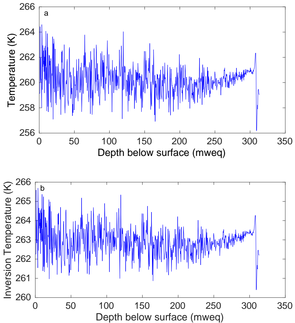
Figure A1.04(a) Surface Temperature reconstruction using eq. 2.03 (stable water isotope profile measured prior to this project); (b) Inversion Temperature for the JRI ice core reconstruction using eq. 2.04 (stable water isotope profile measured prior to this project).
