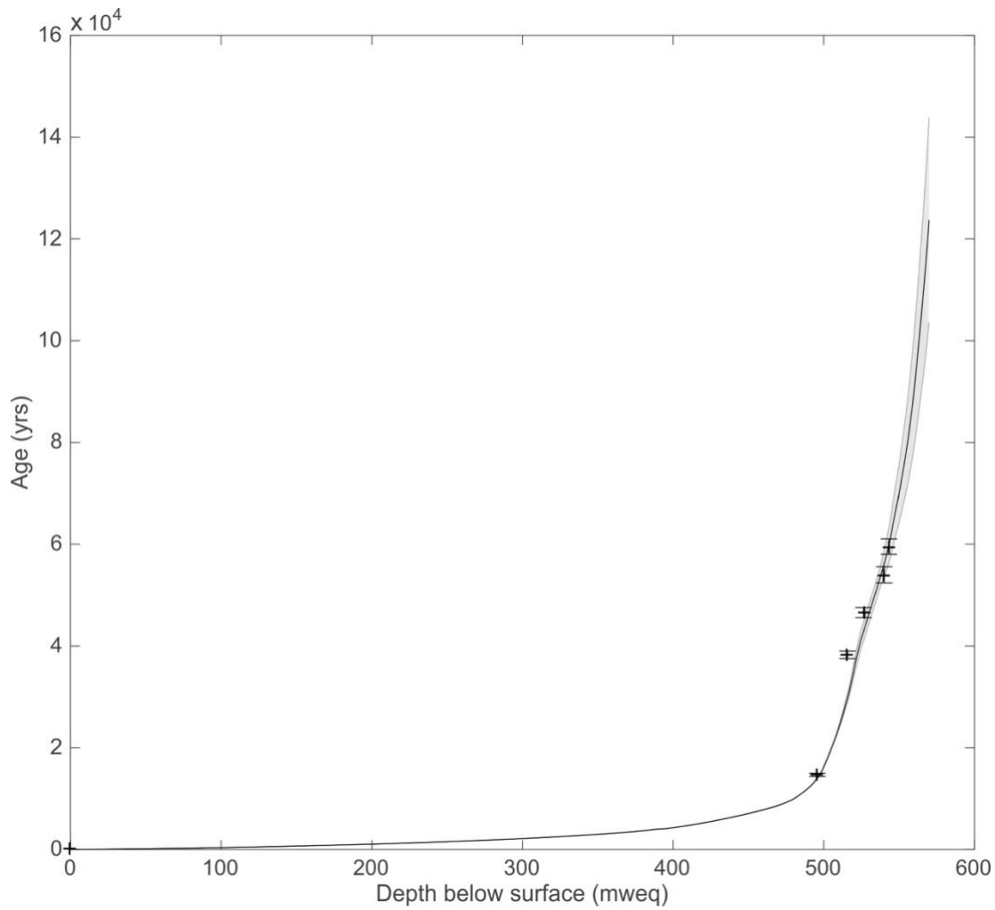
Figure 4.14: Age-depth profile using an empirical age-depth model based on pRES data with uncertainty (grey) and age horizons (black crosses).
