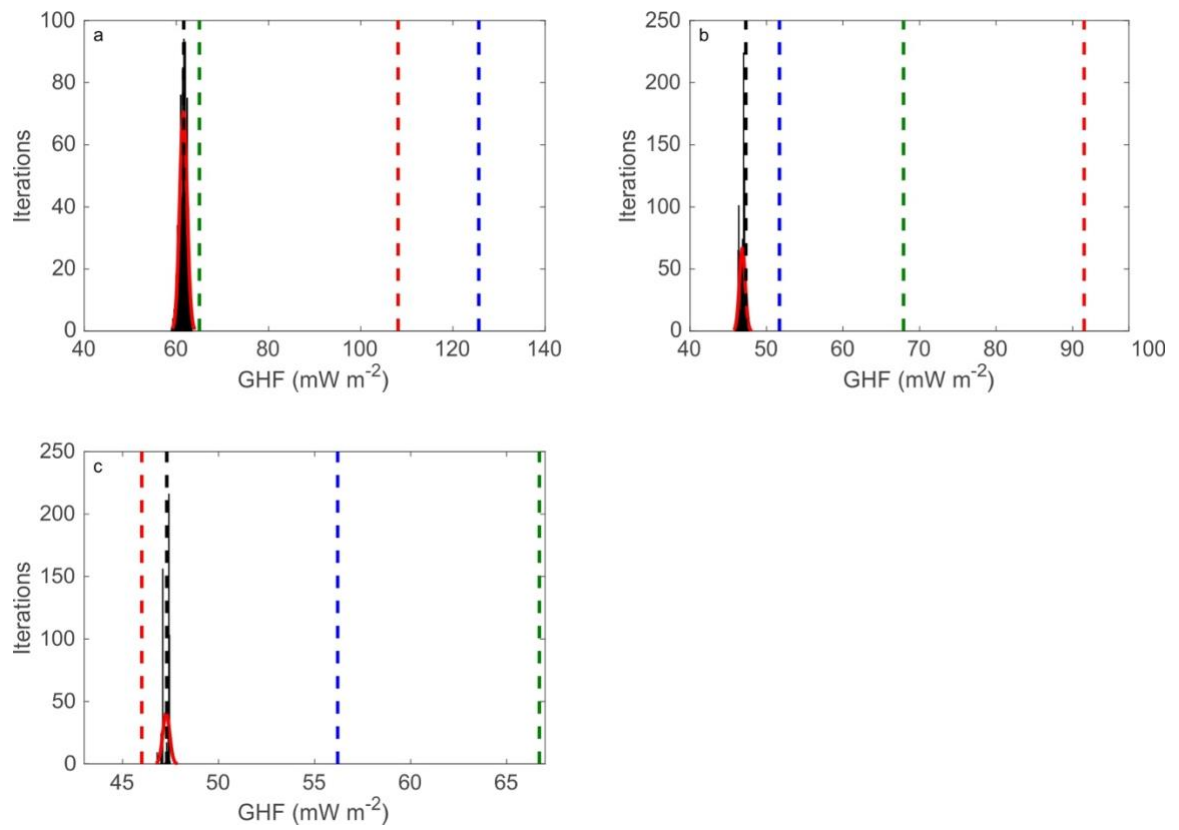
Figure 8.01: Distribution of GHF values with a probability density function fitted (solid red line) for (a) JRI; (b) FP; (c) BI. Dashed lines indicate the modelled GHF estimates: black: the alternative ‘temperature gradient’ method in this study (section 8.2.4); red: Shapiro and Ritzwoller (2004); green: Fox Maule et al. (2005); blue: Purucker (2016).
