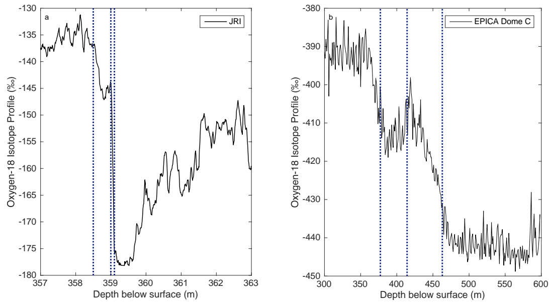
Figure 7.03: (a) The JRI stable water isotope profile at 357 - 363 m (black line) (measured separate to this study); (b) The EPICA Dome C stable water isotope profile at 300 – 600 m (black line) (measured separate to this study). Age constraints at circa 12.8 ka BP, 14.7 ka BP, and 17.5 ka BP are identified by blue dotted lines in each figure.
