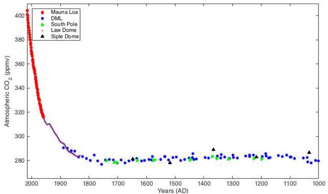
Figure 2.04: 1000-2016 AD record of atmospheric CO 2 concentrations from ice core records and Mauna Loa Observatory. Data has been obtained from www.pangaea.de (Ahn, 2003; Siegenthaler et al., 2005; Etheridge, 2016; Tans, 2016).
