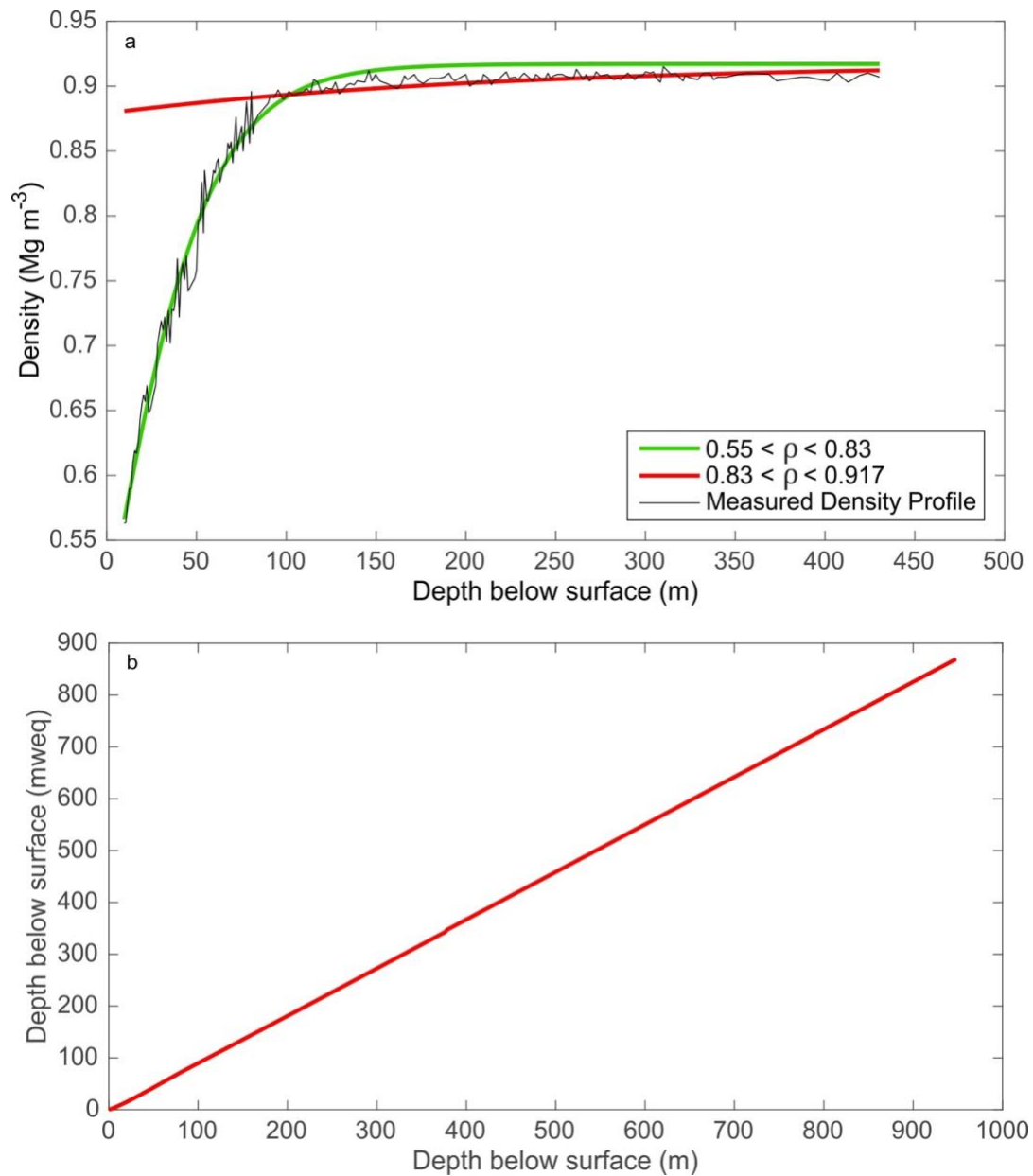
Figure A1.01: (a) Density Reconstruction for the upper 450 m of the BI ice core; (b) Depth below the surface in snow and water-equivalent units. Raw density (black line) measured prior to this research project).
