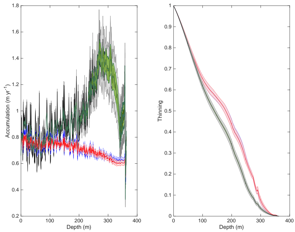
Figure A1.14: Accumulation and thinning reconstructions using the IceChrono model and prescribed accumulation functions at 95% confidence interval for JRI. Different initial accumulation profiles have been used as an input for this figure and are colour-coordinated as black: Clausius-Clapeyron; blue: Simple Exponential; red: Arrhenius; green: IceChrono.
