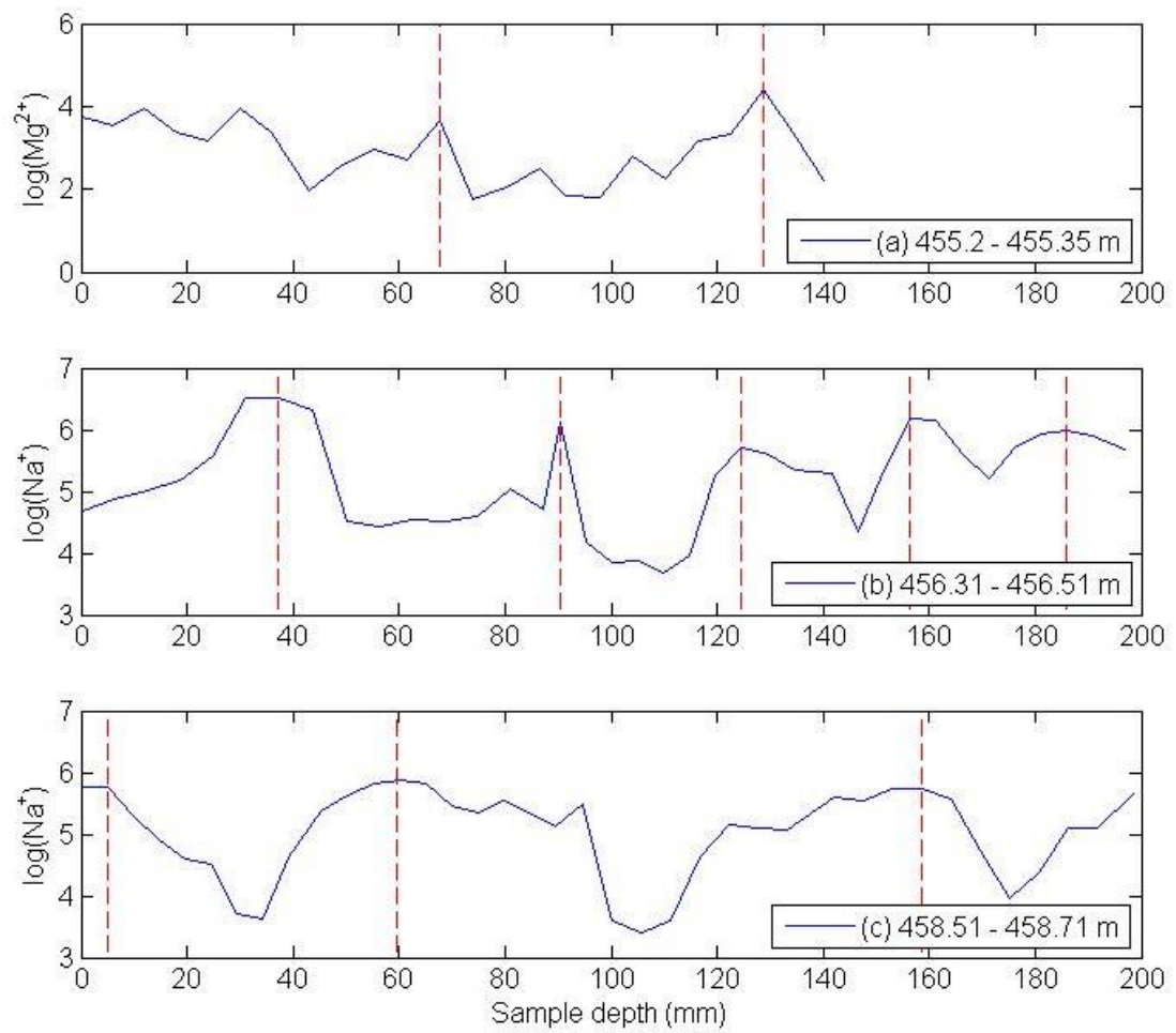
Figure 5.06a – c: Three sections of ice originating from 455 – 459 m analysed by ion chromatography and displayed as semi logarithmic plots of element concentration with red dashed lines indicating annual peaks.
