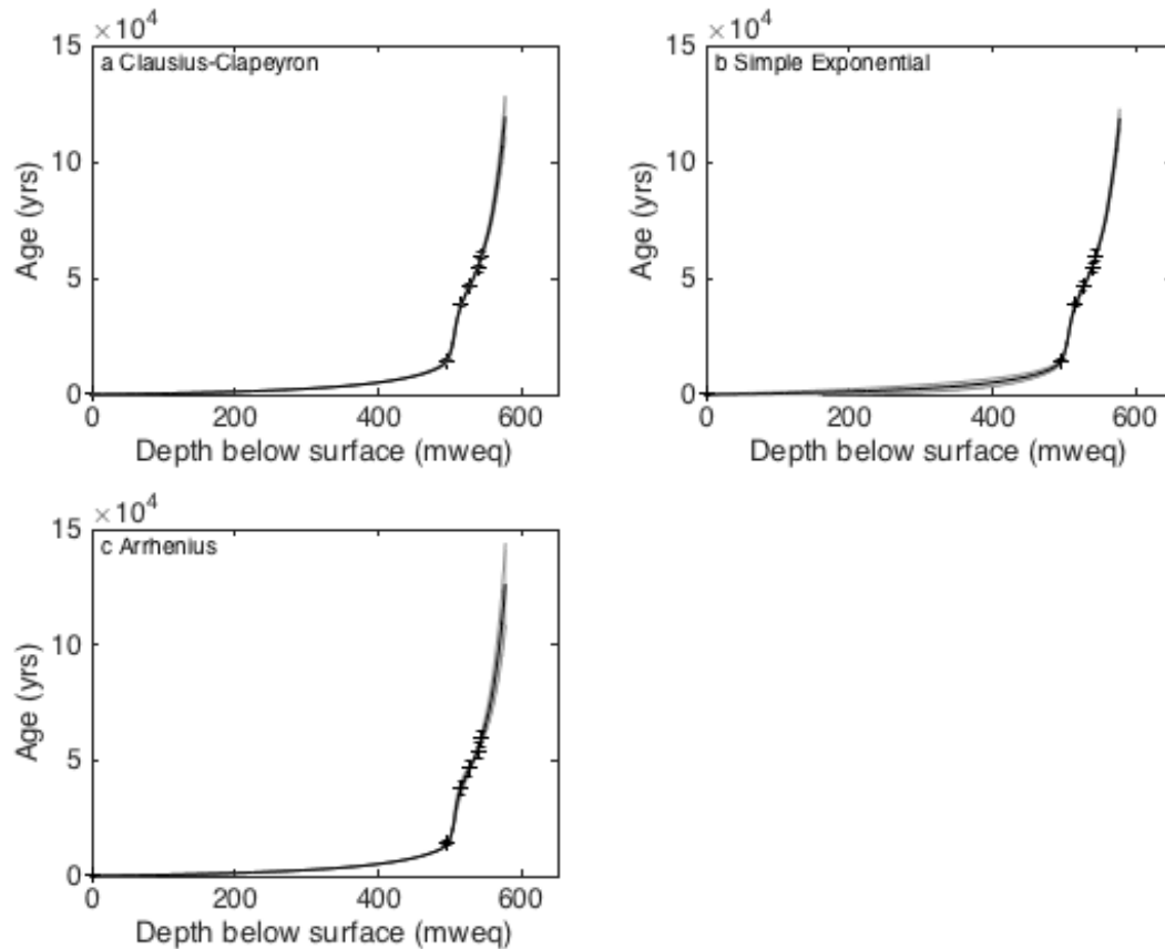
Figure 4.11: Age-depth profiles using the Optimised Accumulation models with uncertainty (grey) and age horizons (black crosses). Clockwise from top left: (a) Clausius-Clapeyron, (b) Simple Exponential, and (c) Arrhenius relationships were used as initial accumulation profiles prior to optimisation.
