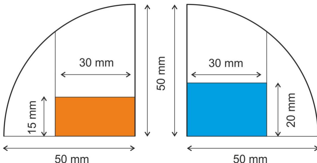
Figure 3.02: Diagram of ice sampling from the archive material; left: the orange shaded section shows sampled ice for LA ICP-MS; right: the blue section shows sampled ice for discrete sampling (see section 3.5).
