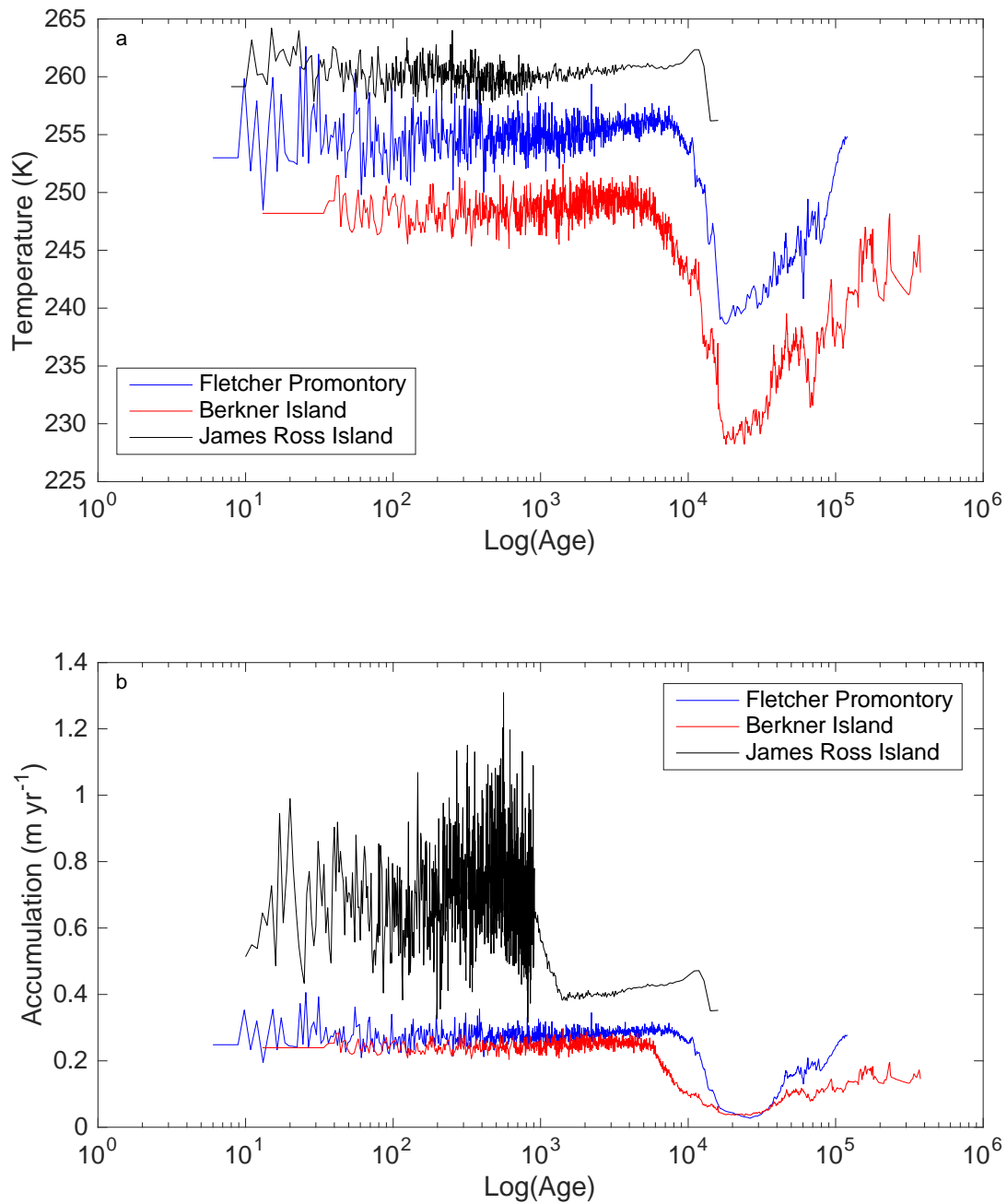
Figure 9.01: (a) Temperature Reconstructions, and (b) Accumulation Reconstructions for James Ross Island (black), Berkner Island (red), and Fletcher Promontory (blue). The JRI profile is capped at the depth of the greatest age constraint used.
