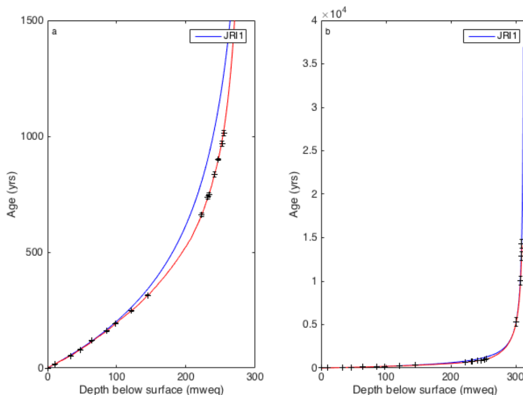
Figure 7.09: (a) Comparison of the JRI1 age-depth profile (blue) with the JRI2 chronology (red) and age horizons (black crosses) for the last 1500 years; (b) Comparison of the initial JRI age-depth profile (blue) with the JRI2 chronology (red) and JRI2 age horizons (black crosses).
