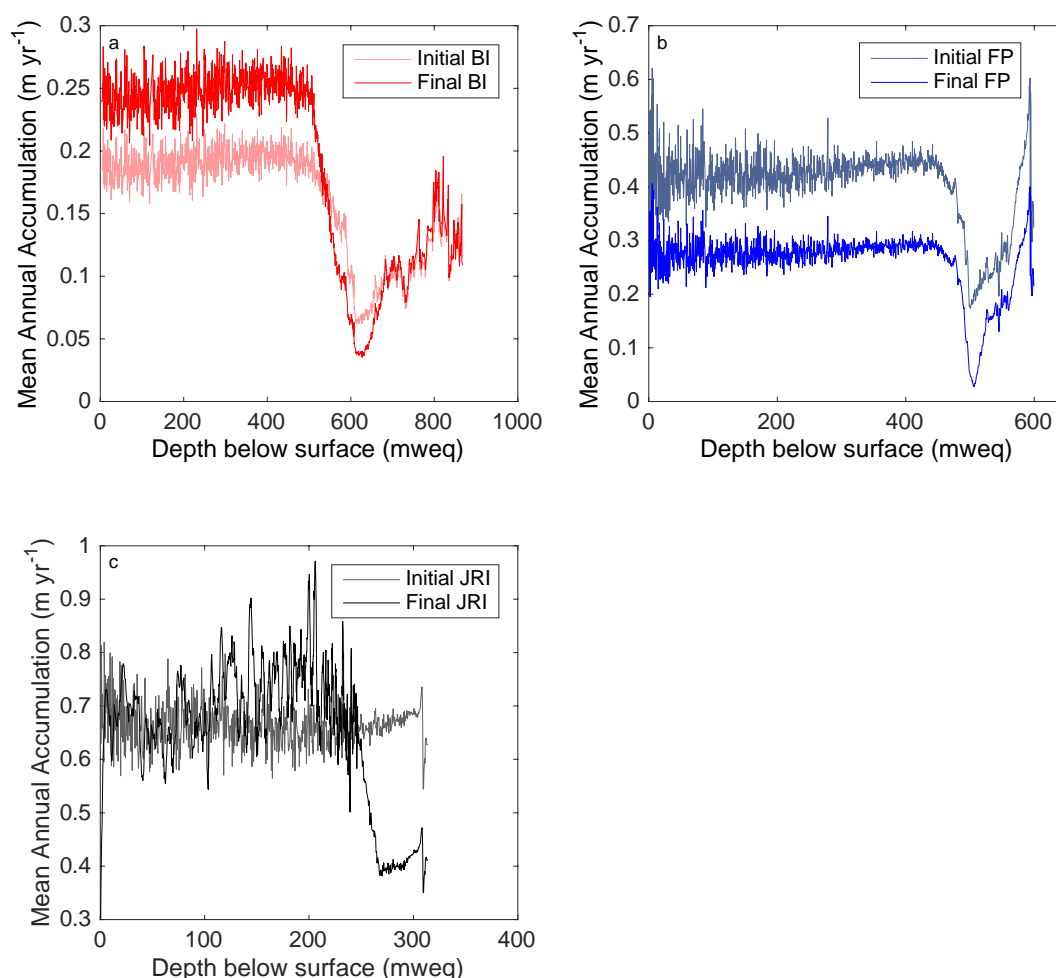
Figure 9.02: Initial and optimised accumulation profiles for the (a) BI; (b) FP; and (c) JRI ice cores. Initial accumulation profiles are estimated using the Clausius-Clapeyron relationship and presented in a pale shade of the colour used to present the optimised reconstruction.
