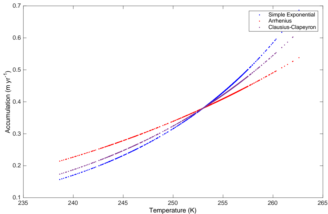
Figure 4.16: Sensitivity change of accumulation reconstructions with respect to temperature.
