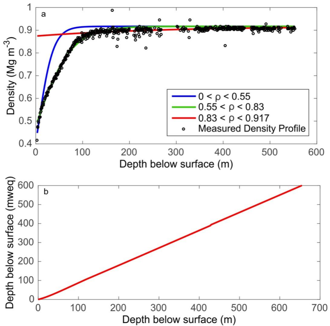
Figure 4.01: (a) Density Reconstruction for the FP ice core plotted against snow depth. The three different colours refer to the three stages of densification; parameters describing these three stages are optimised by least squares approach (section 2.6). The raw density profile is shown as black circles and was measured prior to this research project. Raw density was not measured for the full length of the ice core, and hence the reconstructions only go to the same depth. Density is extrapolated to the bed using the third stage equation fitted to the data; (b) Water-equivalent depth with respect to snow depth.
