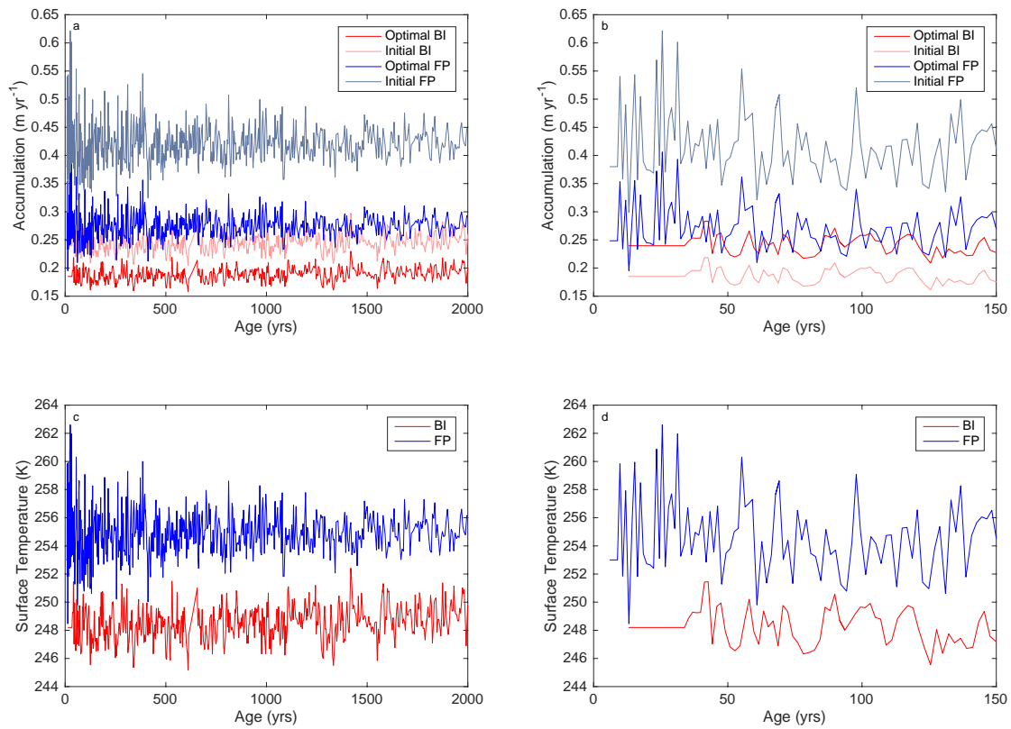
Figure 6.15: Accumulation reconstructions over the last 2000 years; a) accumulation spanning 2000 years; b) accumulation over the last 150 years. Red: BI accumulation with the initial profile in pale red; Blue: FP accumulation profile with the initial profile in pale blue. Underneath, the surface temperature reconstructions of the BI and FP ice cores spanning (c) 2000 years, and (d) the last 150 years.
