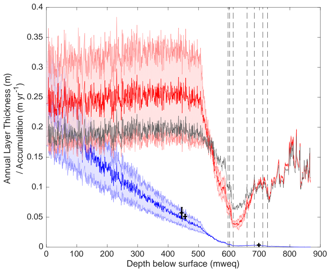
Figure 6.02: Present-day (blue) and original annual layer thickness (red) for the BI ice core. Present-day annual layer thickness is assumed to be the product of the final accumulation and thinning profiles. Black crosses show the observed annual layer thickness measurements. The initial Clausius-Clapeyron accumulation history is presented in grey. The depths corresponding to age horizons are delineated by black dashed lines.
