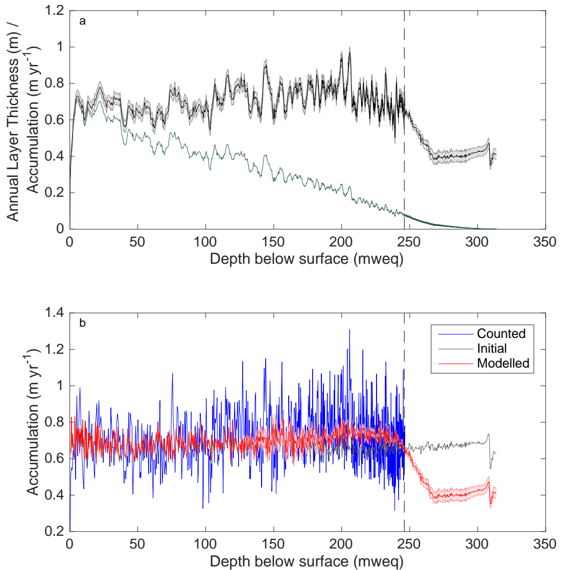
Figure 7.04: The final accumulation and annual layer thickness profiles, and the accumulation reconstructions that contribute to the final accumulation reconstruction. Plot (a) Dark green: present-day annual layer thickness; black: the final accumulation profile. The final accumulation profile is constructed by combining the ten-year mean of the annual layer measurements (left of the grey dashed line), and the OptAcc model reconstruction (right of the grey dashed line). Figure (b) presents the three alternative accumulation profiles. Grey: the initial accumulation profile, reconstructed empirically from the stable water isotope record using the Clausius-Clapeyron relationship; red: the full modelled accumulation reconstruction using the OptAcc model; blue: the annual layer-measured accumulation reconstruction. In each plot, uncertainty on the profiles is presented in the pale shade of the optimised profile. The annual layer measured accumulation reconstruction is estimated by inverting the annual layer thickness measurements (green profile; plot a) using the optimised thinning function.
