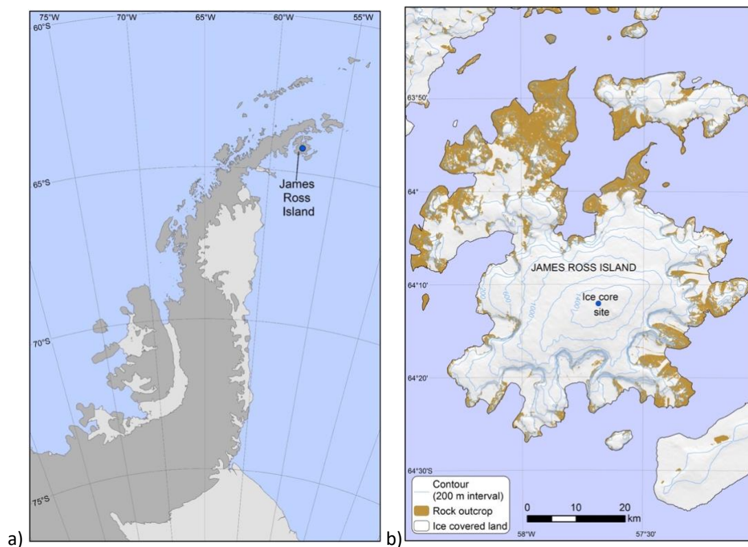
Figure 7.01: (a) JRI in the AP region; (b) a zoom-in to JRI showing the drill site in the context of the Mt. Haddington ice cap that covers the majority of the island.
