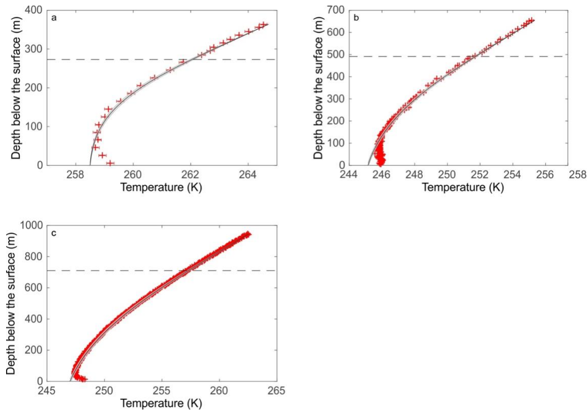
Figures 8.04: Red crosses: Observed temperature measurements with the associated error on depth and temperature measurements (measurements provided by Rob Mulvaney (pers. comm.); black line: modelled temperature profiles with associated uncertainty in grey; (a) James Ross Island; (b) Fletcher Promontory; (c) Berkner Island. A dashed line across each plot represents the depth below which the temperature gradient is used in the alternative GHF calculation (section 8.2.4). All of the ice-core profiles are presented with respect to the depth from the surface (m).
