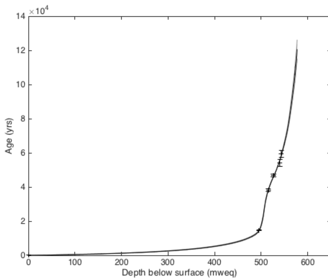
Figure 6.10: Age-depth profile of the FP ice core (black line) with associated error margin (grey). Age constraints are represented by black crosses with the associated age uncertainty.
