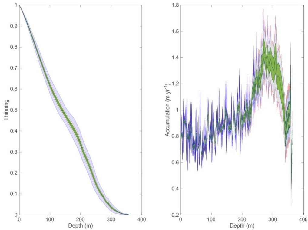
Figure A1.15: Thinning and accumulation reconstructions using the IceChrono model and a prescribed thinning function at 95% confidence interval for the JRI ice core. Different initial initial profiles have been used as an input for this figure and are colour-coordinated as red: Nye; blue: Dansgaard-Johnsen; black: One-Dimensional; green: IceChrono.
