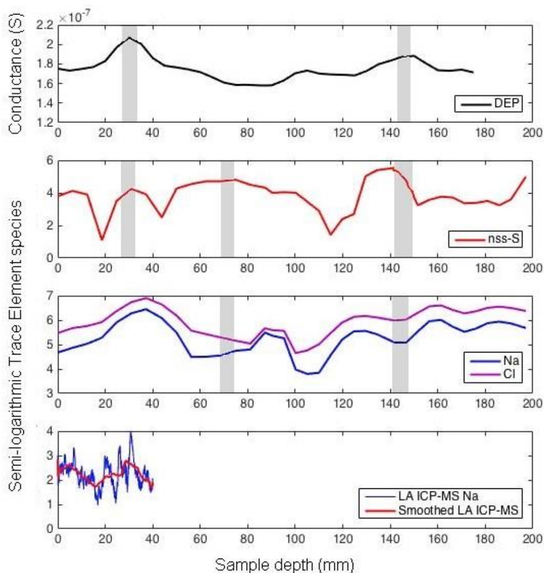
Figure 5.07: Comparison of parallel sections of ice from 456.31 m – 456.51 m from top to bottom: the DEP data; nss-S profile analysed by discrete sampling; sodium and chloride profiles analysed by discrete sampling; ice analysed by LA ICP-MS with the profile smoothed to the same resolution used in the discrete sampling technique, with annual layers indicated by grey lines.
