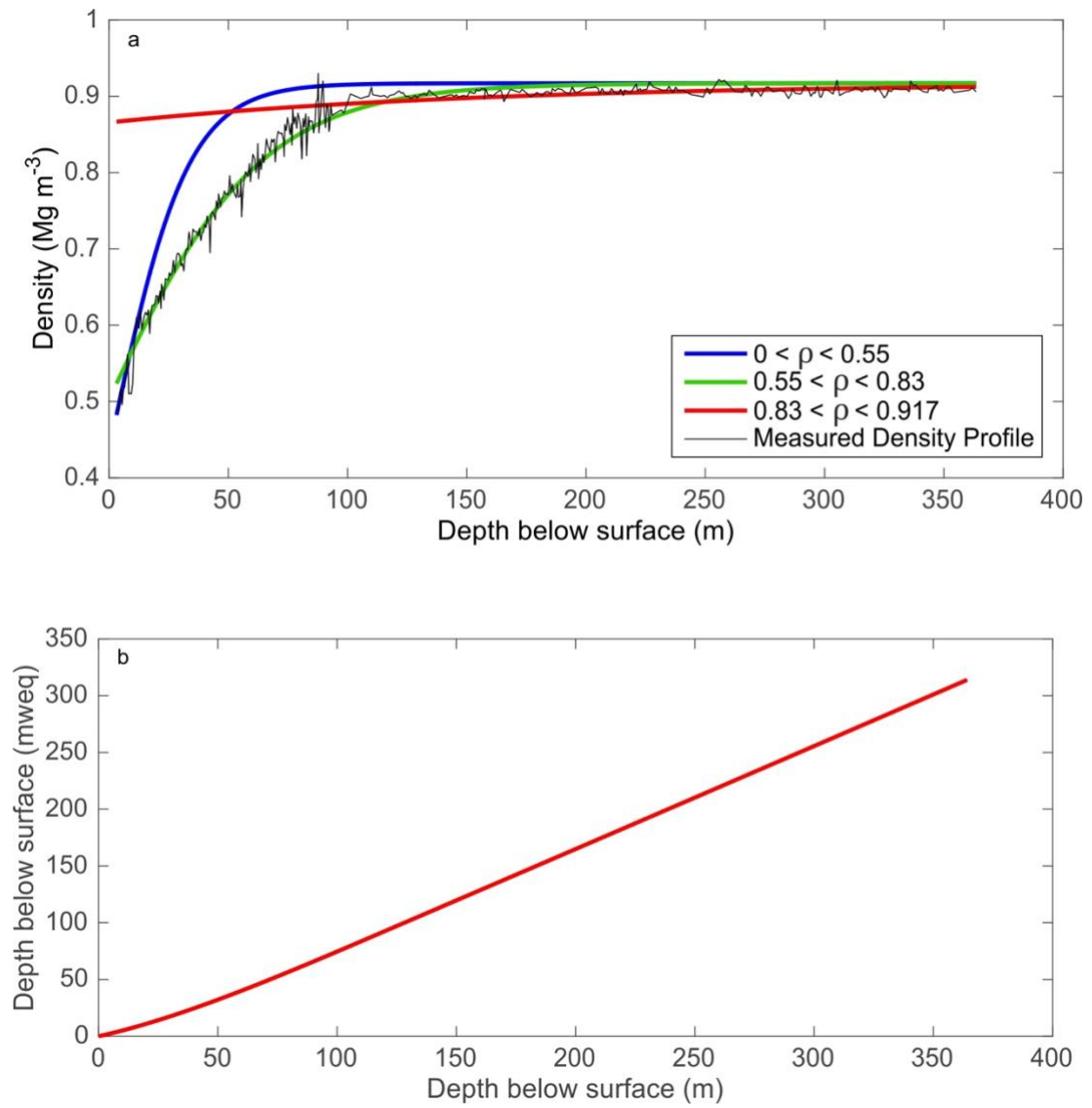
Figure A1.02: (a) Density Reconstruction for the JRI ice core; (b) Depth below the surface in snow and water-equivalent units. Raw density (black line) measured prior to this research project).
