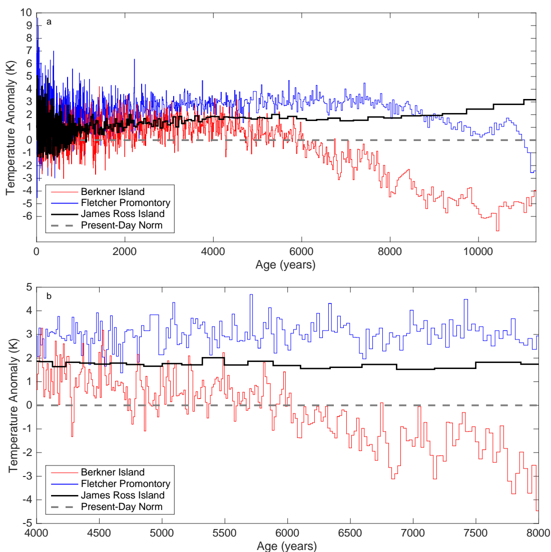
Figure 9.03: (a) Reconstructed surface temperature anomaly covering the Holocene (11.3 - 0 ka BP) for JRI (black), FP (blue), and BI (red). The grey dashed line is a normalised present-day surface temperature; (b) a zoom-in of plot (a) on the period 8-4 ka BP when marine and geomorphological records indicate the AP had more open ocean.
