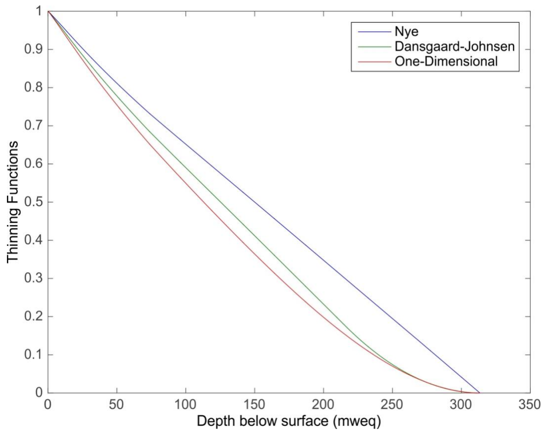
Figure A1.08: Thinning Functions for the JRI ice core.
