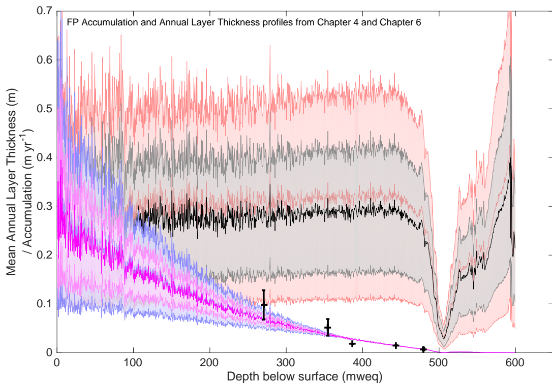
Figure 6.12: The optimised accumulation and present-day annual layer thickness profiles of FP, estimated using the OptAcc model. The 10-point averaged accumulation profiles and associated uncertainty for the model scenarios that are constrained by either only age horizons (red), or constrained by age horizons and measured annual layer thickness (black). Also shown are the 10-point averaged layer thickness profiles and associated uncertainty for the model scenarios that are constrained by only age horizons (blue), or constrained by age horizons and measured annual layer thickness (purple). Annual layer thickness constraints are also shown as black crosses on the figure.
