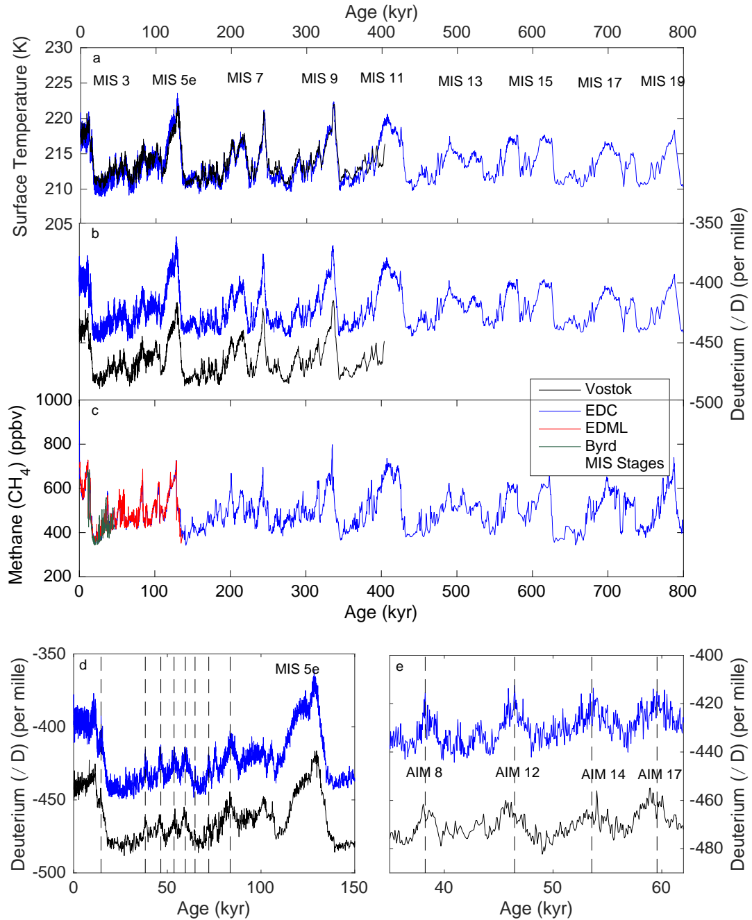
Figure 2.05: (a) Surface temperature reconstructions for the EDC and Vostok ice cores on a common timescale; (b) Stable water isotope profile for EDC and Vostok ice cores on a common timescale; (c) Methane profiles for the EDC, EDML, and Byrd ice cores on a common timescale. Odd-numbered Marine Isotope Stages (interglacials) are highlighted in grey and labelled in plot (a). Panels (d) and (e) are zoom-in plots of the stable water isotope profiles of EDC and Vostok (the pink highlighted section of plot (b), and the grey highlighted panel in plot (d), respectively). MIS 5e is highlighted as a grey band and labelled. Antarctic Isotope Maxima events are delineated by black dashed lines and labelled in plot (e).
