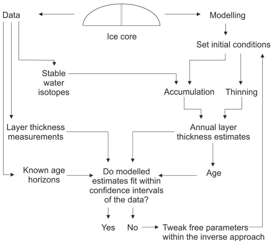
Figure 2.08: A flow chart outlining the construction of an age-depth profile and where each reconstruction or chemical measurement is incorporated.
