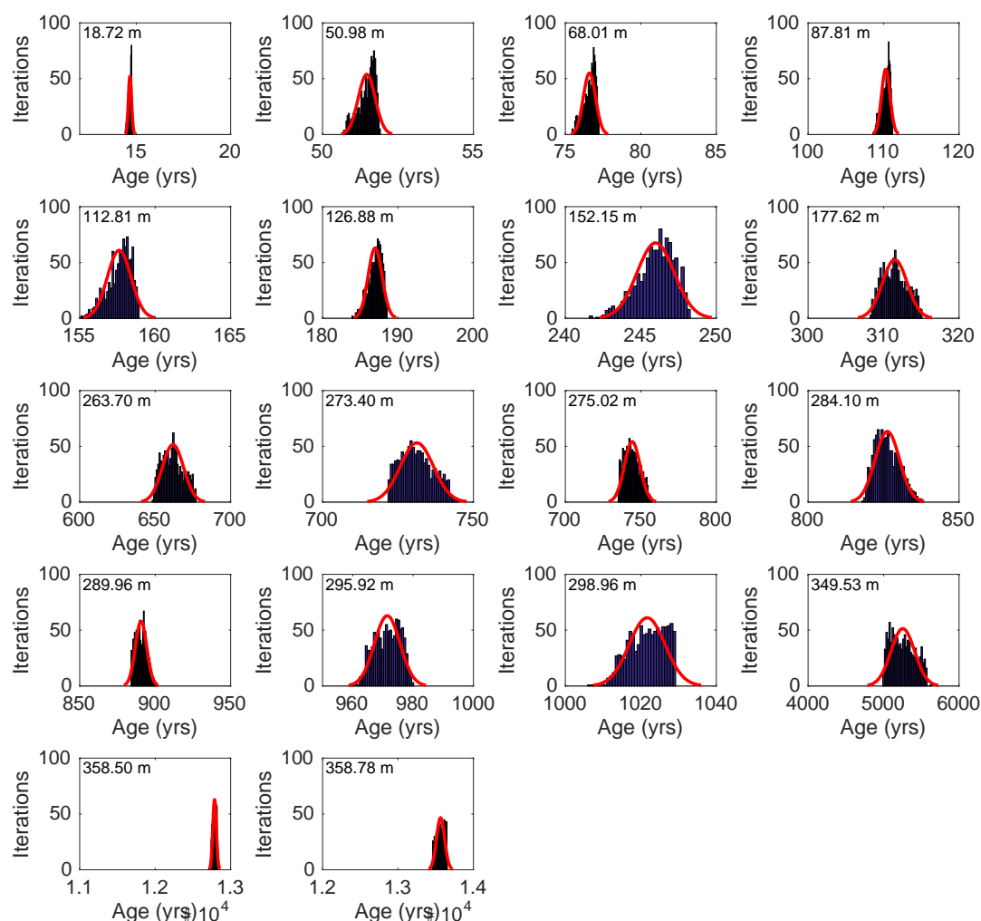
Figure 7.08: Histogram distributions of modelled age estimates at depths corresponding to age horizons with a normal distribution function fitted. A grey box corresponds to the age horizon and uncertainty. The depth in snow-equivalent metres is in the top-left corner.
