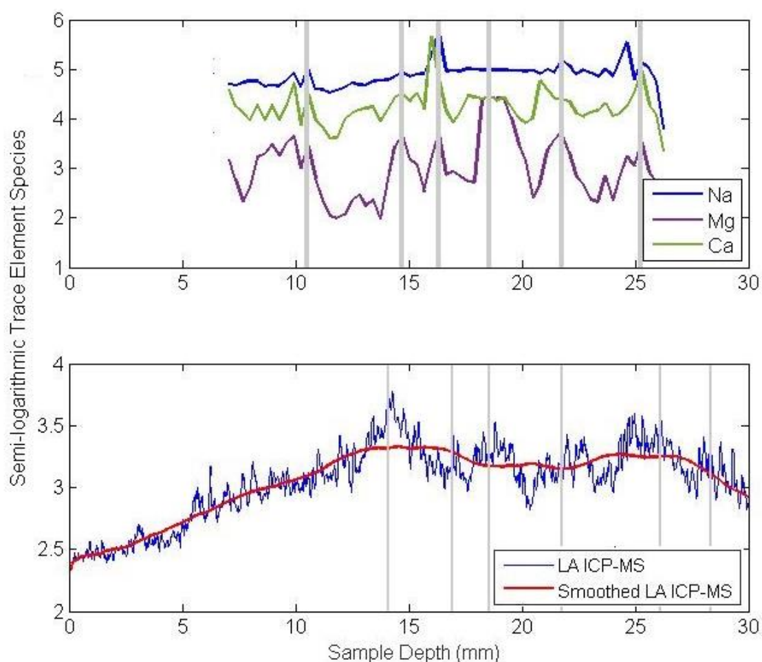
Figure 5.09: Comparison of parallel sections of ice from 703.2 - 703.22 m from top to bottom: ice analysed by discrete sampling technique; ice analysed via LA ICP-MS with a smoothed profile (red).
