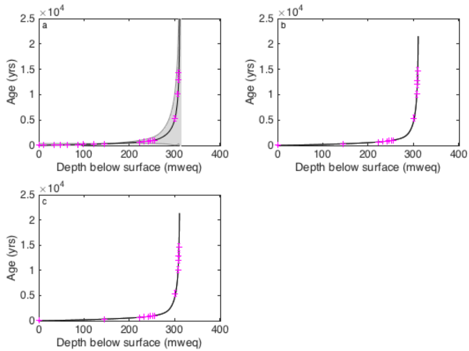
Figure A1.25: Age-depth reconstructions using different initial accumulation profiles and optimised using the Optimised Accumulation and Thinning model for JRI, with known-age horizons in pink crosses. Initial accumulation history from top left: (a) Clausius-Clapeyron; (b) Simple Exponential; (c) Arrhenius relationships.
