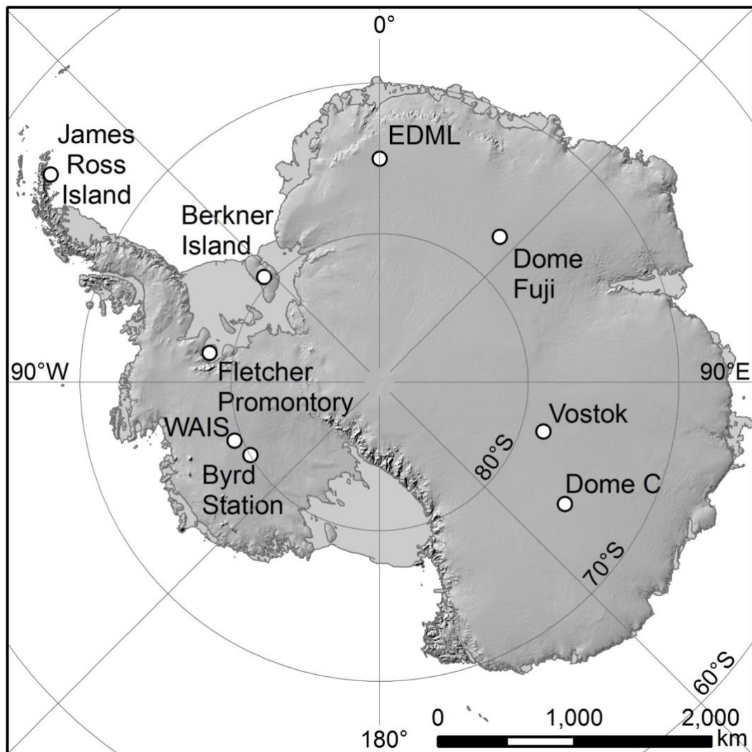
Figure 2.02: Map of ice core sites across Antarctica mentioned in the text.
