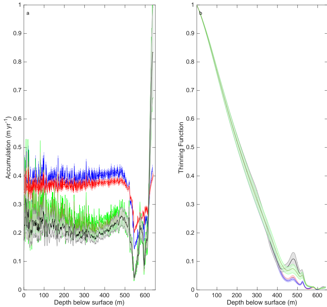
Figure 4.07: (a) Four accumulation reconstructions that have been optimised using the IceChrono toolbox, and (b) the associated thinning profiles for each model scenario. In these model scenarios, boundary accumulation profiles were fixed with 95% confidence to assess how this constraint would affect the thinning profile. Optimised profiles are colour-coded for each model scenario. Black: freely-calculated; green: Clausius-Clapeyron; blue: Simple Exponential; red: Arrhenius, with the associated uncertainty for each profile marked by a lighter shade of the main profile colour. The freely-calculated and Clausius-Clapeyron reconstructions are so similar that the freely-calculated reconstructions are presented as a 5-point moving average in order to smooth the profile and ensure that all profiles are visible.
