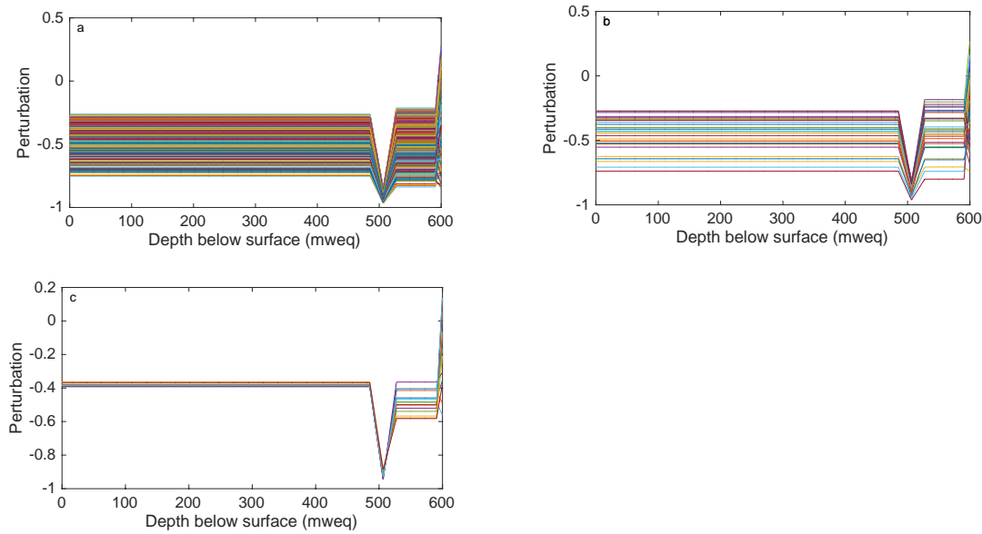
Figure 4.13: Perturbation profiles for each possible optimal profile (1000 profiles) for the FP ice core using an initial accumulation profile derived from the (a) Clausius-Clapeyron relationship; (b) Simple Exponential relationship; (c) Arrhenius relationship.
