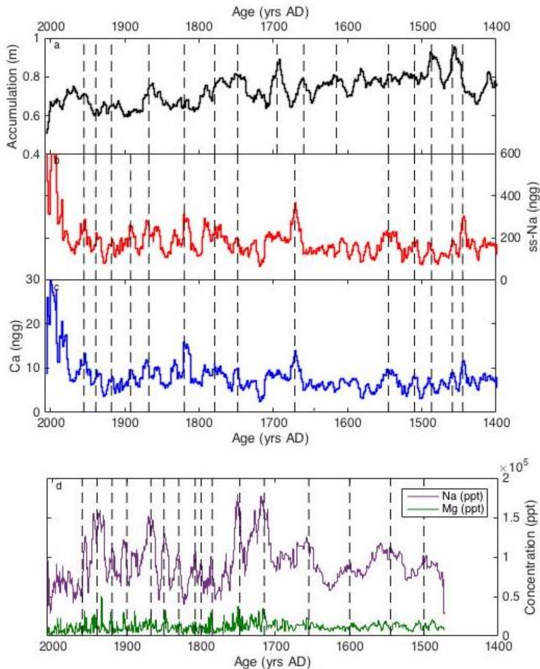
Figure 7.12: LIA signatures in the JRI ice core from 1400 AD – 2000 AD. From top to bottom, a: accumulation ( \text{m yr}^{-1} ); b: sea-salt Sodium (ngg); c: Calcium (ngg). All profiles were measured separate to this research project at DRI. Profiles are presented on a decadal-mean to show trends. Plot d: Mt Erebus ice core data presented as a smoothed decadal mean record in parts per trillion (ppt) (data available courtesy of Rhodes et al. from https://www.ncdc.noaa.gov/paleo-search/study/13175 ). Purple: Sodium; green: Magnesium. Dashed lines indicate decadal to centennial variability in the records.
