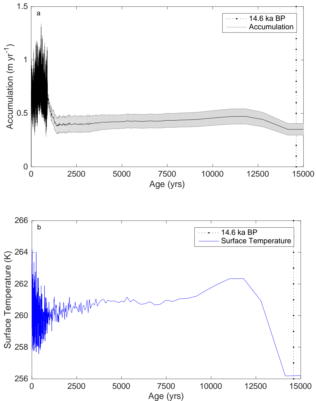
Figure 7.10: (a) Full-resolution accumulation reconstruction from 15-0 ka BP with the uncertainty (grey), and the 14.6 ka BP constraint presented as a dotted line; (b) Mean annual surface temperature spanning 15 - 0 ka BP, with the 14.6 ka BP constraint presented as a dotted line.
