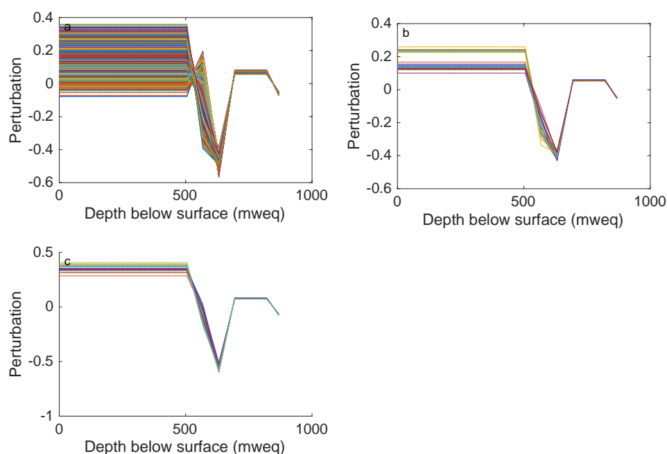
Figure A1.23: Perturbation profiles for 100 possible scenarios for the BI ice core using the Optimised Accumulation and Thinning model. Model scenarios use an initial accumulation profile using (a) Clausius-Clapeyron; (b) Simple Exponential; (c) Arrhenius relationships.
