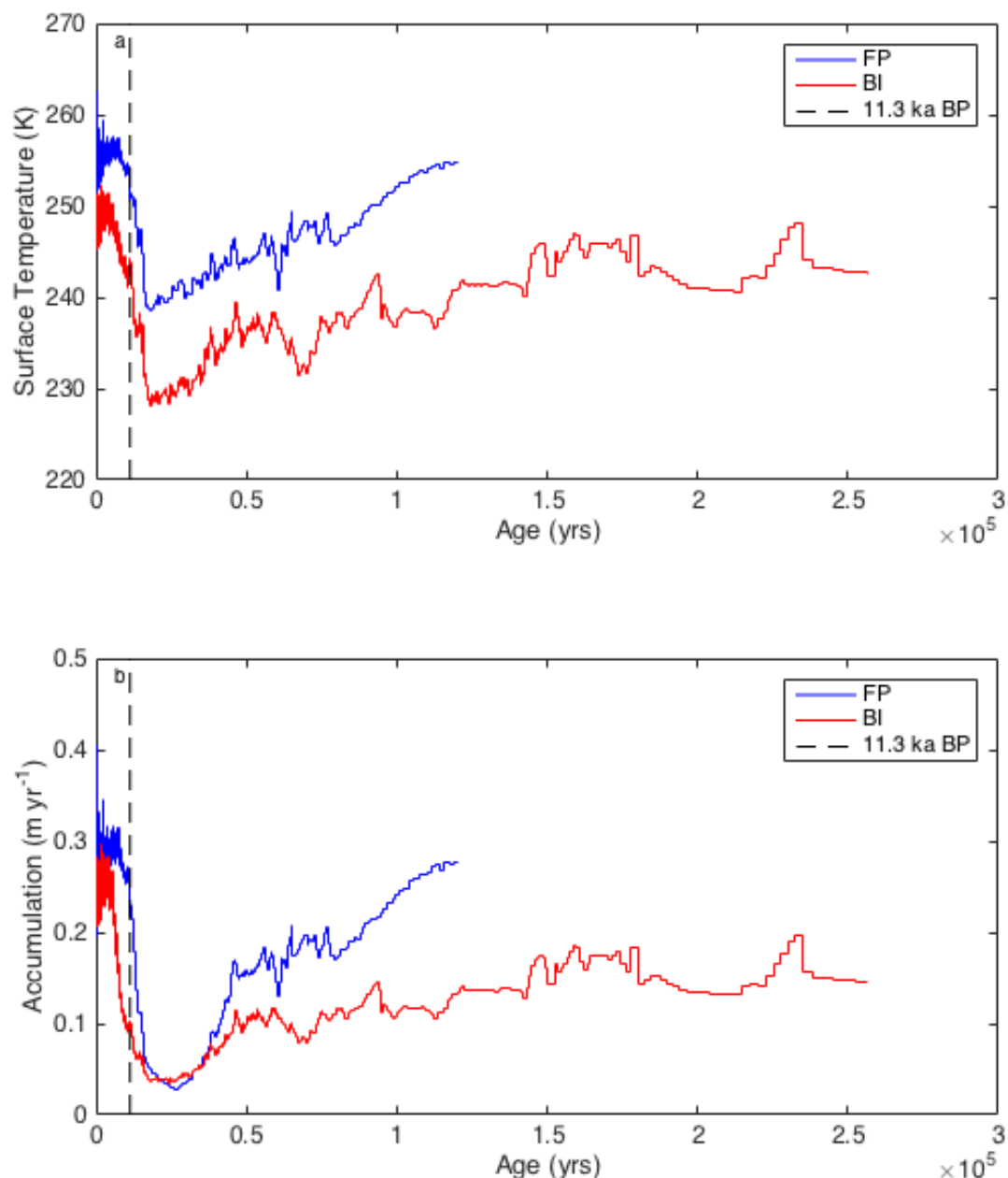
Figure 6.13: (a) Temperature reconstructions, and (b) Accumulation reconstructions for FP and BI ice cores. Blue: FP records; Red: BI ice core reconstruction. The 11.3 ka BP initiation of the Holocene period is marked by the grey dashed line.
