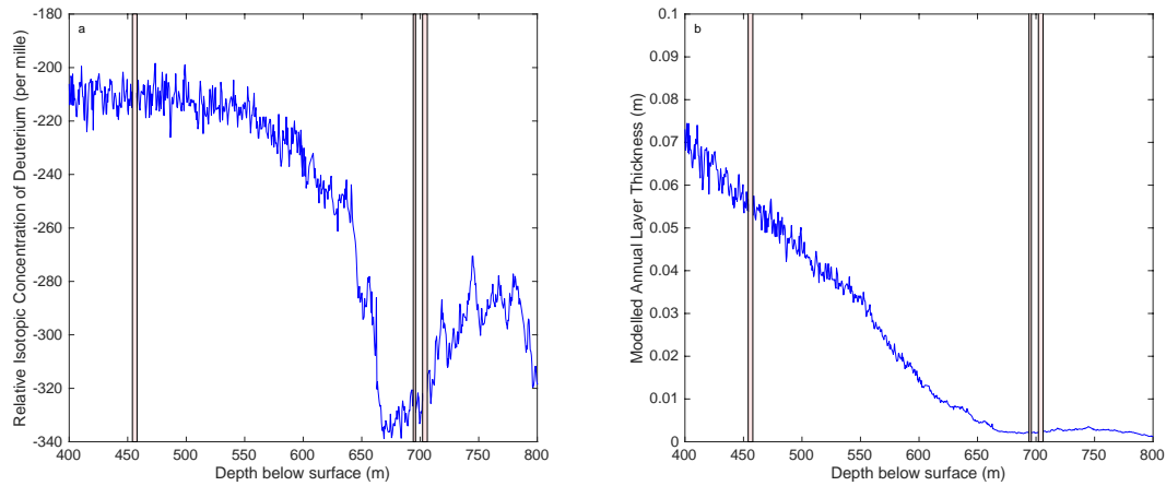
Figure 5.01: Berkner Island ice core sampled sections of ice (pink bands) across the (a) isotopic and (b) modelled annual layer thickness profiles. See supplementary information for model description.
