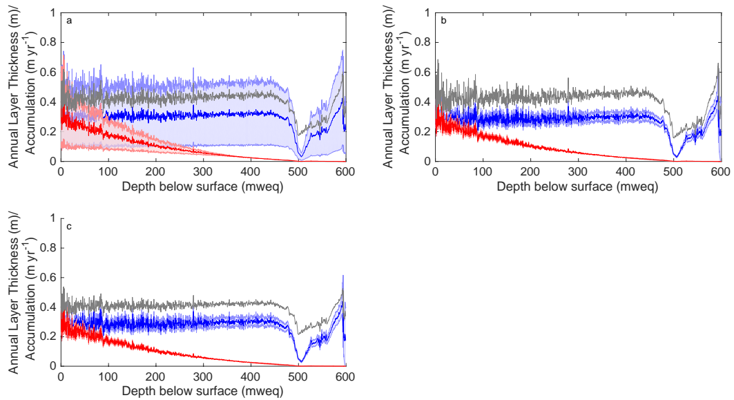
Figure 4.12: Annual layer thickness profiles and accumulation estimated for FP ice core. A priori accumulation profiles: (a) Clausius-Clapeyron; (b) Simple Exponential; (c) Arrhenius. Dark blue: optimal accumulation profile modelled using the optimisation model; pale blue: uncertainty on the optimal accumulation profile; grey: the a priori accumulation profile (one of three empirical reconstructions); red: optimal annual layer thickness profile; pale red: uncertainty on annual layer thickness profile.
