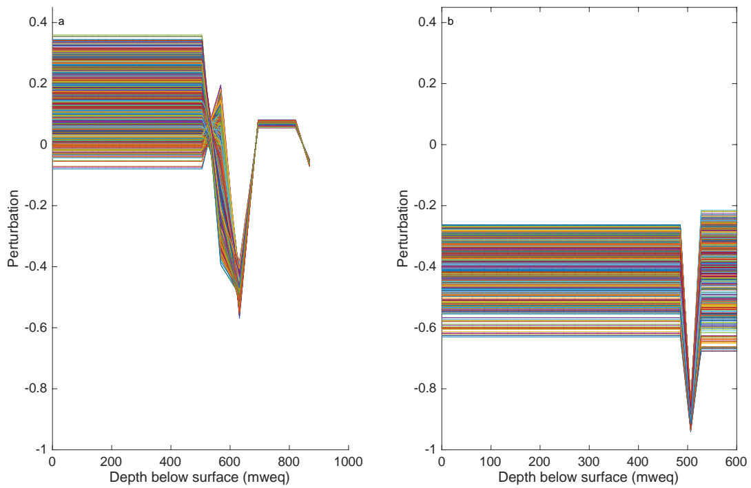
Figure 6.03: Perturbation profiles for each ice core reconstruction: (a) 1000 perturbation profiles for BI; (b) 1000 perturbation profiles for FP. Each coloured line is an individual perturbation profile.
