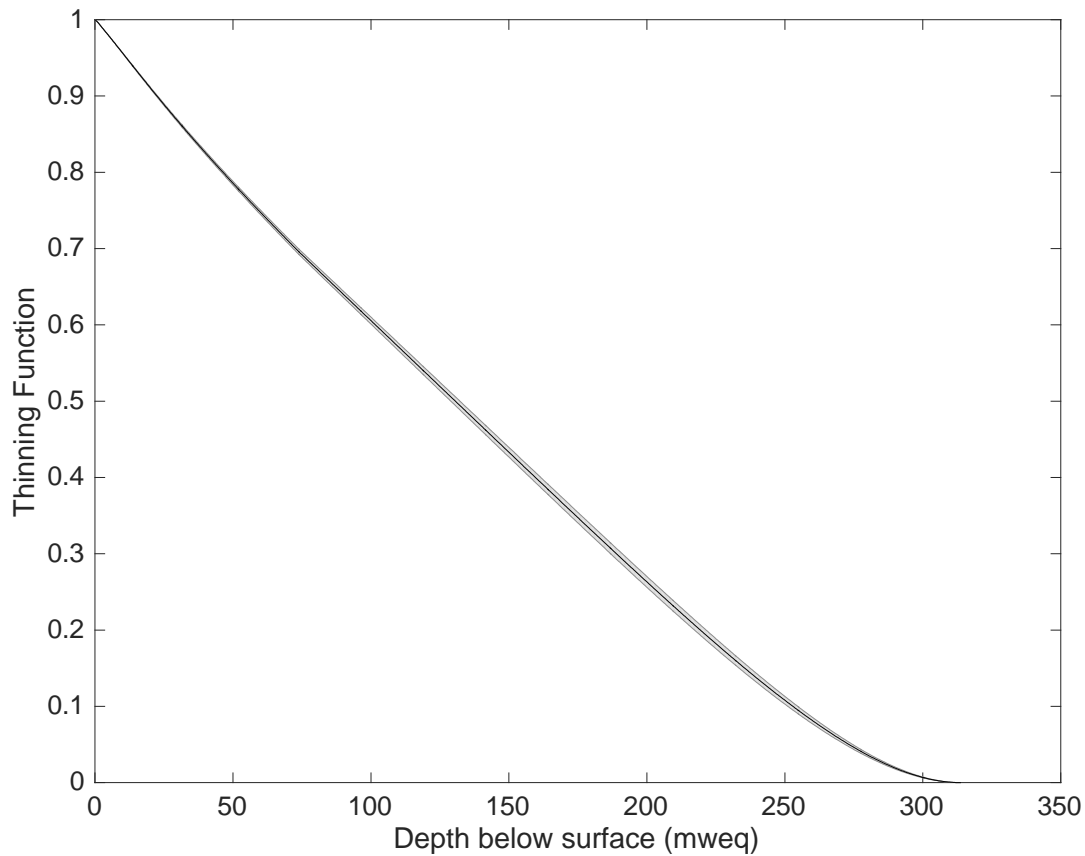
Figure 7.06: Thinning function for the JRI ice core with associated uncertainty in grey.
