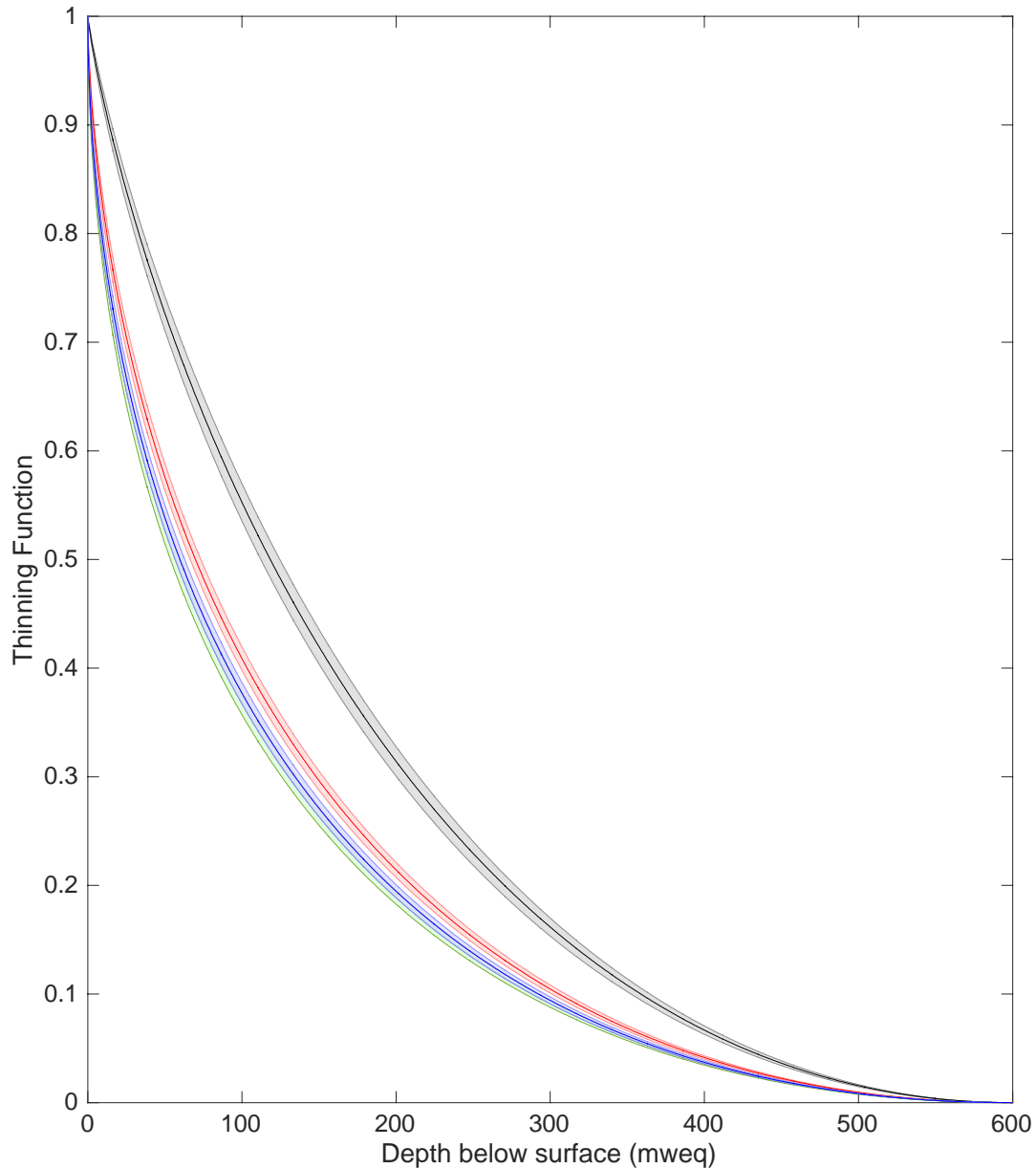
Figure 4.10: Posterior thinning functions and associated uncertainty constrained using the Direct Search method: four model scenarios using prescribed empirical accumulation. Green: Clausius-Clapeyron; Red: Simple Exponential; Blue: Arrhenius; Black: IceChrono.
