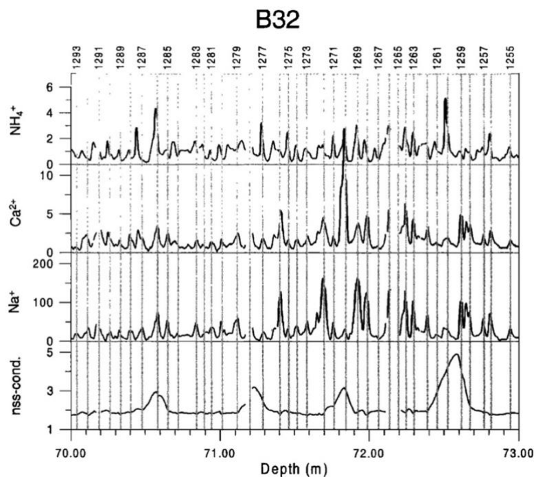
Figure 2.03(b): Example of annual layer counting using three aerosol components in parts per billion (ppb) (Sodium, Calcium, and Ammonium), and non-sea-salt conductivity measurement in the B32 ice core, Antarctica, across a 3 m section covering 1255 - 1293 AD (Sommer et al., 2000).
