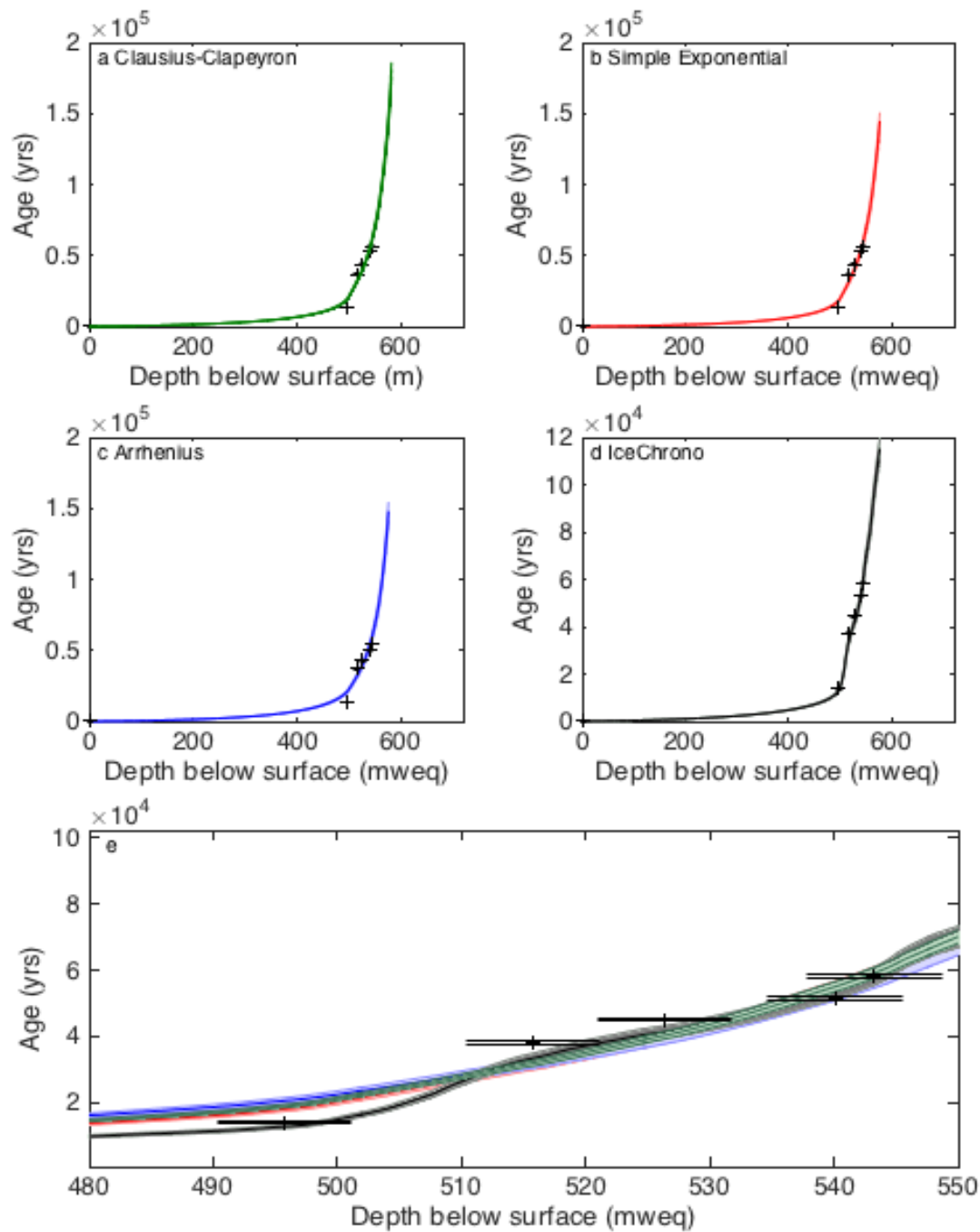
Figure 4.09: Age-depth profiles using the Direct Search approach as calculated using four different accumulation history profiles. Plot a-d: individual age-depth estimates (coloured line) and age horizons (black crosses; height of cross indicates age uncertainty but the differences are not visible); plot e: four age-depth estimates zoomed into the depth range 480–550 mweq to focus on fit with age horizons (black crosses). Each model scenario uses a different profile of accumulation and can be identified as: (a) Clausius-Clapeyron (green); (b) Simple Exponential (red); (c) Arrhenius (blue); (d) IceChrono (black). The zoom-in on plot (e) shows the four age-depth profiles; the Simple Exponential profile (red) is not easily visible in the figure due to its similarity with Clausius-Clapeyron profile (green).
