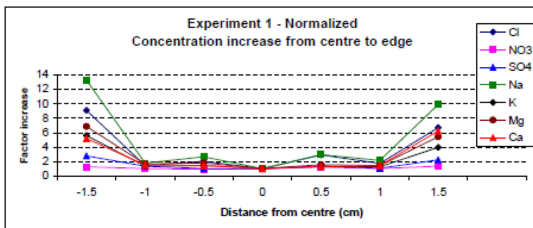
Figure 3.06: Factor increase of ion concentrations emanating from the centre of a section of the GRIP ice core. Results show concentrations decrease from the outside towards the centre of the core, suggesting that the outer 1 cm of ice contains contaminants from the drilling process. Figure taken from Thomas (2006).
