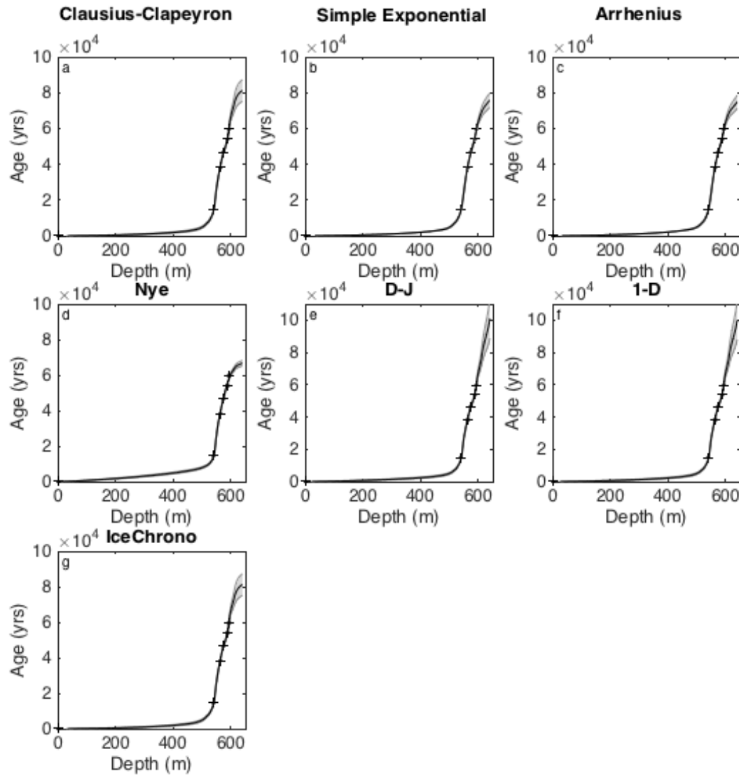
Figure 4.06: Age-depth profiles constructed using the IceChrono model. Top row (a-c): age-depth profiles with prior information on the accumulation profile; middle row (d-f): age-depth profiles with prior information on the thinning profile; bottom left (g): no prior information on either reconstruction. Uncertainty (grey) and age horizons with their associated uncertainty (black crosses) are included with each figure.
