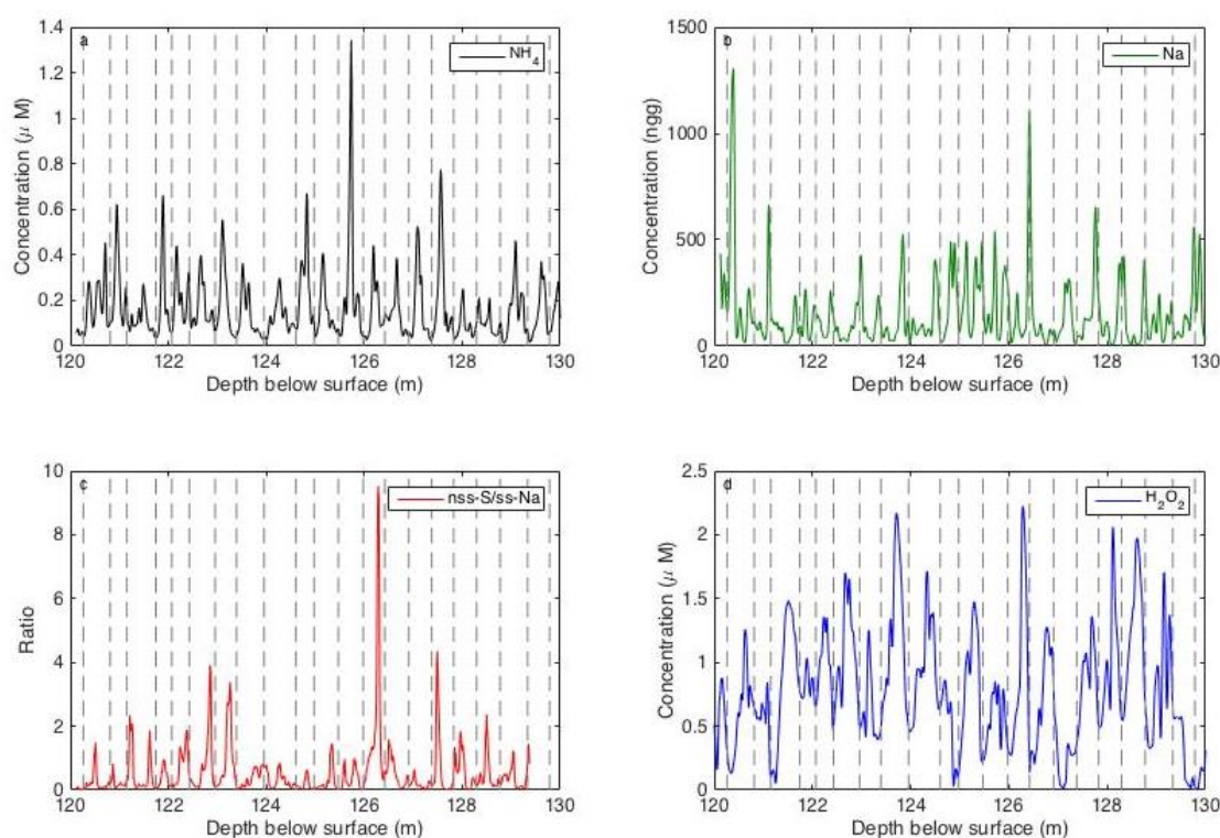
Figure 7.02: Seasonal cycles across a 10 m section of the JRI ice core (120 – 130 m) analysed by colleagues at DRI; a) Ammonium b) Sodium; c) the ratio of non-sea salt Sulphur and sea-salt Sodium; d) Hydrogen Peroxide. Grey dashed lines indicate annual layers identified using the Matchmaker tool.
