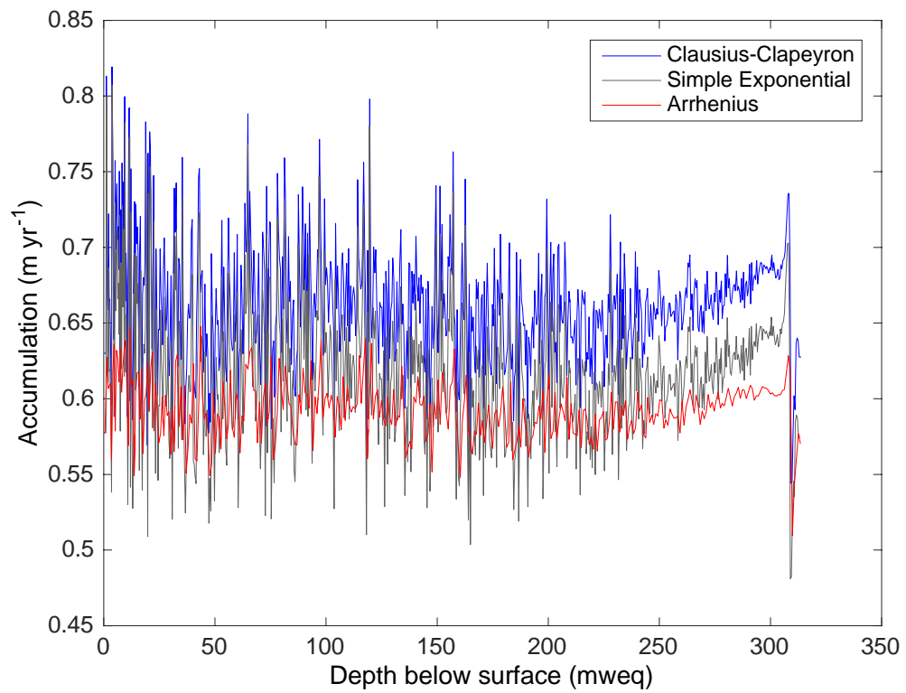
Figure A1.06: Accumulation reconstructions for the JRI ice core. Accumulation reconstructions use stable water isotope profiles obtained separate to this research project.
