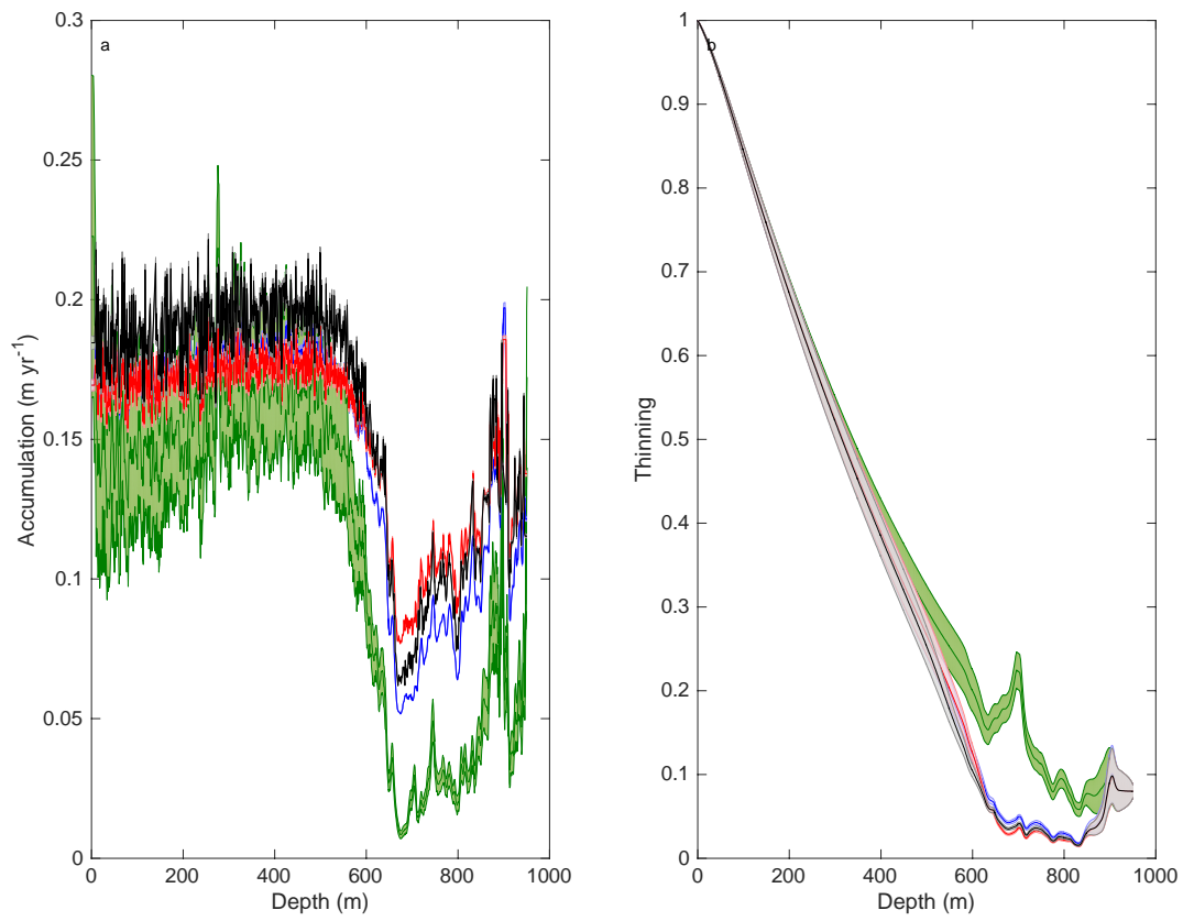
Figure A1.11: Accumulation and thinning reconstructions using the IceChrono model and prescribed accumulation functions at 95% confidence interval for BI. Different initial accumulation profiles have been used as an input for this figure and are colour-coordinated as black: Clausius-Clapeyron; blue: Simple Exponential; red: Arrhenius; green: IceChrono .
