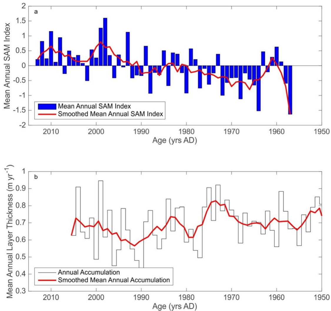
Figure 7.14: (a) the Mean Annual SAM index for the period 1957 – 2012, for comparison with (b) annual accumulation at JRI between 1955 and 2005. Comparison of the annual records in plot (a) and plot (b) give an r^2 coefficient of 0.3, suggesting there is additional forcing on the high variability in annual accumulation at JRI.
