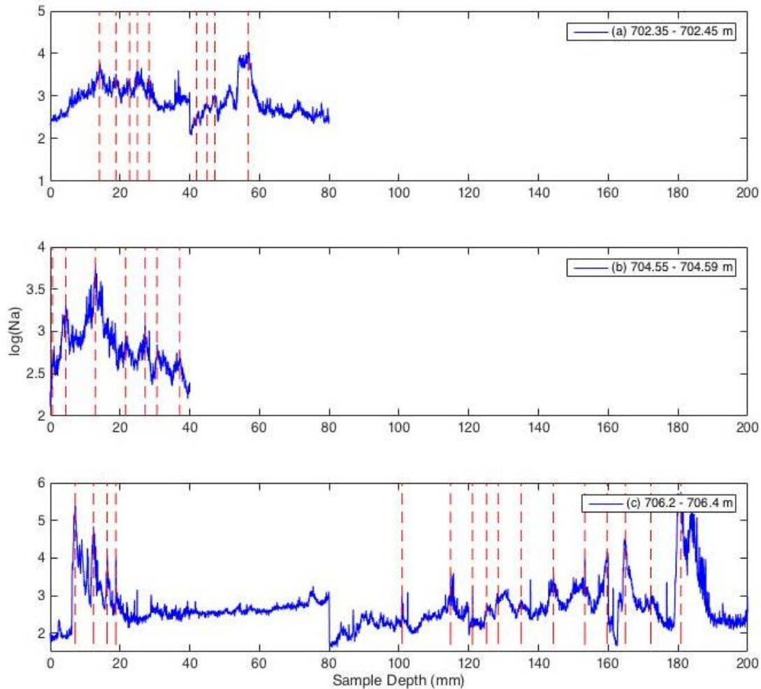
Figure 5.05a – c: LA ICP-MS profiles for three sections of ice from 702 – 707 m; semi logarithmic plots show the \log(\text{Na}) on a common depth scale with red dashed lines delineating a seasonal peak.
