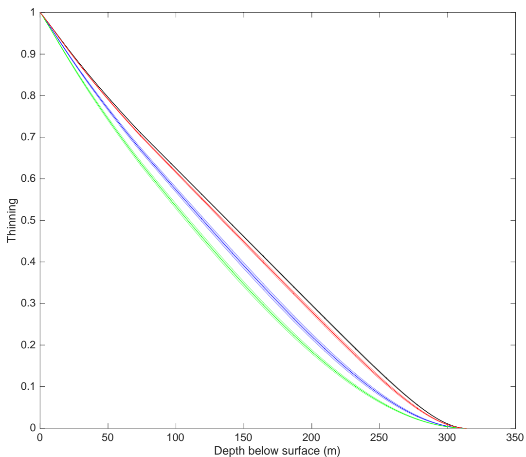
Figure A1.19: Reconstructed thinning functions for the JRI ice core using the Direct Search model. Each scenario uses a different initial accumulation profile: red: Clausius-Clapeyron; blue: Simple Exponential; green: Arrhenius; black: IceChrono. Each scenario has an associated uncertainty presented in a pale shade of the presented colour.
