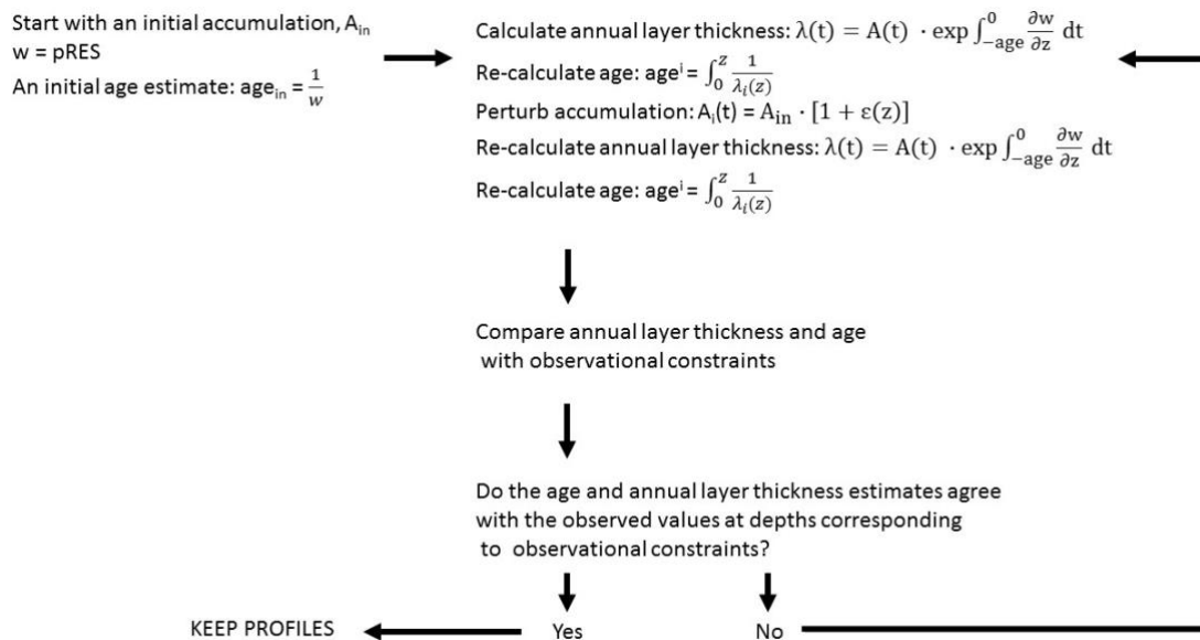
Figure 3.07: A flow diagram outlining an approach to reconstruct the accumulation, annual layer thickness, and age-depth profile using pRES measurements.
