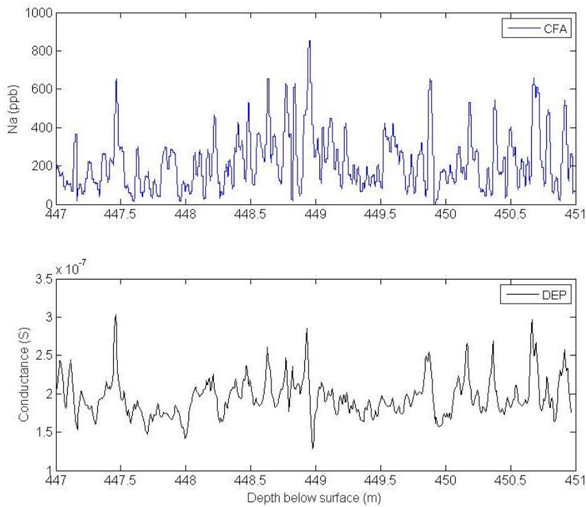
Figure 5.02: Four-metre section analysed by CFA and DEP. Top: CFA Na; bottom: DEP.
