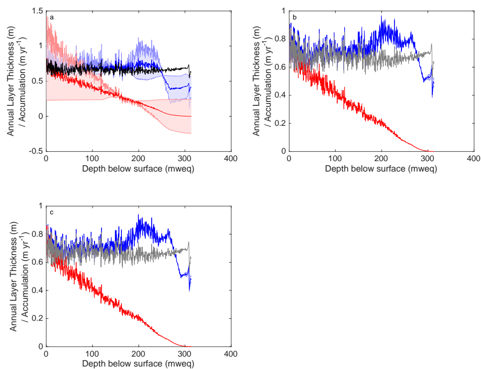
Figure A1.24: Original (red with the confidence interval in pale red) and present-day annual layer thickness (blue with the confidence interval in pale blue) reconstructions using different initial accumulation profiles and perturbed using the Optimised Accumulation and Thinning model for JRI. Initial accumulation history (grey) from top left: (a) Clausius-Clapeyron, (b) Simple Exponential, and (c) Arrhenius.
