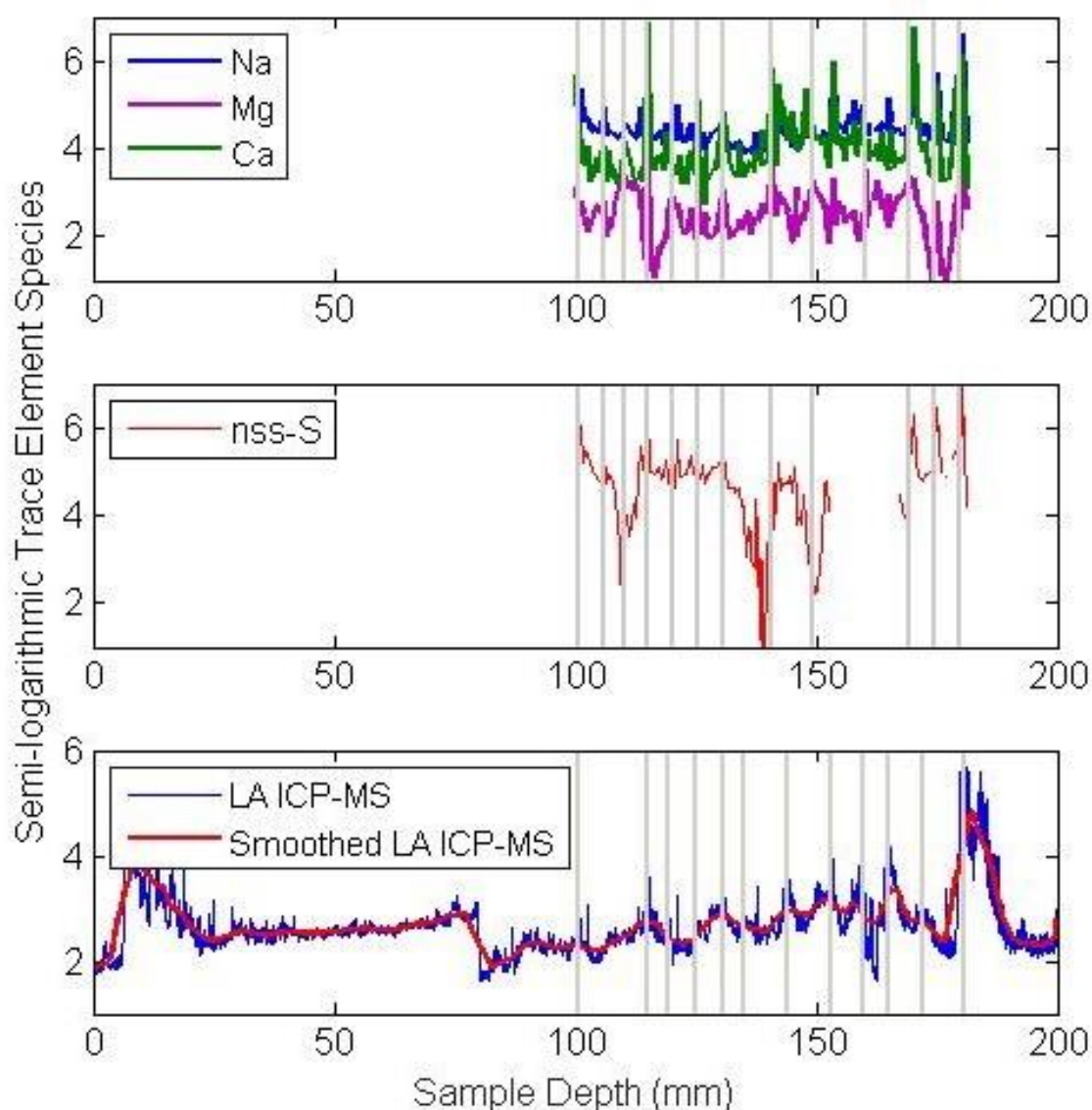
Figure 5.10: Comparison of parallel sections of ice from 706.3 - 706.38 m from top to bottom: ice analysed by discrete sampling technique; the nss-S profile from the discrete sampling technique; ice analysed via LA ICP-MS with a smoothed profile (red).
