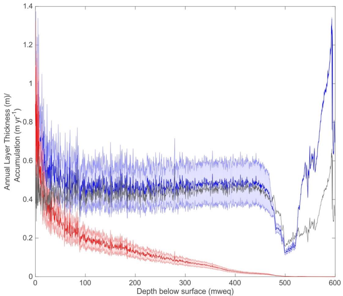
Figure 4.15: As calculated by pRES model: accumulation (original annual layer thickness) profile (blue) with uncertainty (pale blue); present-day annual layer thickness (red) with uncertainty (pale red). An initial accumulation history calculated using the Simple Exponential empirical relationship is shown in grey.
