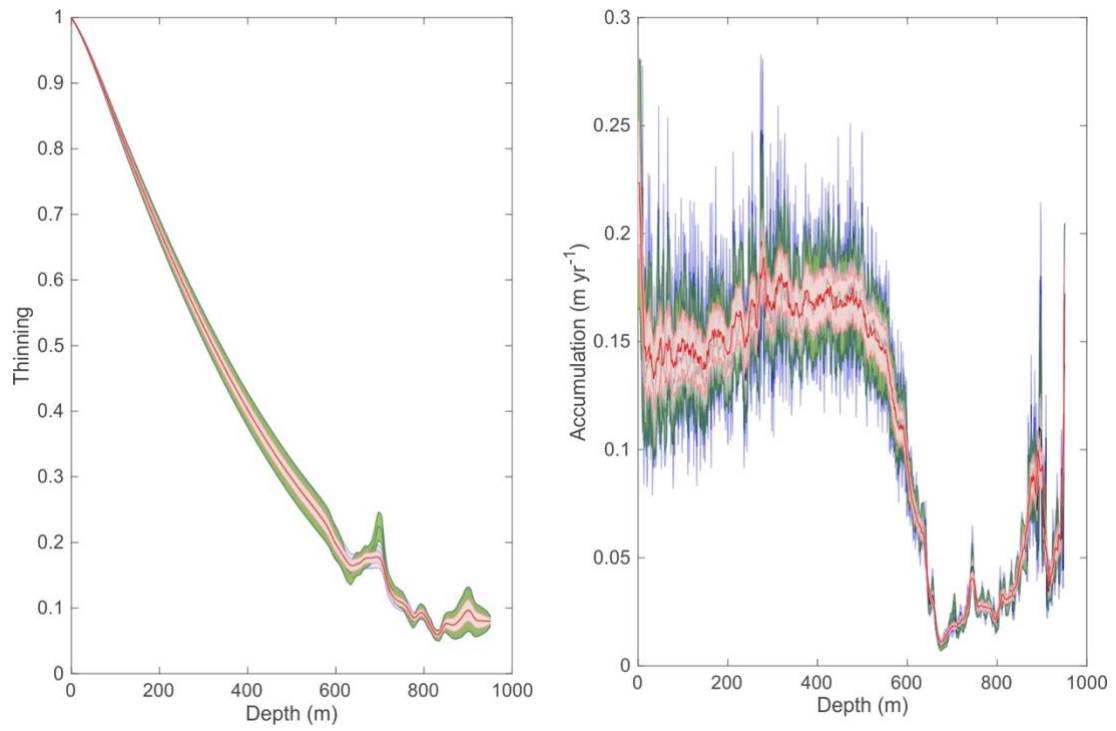
Figure A1.12: Thinning and accumulation reconstructions using the IceChrono model with prescribed thinning functions at 95% confidence interval for the BI ice core. Different initial thinning profiles have been used as an input for this figure and are colour-coordinated as red: Nye; blue: Dansgaard-Johnsen; black: One-Dimensional; green: IceChrono.
