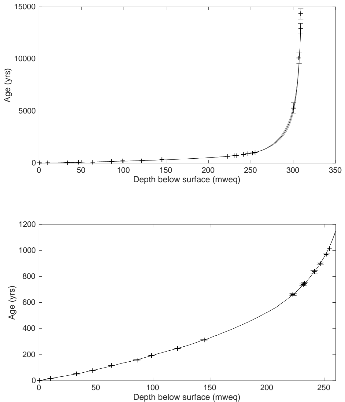
Figure 7.07: (a) Age-depth profile with confidence interval (grey). Black crosses show age horizons (table 7.02) and the associated error of the observational constraints used in the model; (b) A zoom-in of plot (a) to show the most recent 1100 years.
