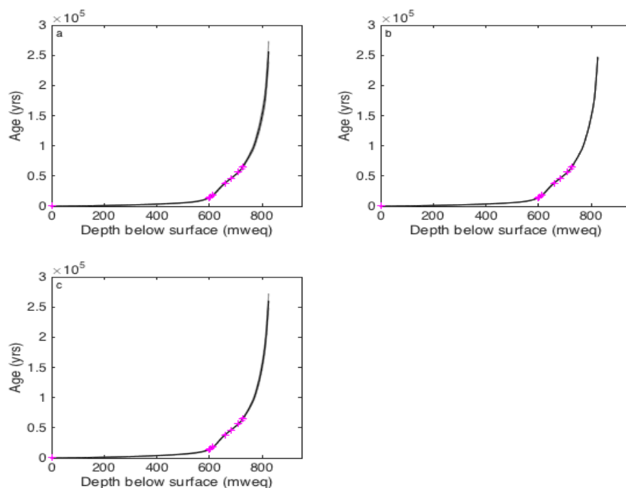
Figure A1.22: Age-depth reconstructions using different initial accumulation profiles and optimised using the Optimised Accumulation and Thinning model for BI, with known-age horizons in pink crosses. Initial accumulation history from top left: (a) Clausius-Clapeyron, (b) Simple Exponential, and (c) Arrhenius.
