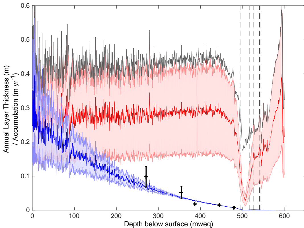
Figure 6.06: Present-day and original annual layer thickness for the FP ice core. Present-day annual layer thickness is assumed to be the product of the final accumulation and thinning profiles. Black crosses show the observed annual layer thickness measurements. The initial Clausius-Clapeyron accumulation history is presented in grey. The depths corresponding to age horizons are delineated by grey dashed lines.
