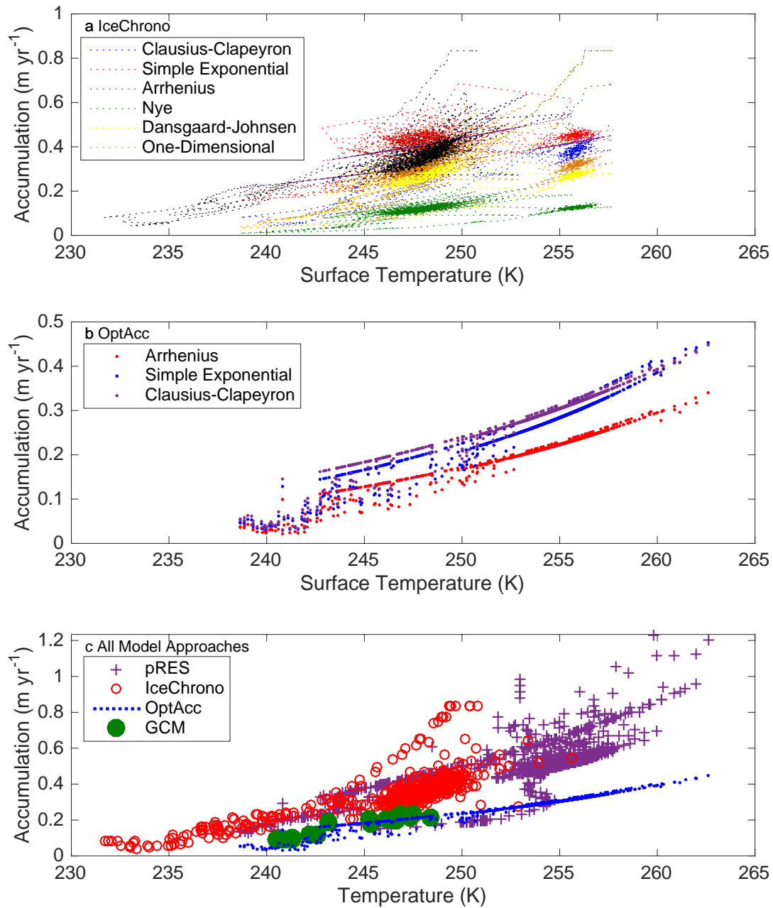
Figure 4.18: Changes in accumulation reconstructed using inverse methods with respect to changes in surface temperature (K) for (a) IceChrono model scenarios; (b) OptAcc model scenarios; (c) all model approaches for comparison.
