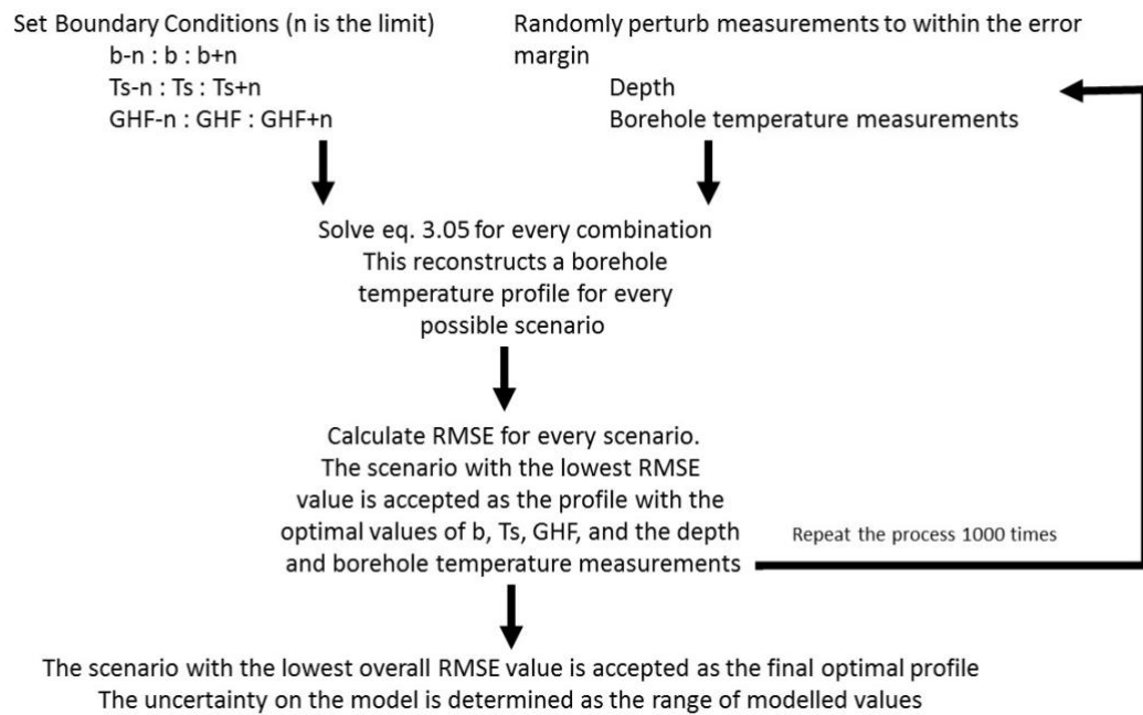
Figure 3.08: Flow chart outlining the methodological approach of the borehole temperature model.
