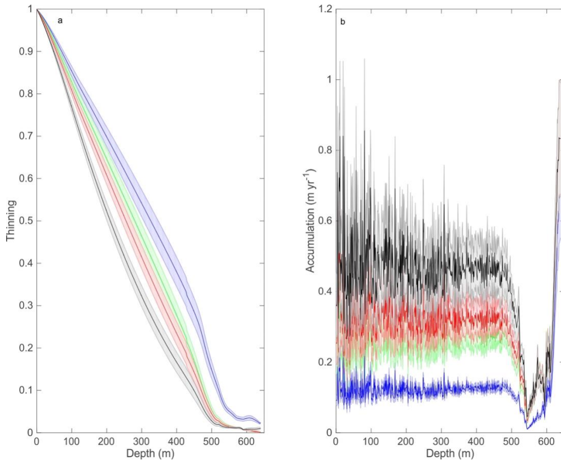
Figure 4.08: (a) Four thinning reconstructions that have been optimised using the IceChrono toolbox, and (b) the associated accumulation profiles for each model scenario. In these model scenarios, boundary thinning functions were fixed with 95% confidence to assess how this constraint would affect the accumulation profile. Optimised profiles are colour-coded for each model scenario. Black: freely-calculated; Blue: Nye; Green: Dansgaard-Johnsen; Red: One-Dimensional, with the associated uncertainty for each profile marked by a lighter shade of the main profile colour.
