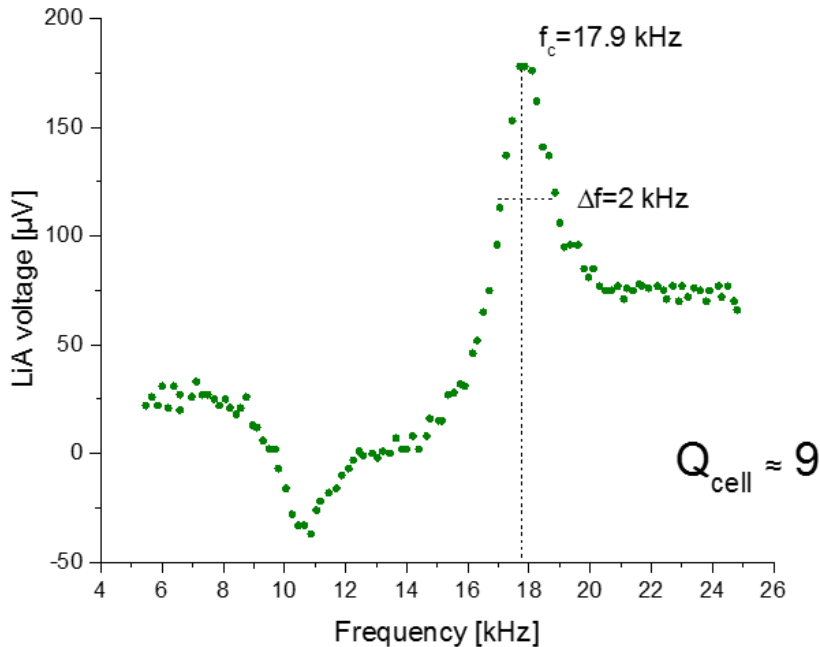
Figure 4. Characteristic of the PAS spectrophone in the intracavity position as the function of the modulation frequency
