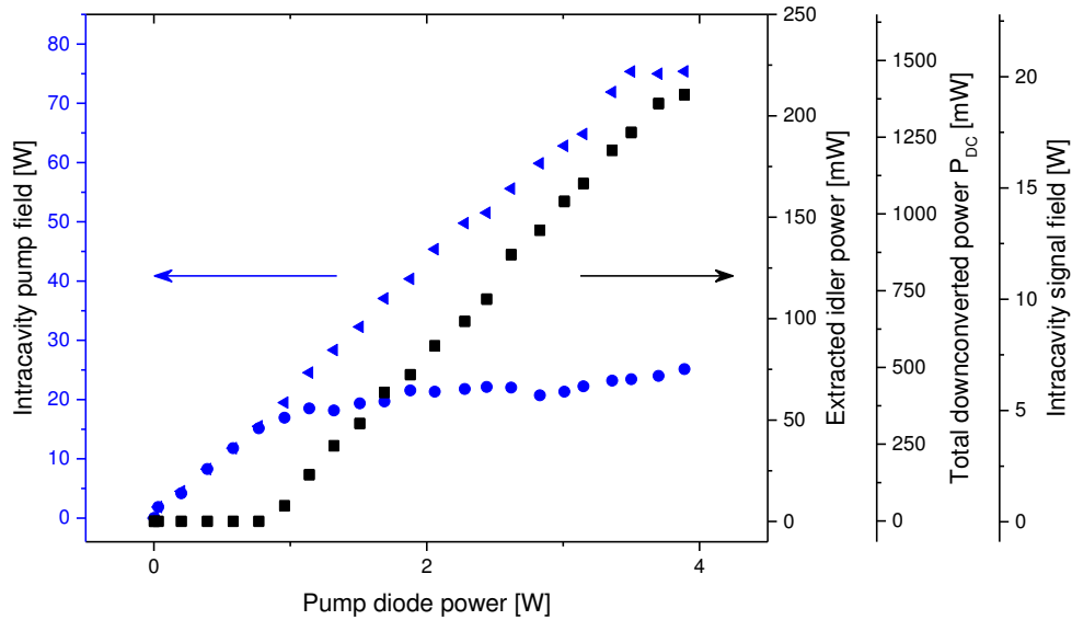
Figure 3. Power characteristics of constructed OPO where blue triangles represent intracavity pump field with OPO not working, blue circles depict the same with OPO working and black squares represent extracted idler power, total down-converted power and intracavity signal field on their respective axes
