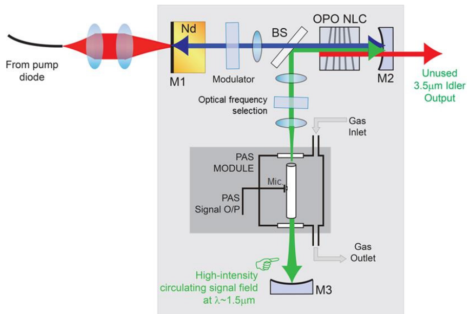
Figure 1. Schematic representation of the signal resonant IC-OPO with an intracavity PAS spectrophone, as developed during this project
