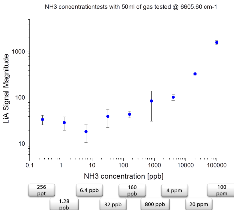
Figure 5. Sensitivity of the system to ammonia on absorption line 6605.6cm -1
