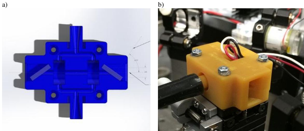
Figure 2. The spectrophone used for this study: cross-section design (a) and fully integrated in the optical setup (b)
