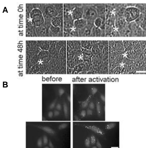
Figure 3. Compound 10 shows low toxicity and photo-activation properties at 20µM in human osteosarcoma cells (U-2 OS) over 48 hours. (A) Short phase contrast timelapse sequence (each 20 mins apart) showed cell division was prevalent at time 0h and after a 48 hour exposure in live U-2 OS cells; *indicates the location of mitosis and the subsequent two daughter cells. (B) Fixed U-2 OS cells labelled with 10 for 1 hr, exposed to a 250ms pulse of excitation light (using a x20 0.8NA lens), excitation 560/40nm and emission
