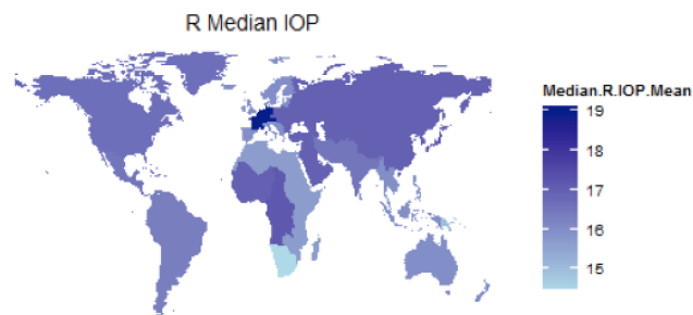
Figure 6: Median OD intraocular pressure by sub-continent
