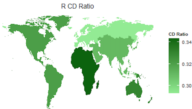
Figure 3: Individual value plots of OD intraocular pressure against continent
