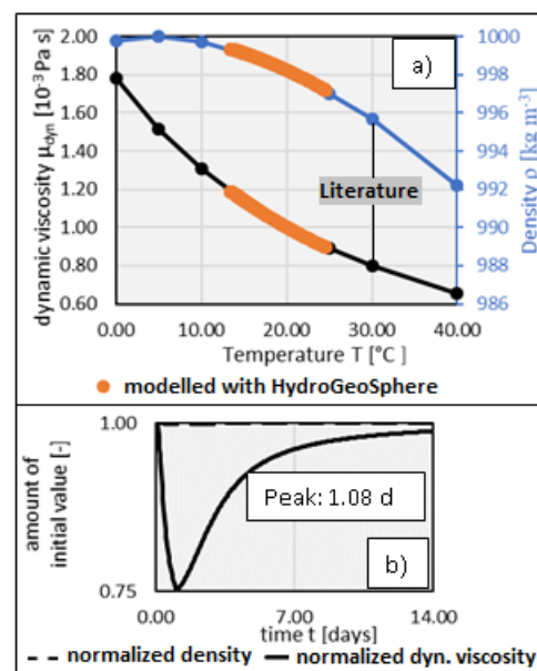
Figure 1: a) Simulated density and dynamic viscosity changes with HGS compared to known literature values. b) Changes (in %) in function of time.
