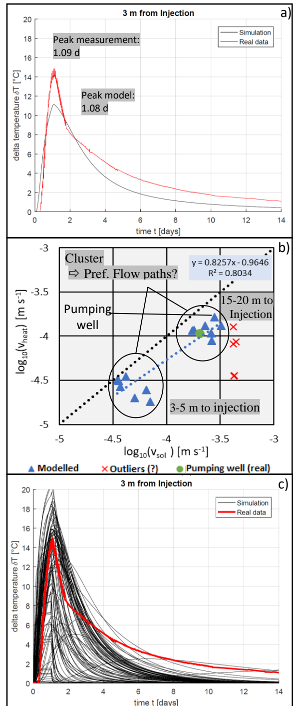
Figure 2: a) Temperature breakthrough with the forward deterministic model. b) Comparison of the heat and solute tracer. c) Temperature breakthrough with 100 simulations of the prior model (BEL).
