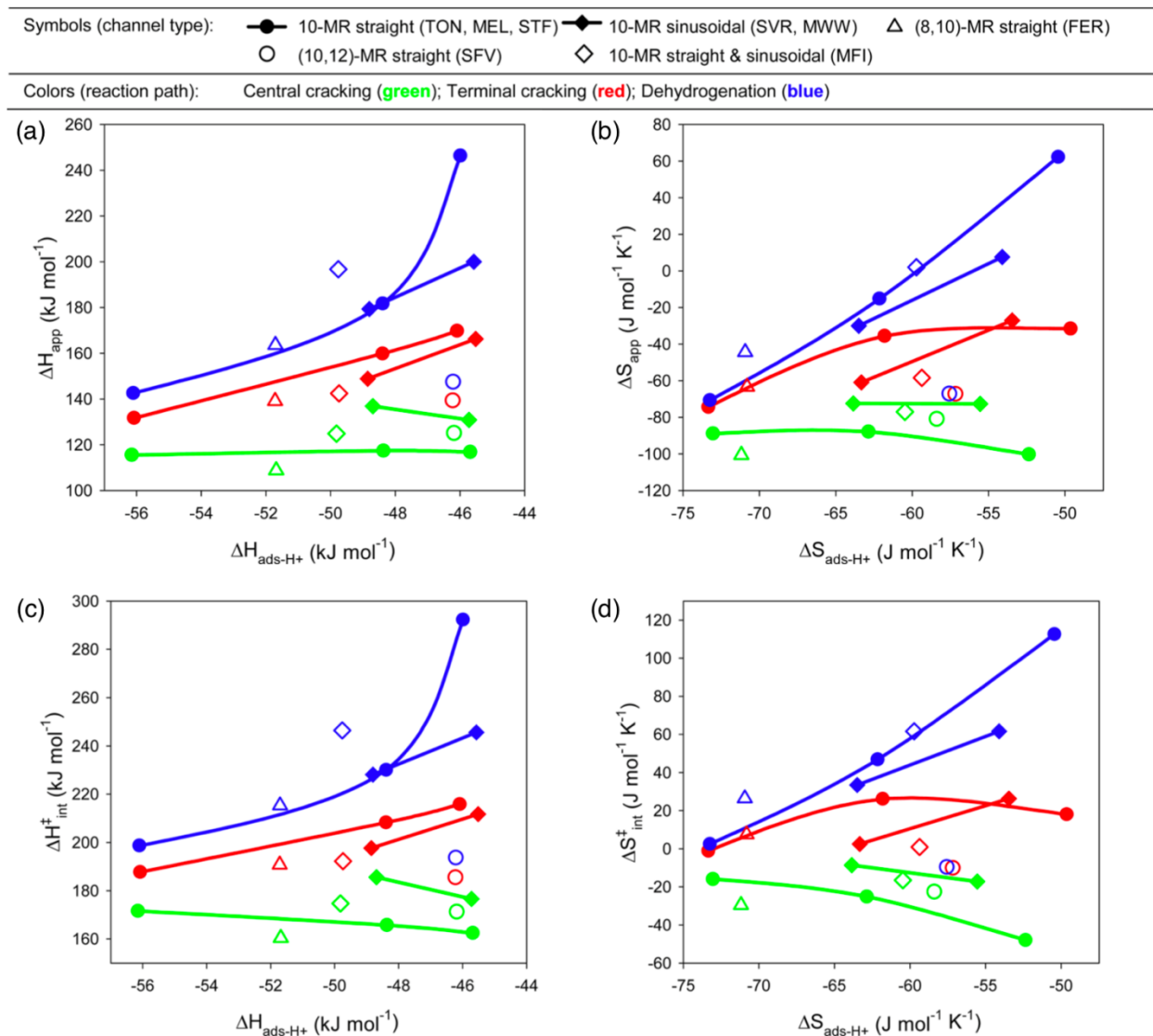
Figure 7. Plots of (a) apparent activation enthalpy vs enthalpy of adsorption, (b) apparent activation entropy vs entropy, (c) intrinsic activation enthalpy vs enthalpy of adsorption and (d) intrinsic activation entropy of adsorption for n-butane monomolecular reactions at 773 K. Values of \Delta H_{ads-H^+} and \Delta S_{ads-H^+} were determined from CBMC simulations, and \Delta H_{app} and \Delta S_{app} from measured rate data. Representative 95% confidence intervals for \Delta H_{app}^\ddagger and \Delta S_{app}^\ddagger are \pm 7 kJ mol -1 and \pm 9 J mol -1 K -1 for cracking, and \pm 8 kJ mol -1 and \pm 11 J mol -1 K -1 for dehydrogenation. Adapted from ref. [9].
