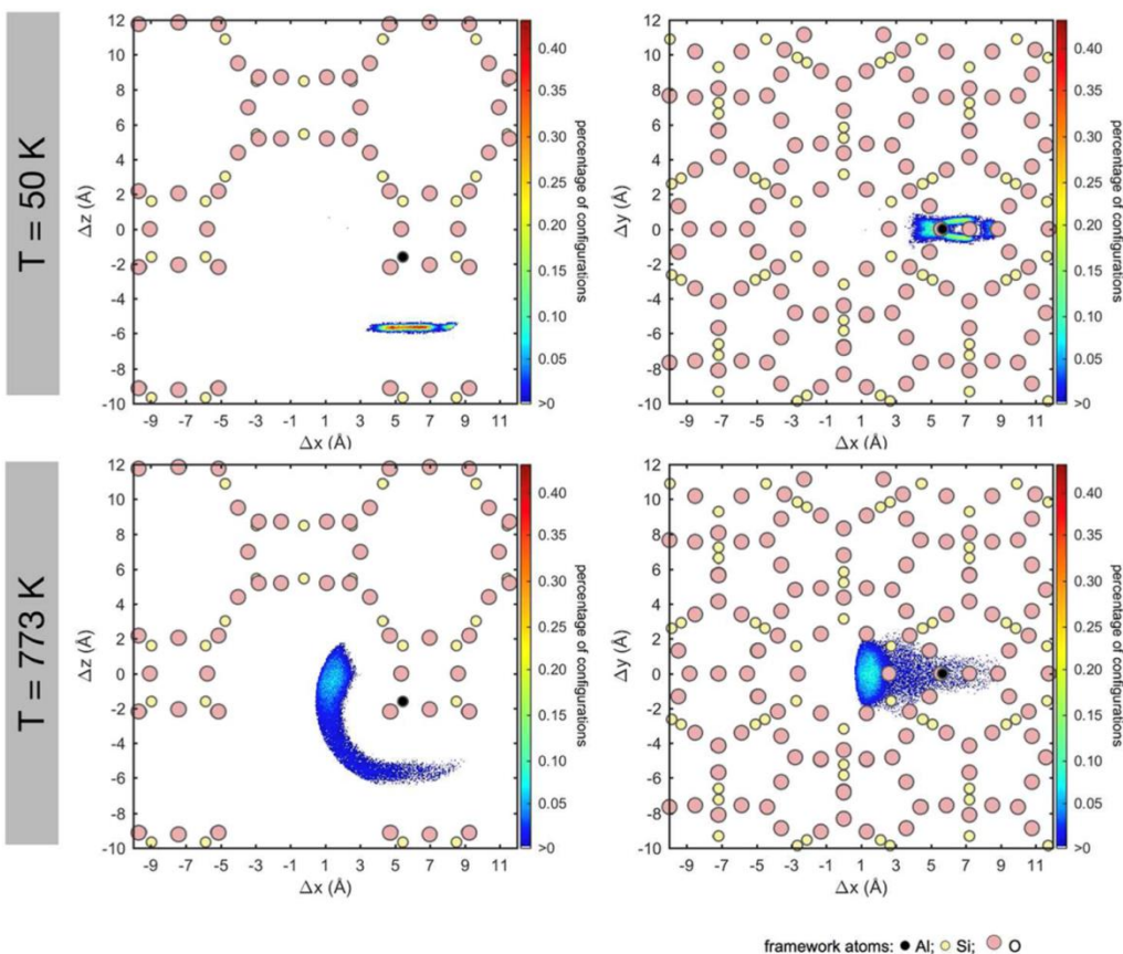
Figure 5. Heat maps showing the distribution of C atoms of the terminal C–C bond of n-butane interacting via this bond with a Brønsted acid site at site T4 in MWW, obtained from CBMC simulations at 50 K and at 773 K. At 50 K, butane is predominantly adsorbed in the sinusoidal channel, while at 773 K, adsorption in the supercage is favored for entropic reasons. Framework atoms outside the plane represented in the heat maps have been omitted for clarity. The color scale represents the percentage of configurations in which the C atom is found within a square with side length 0.05 Å projected onto different planes. Adapted from ref. [31].
