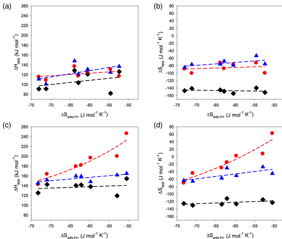
Figure 11. Plots of apparent activation enthalpy (a,c) and entropy (b,d) vs adsorption entropy determined from CBMC simulations for central cracking (a,b) and central dehydrogenation (c,d) of n-butane at 773 K. Experimental values (red circles) are compared with theoretical values determined from QM/MM using the quasi-RRHO approach, before (black diamonds) and after (blue triangles) adding the thermal corrections derived from CBMC simulations. Representative 95% confidence intervals for the experimental values of \Delta H_{app}^\ddagger and \Delta S_{app}^\ddagger are \pm 8 \text{ kJ mol}^{-1} and \pm 11 \text{ J mol}^{-1} \text{K}^{-1} . Adapted from ref. [31] .
