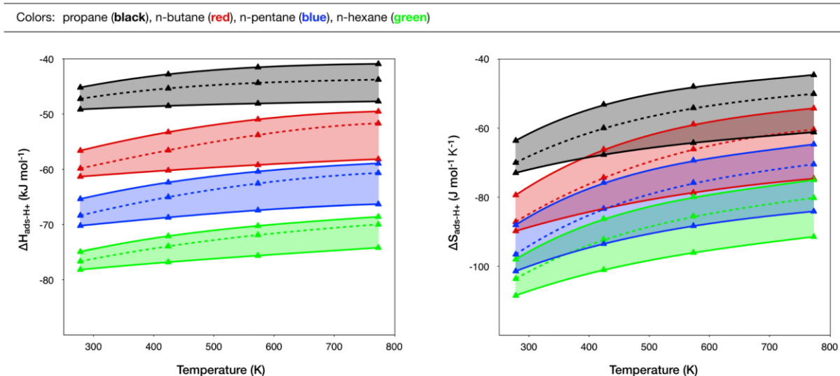
Figure 4. Plots of (a) enthalpy changes \Delta H_{\text{ads-H}^+} and (b) entropy changes \Delta S_{\text{ads-H}^+} for the adsorption of propane (black triangles), n-butane (red triangles), n-pentane (blue triangles) and n-hexane (green triangles) from the gas phase onto Brønsted protons in H-MFI with one Al per unit cell obtained using CBMC simulations. The upper and lower solid lines correspond to Al located only at T9 and T4, respectively. The dashed lines represent the Boltzmann weighted averages of \Delta H_{\text{ads-H}^+} and \Delta S_{\text{ads-H}^+} for Al distributed evenly between T9 and T4. Adapted from ref. [24] .
