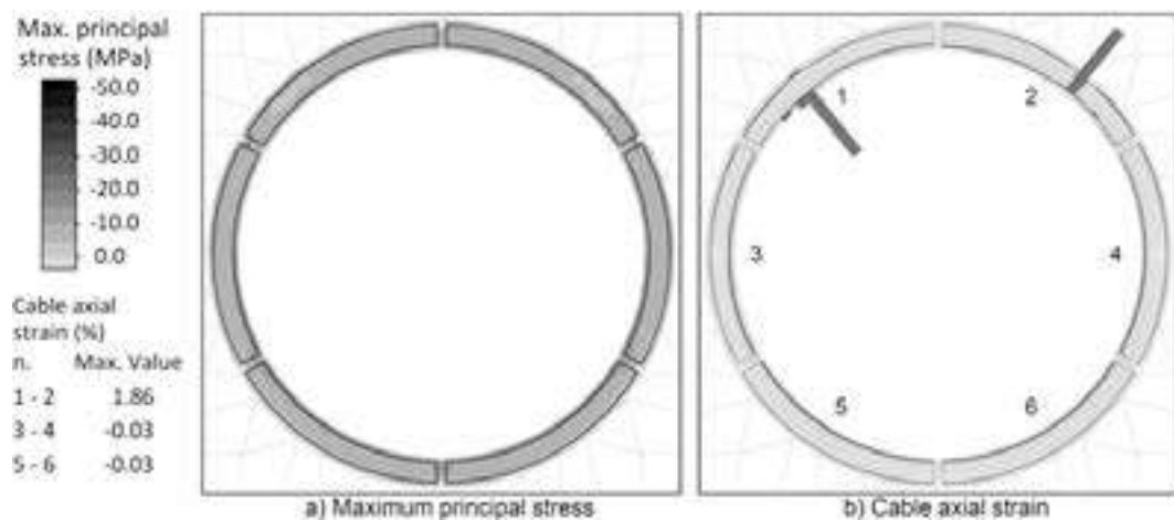
Figure 15. Maximum principal stress contours in the concrete and axial strains in the steel bars with repair.
