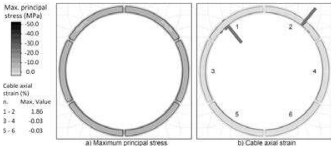
Figure 14. Maximum principal stress contours in the concrete and axial strains in the steel bars without repair.
