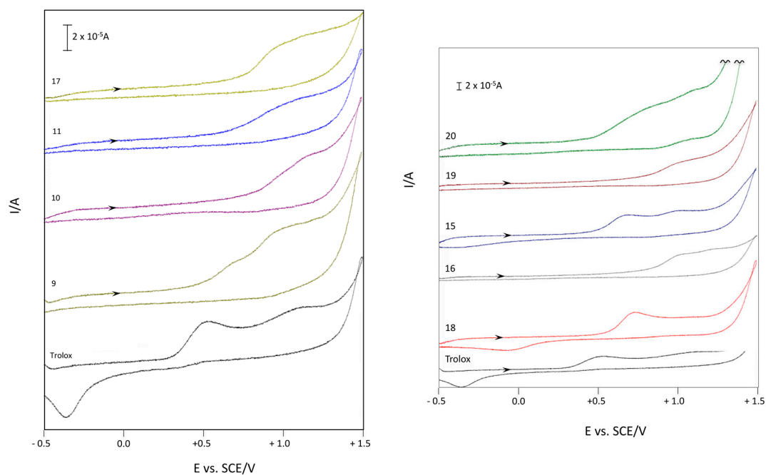
Figure 4. Voltammetric curves of compounds 9–11 and 15–20 ( c = 2 \times 10^{-3} M) in aqueous medium ( \text{H}_2\text{O} -0.5 M NaCl). Starting potential: -0.5 V; reversal potential: +1.5 V (GC working electrode, \nu = 0.2 \text{ V}\cdot\text{s}^{-1} , SCE reference electrode, 25^\circ\text{C} , \text{N}_2 ).
