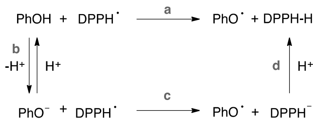
Scheme 1. Reaction involved in the kinetic solvent effects.
