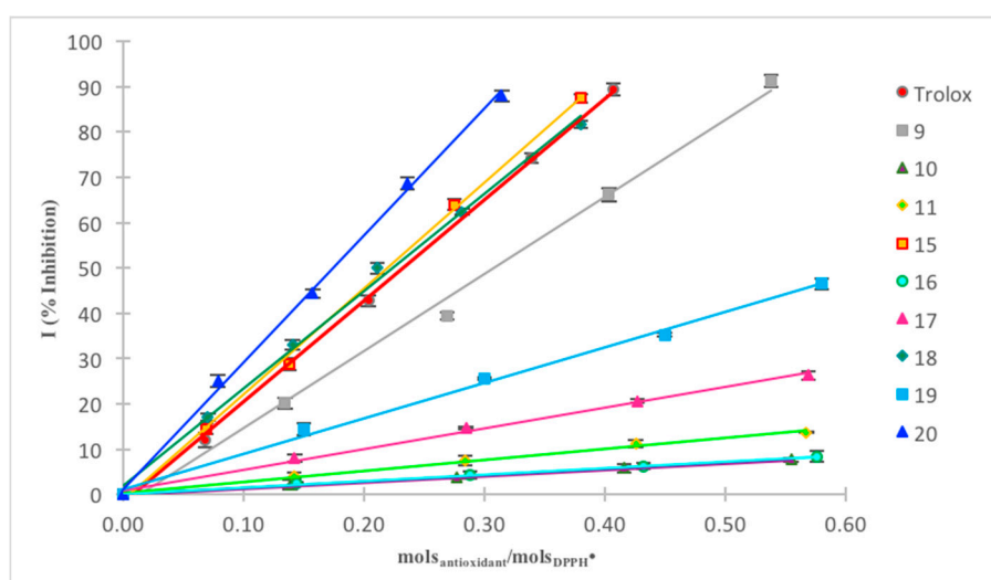
Figure 2. Regression line of the tested compounds 9–11 and 15–20 in DPPH assay in methanol.
