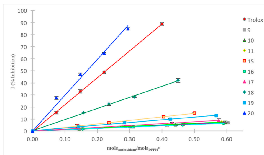
Figure 3. Regression line of the tested compounds 9–11 and 15–20 in DPPH assay in acetonitrile (ACN).
