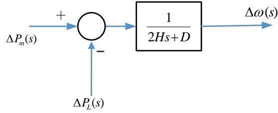
Figure 3.2: Generator-load model in Laplace transform.
