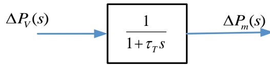
Figure 3.3: Modeling of a non-reheat steam turbine in Laplace transform.
