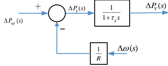
Figure 3.5: Modeling of a speed governor in Laplace transform.
