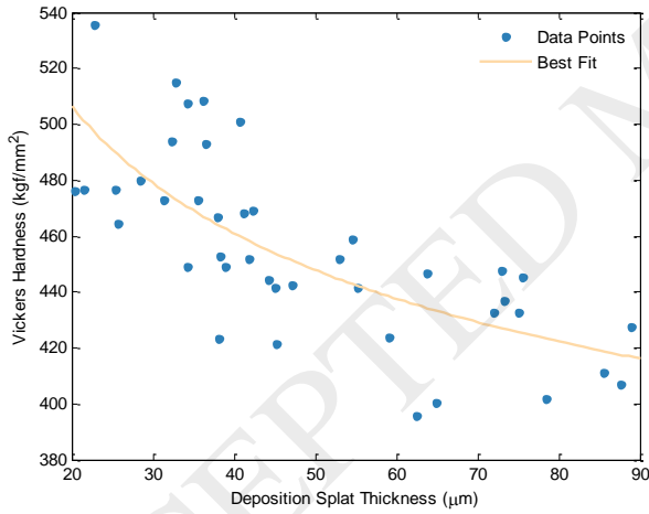
Figure 7. Vickers hardness for various deposition splat thicknesses
