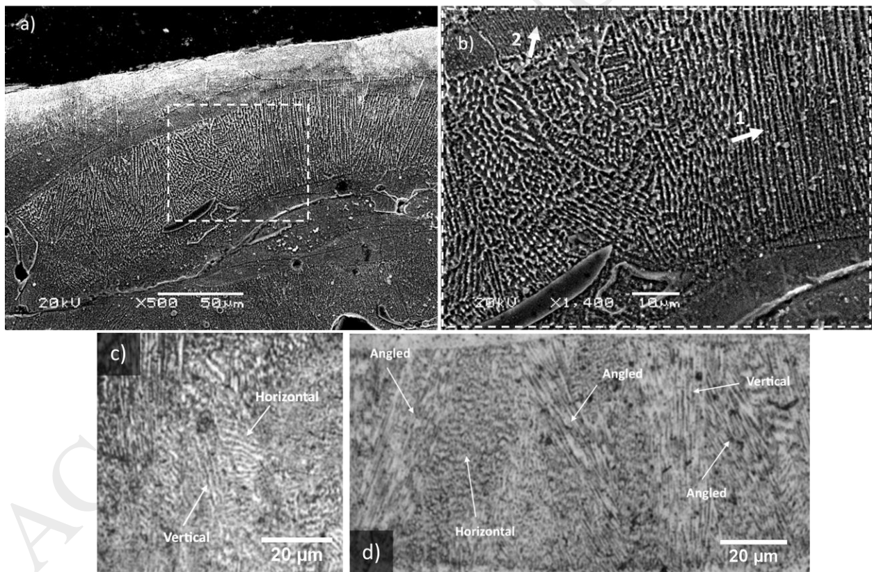
Figure 3. a) SEM image of deposition with cellular dendritic subgrain, b) area of interest, and OM images of competing cellular growth directions in c) a 100 \mu\text{m} thick splat and d) a 70 \mu\text{m} thick splat
