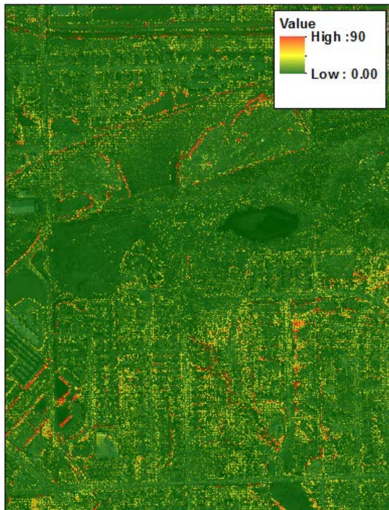
Figure 4: Slope Raster
