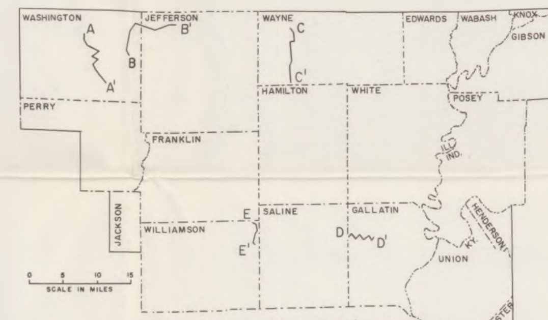
Index map showing location of cross sections (see plate 1 for relation to distribution of channels)
