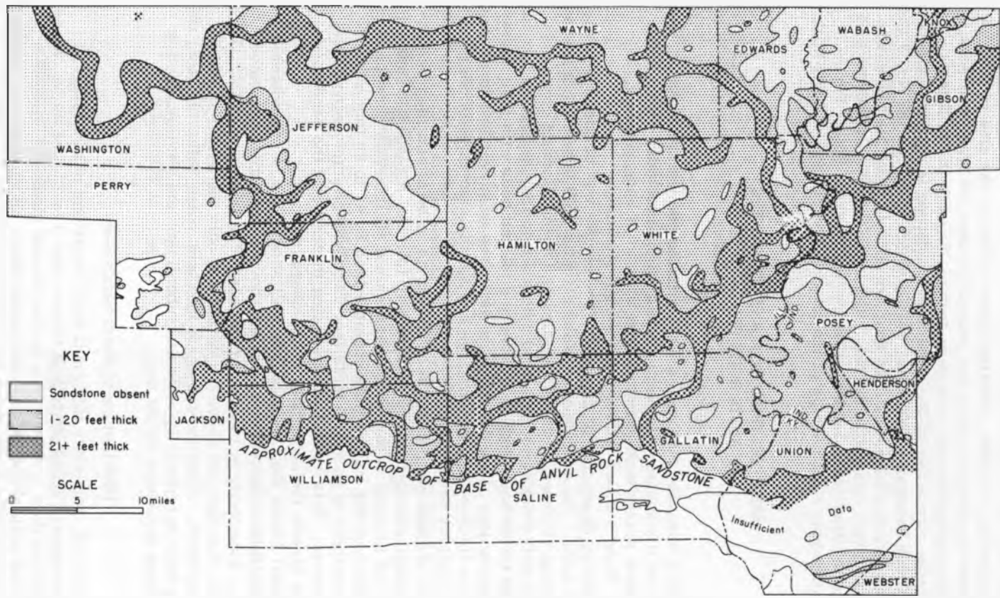
Fig. 4. - Generalized distribution and thickness of Anvil Rock Sandstone in southern Illinois, southwestern Indiana, and western Kentucky.
