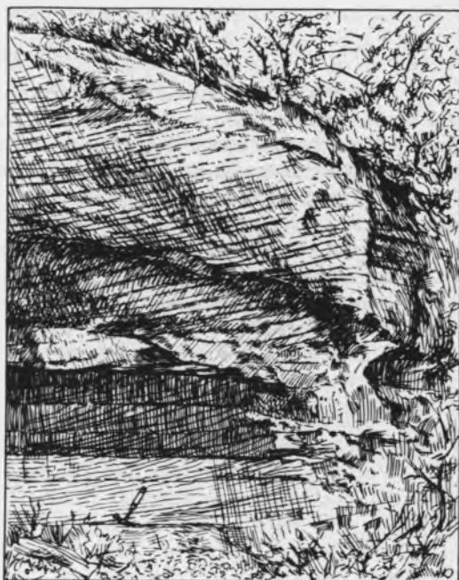
Fig. 14. - Cross-bedding in the channel phase of the Anvil Rock Sandstone, Gallatin County, Illinois.
