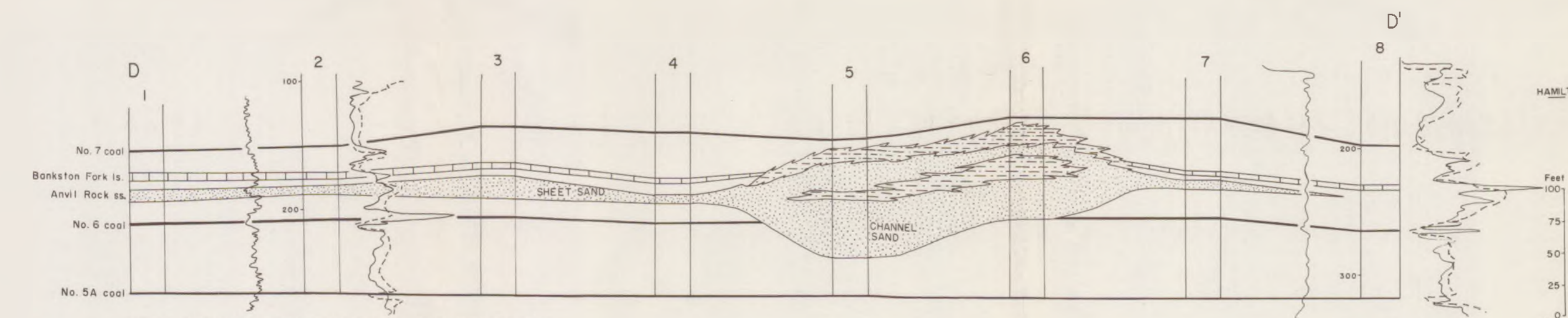
Section across major channel in Gallatin County, datum No. 5A coal.
