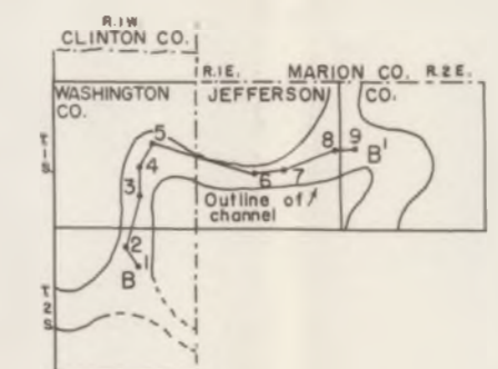
Index map showing location of cross sections (see plate 1 for relation to distribution of channels)
