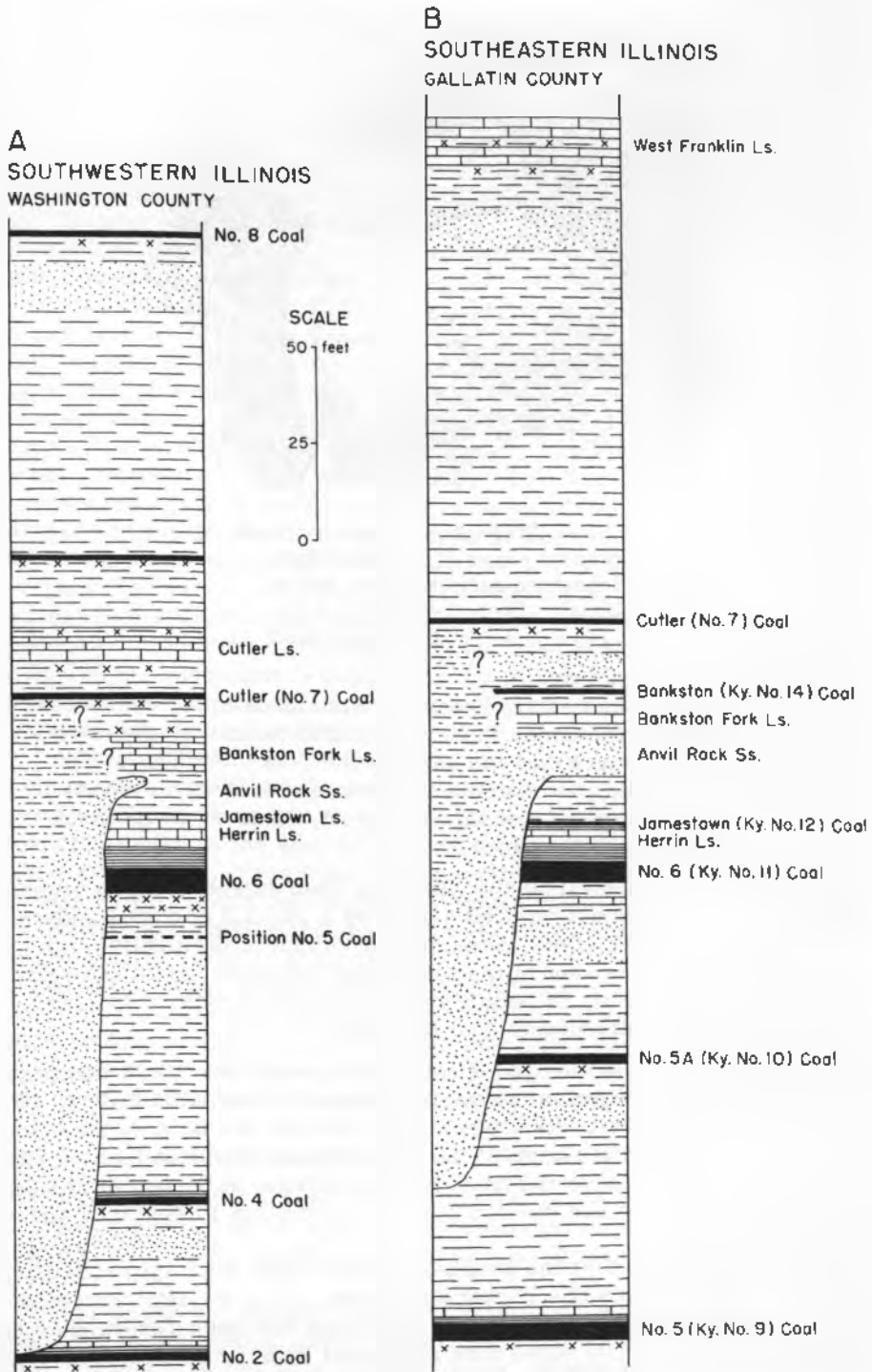
Fig. 3. - Generalized stratigraphic sections of upper Carboniferous and lower McLeansboro strata in southwestern and southeastern Illinois.
