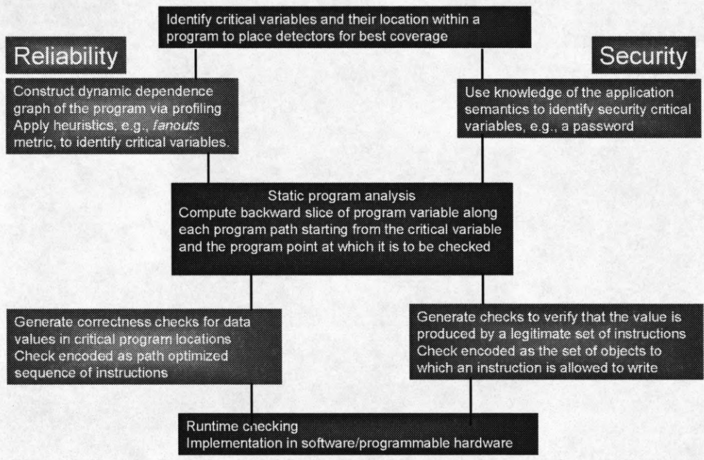
Figure 1: Steps in Compiler-based Static Analysis presented as part of a compiler-based security and reliability framework
