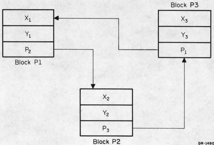
Linked List of Three Blocks Figure 2.1
