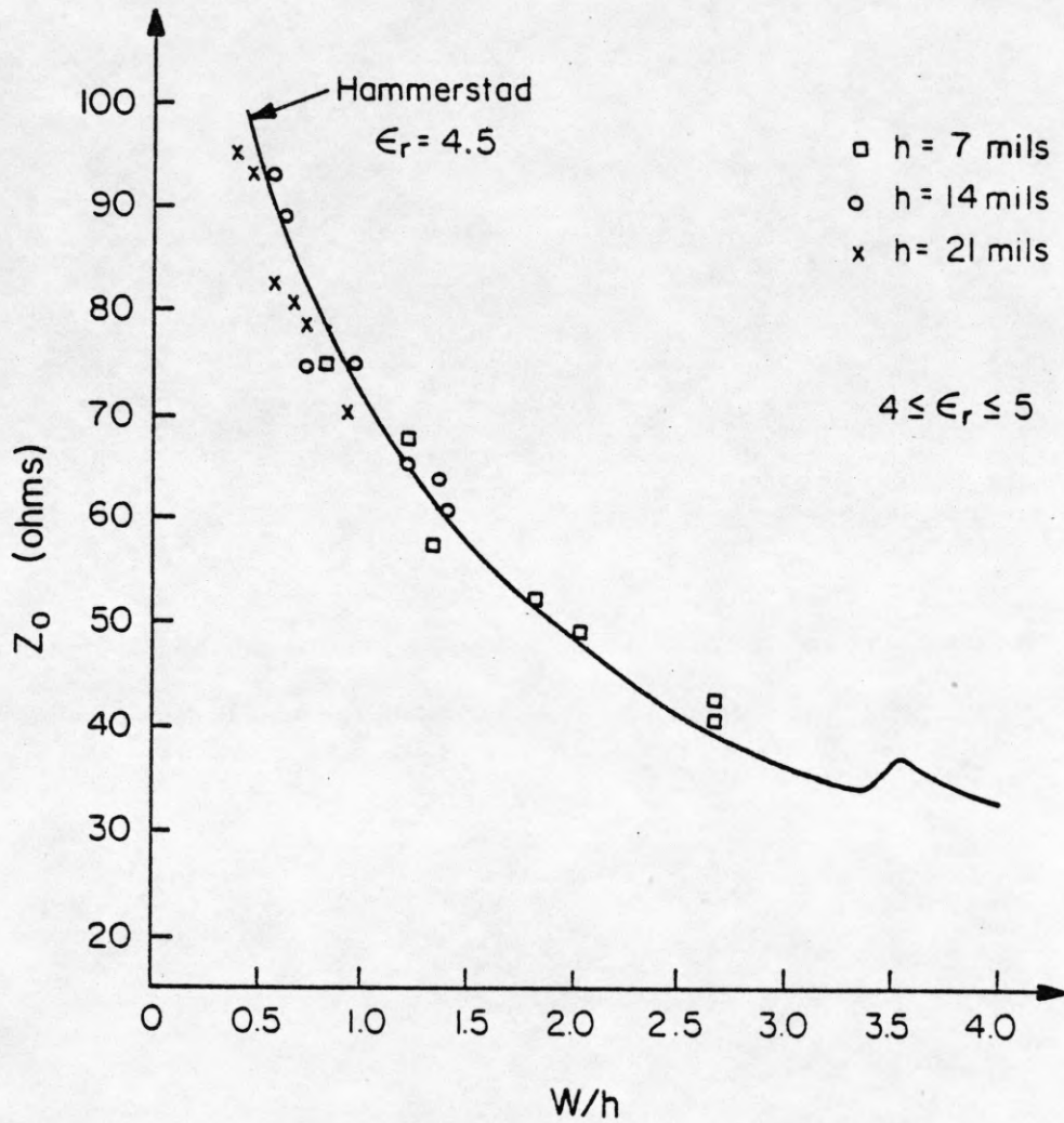
Figure 1.2 : Characteristic impedance Z_0 versus width to height ; W/h . Solid line : theoretical expressions from Hammerstad with \epsilon_r = 4.5 ; points: experimental measurement using time domain reflectometry. For the experimental points, the lines have a dielectric constant 4 \leq \epsilon_r \leq 5 .
