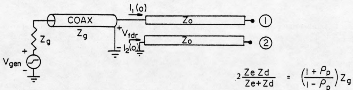
(b) "PARALLEL" CONNECTION
