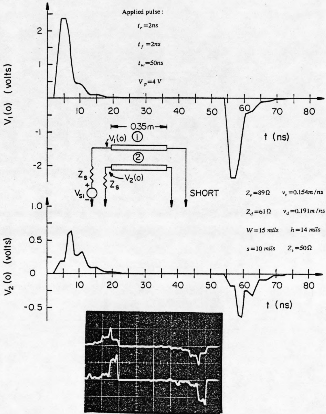
Figure 3.3 : Cross-coupling for passive terminations with far end shorted. Theoretical (plot) and actual (photograph) waveforms. Photographs : top waveform is V_1(o) (driving line) with vertical : 1V/div , bottom waveform is V_2(o) (idle or sense line) with vertical : 0.5V/div . Each horizontal division is 5ns .
