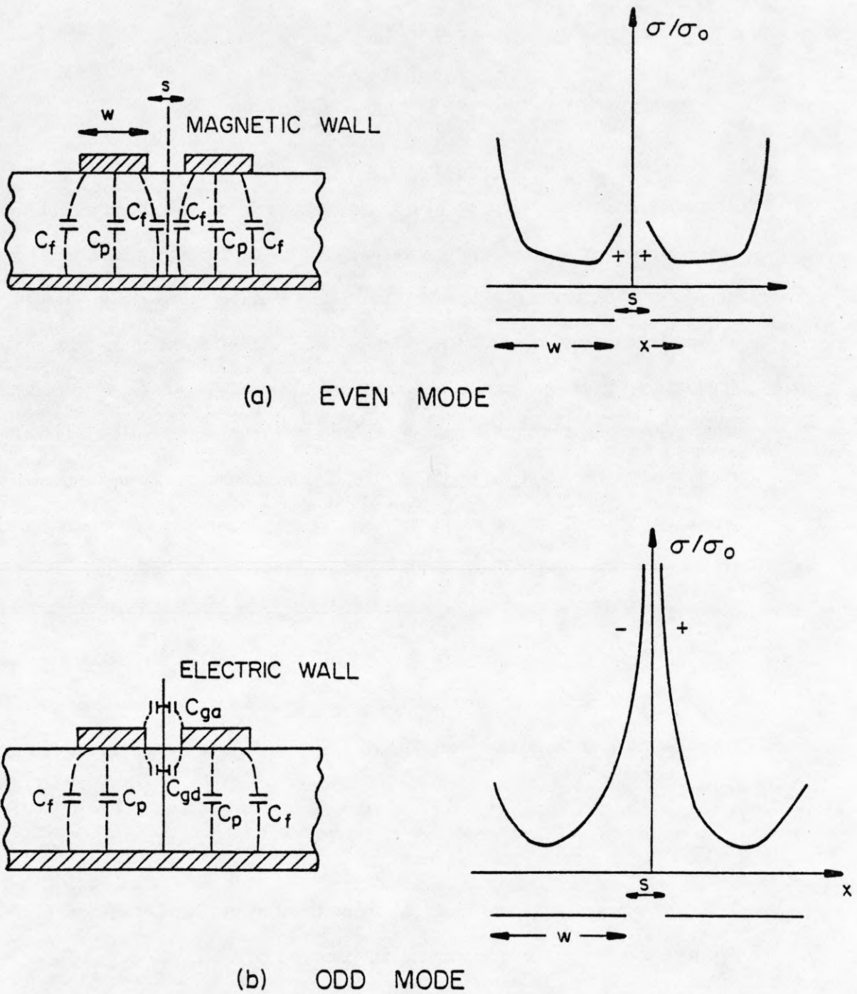
Figure 2.4 : Decomposition of the capacitances into odd and even mode components. C_p represents the capacitance associated with the TEM propagation mode; C_f is the fringing capacitance. C_{ga} and C_{gd} are the mutual capacitances in air and in the dielectric, respectively. The normalized charge distribution associated with each mode is shown on the right with \sigma_0 being the charge at the center of each strip.
