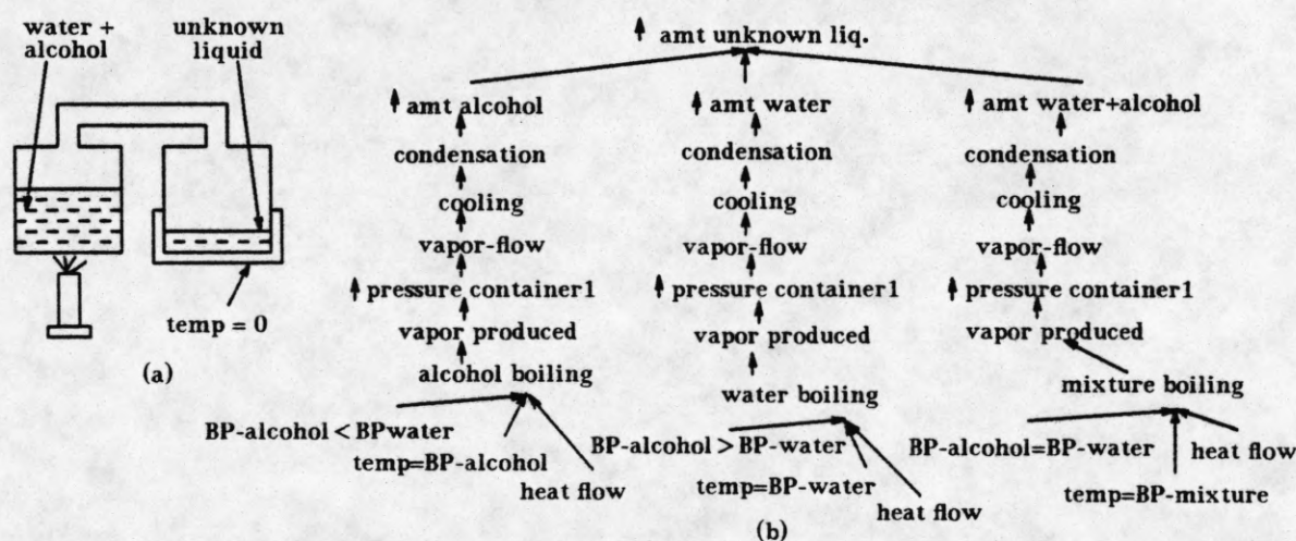
Figure 2: An example illustrating the multiple explanations problem due to incomplete knowledge.
