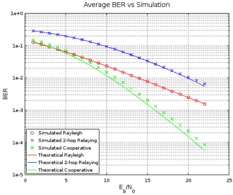
Figure 2.2: \bar{P}_\epsilon in Cooperative Communication ( \sigma_{SR}^2 = \sigma_{SD}^2 = \sigma_{RD}^2 = 1 )
