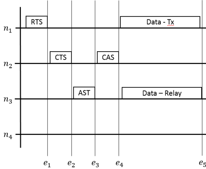
Figure 3.5: Handshaking Between Nodes with Cooperation in \mathbf{G}_1
