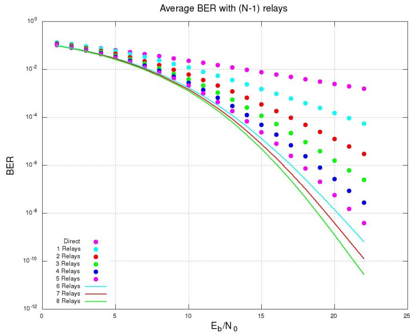
Figure 2.3: \bar{P}_\epsilon in Cooperative Communication with Multiple Relays
