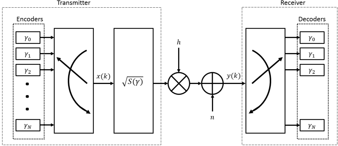
Figure 2.6: Channel State Based Encoding/Decoding Architecture
