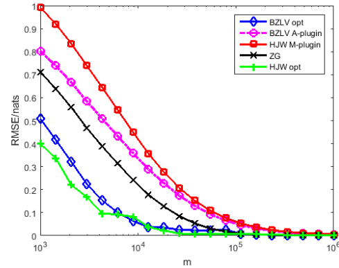
Figure 5.1: Comparison of five estimators under traditional setting with k = 10^4 , m ranging from 10^3 to 10^6 and n \asymp f(k)m .
