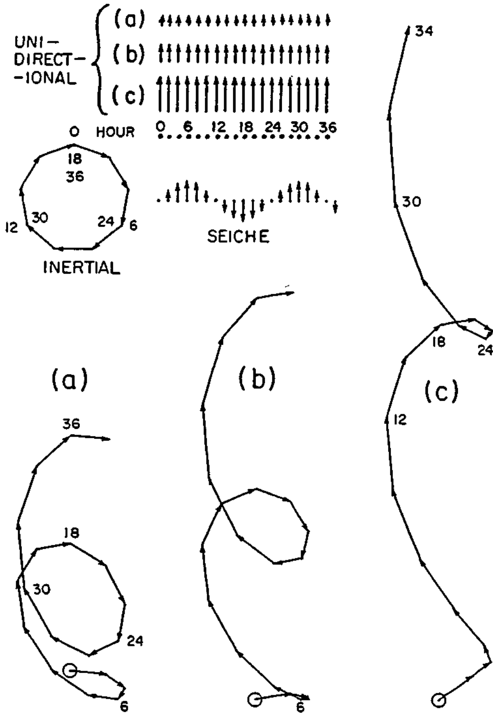
Figure 28. Vector combination of a rotating inertial current, a seiche current, and unidirectional current components of three speeds (From Mortimer, 1978)
