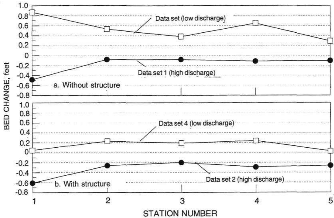
Figure 12. Effects of high and low discharges on bed changes without the control structure (a) and with the structure (b)
