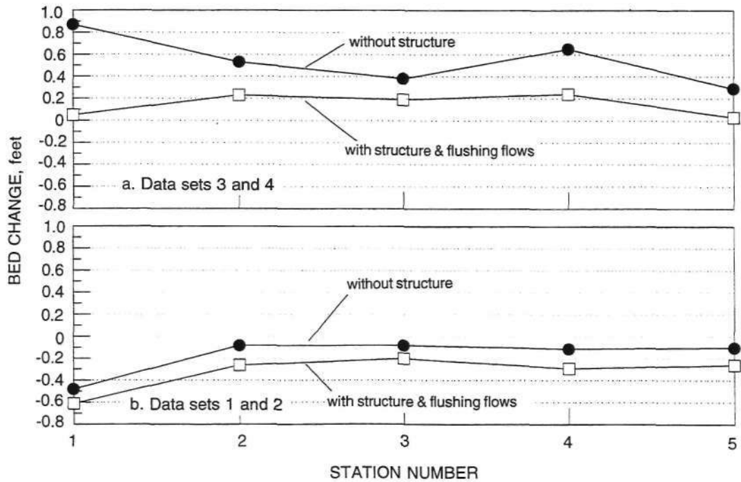
Figure 13. Effects of low discharges (a) and high discharges (b) on bed changes, both with and without the structure
