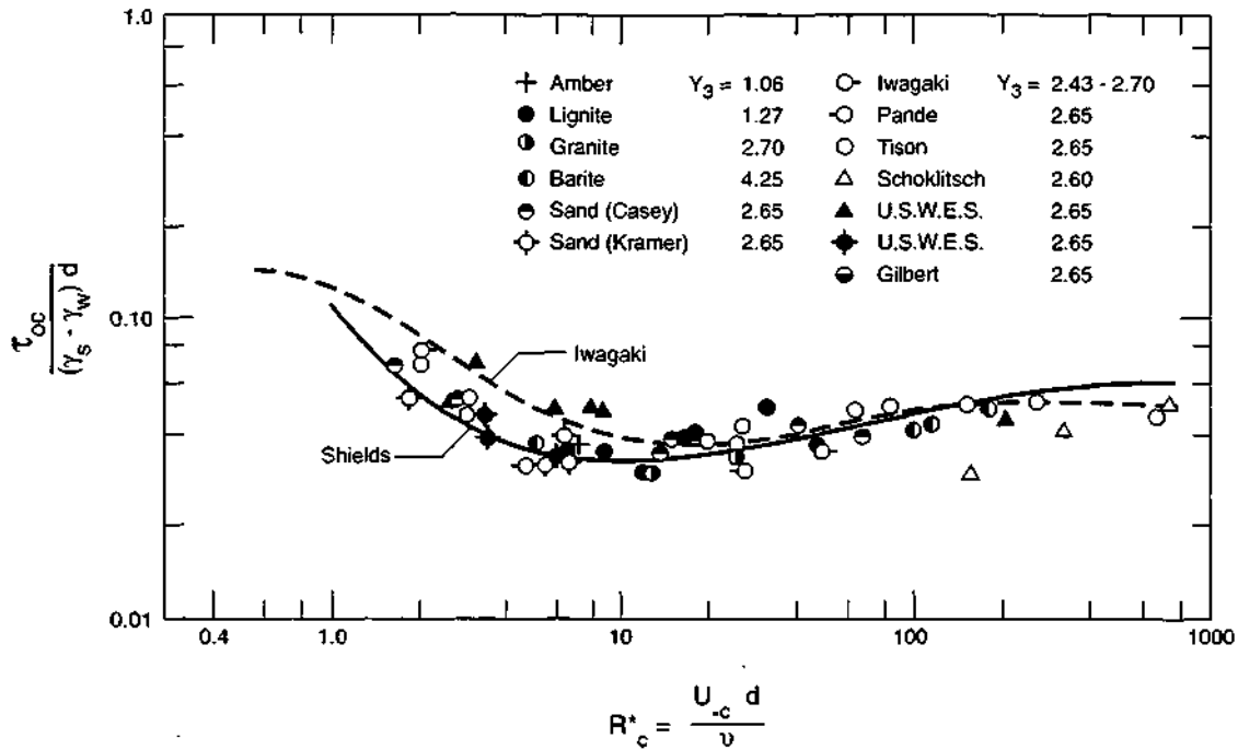
Figure 8. Variation of \frac{\tau_{oc}}{(\gamma_s - \gamma_w)d} with R_c^* obtained by Shields (1936)
