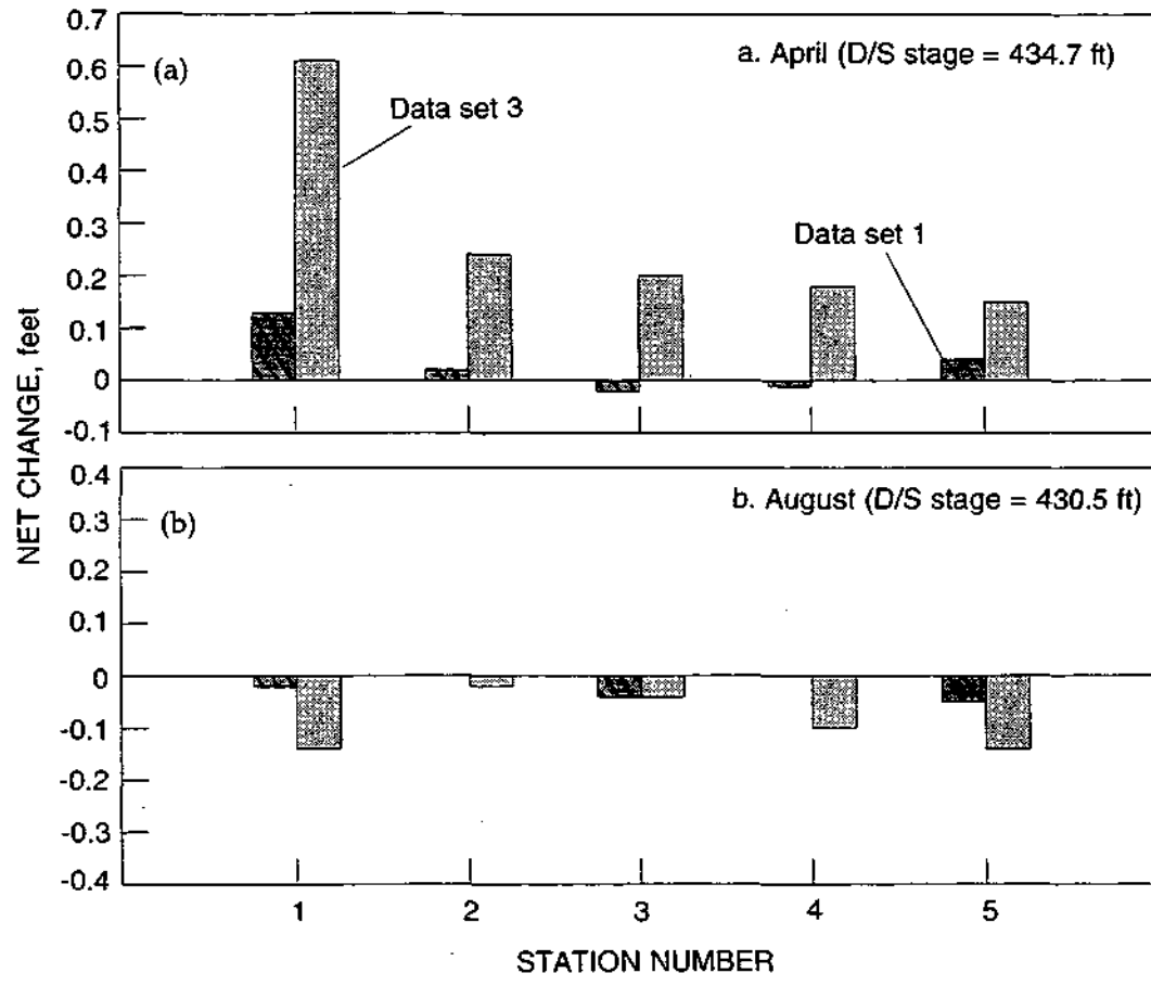
Figure 11. Effect of downstream stages on sedimentation patterns in April (a) and August (b)
