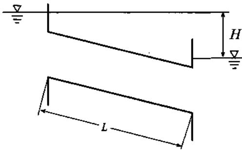
c. Full: outfall submerged, pipe flow
