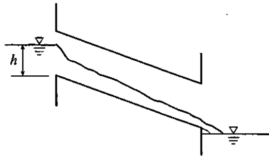
e. Inlet not submerged: inlet controls, weir flow
