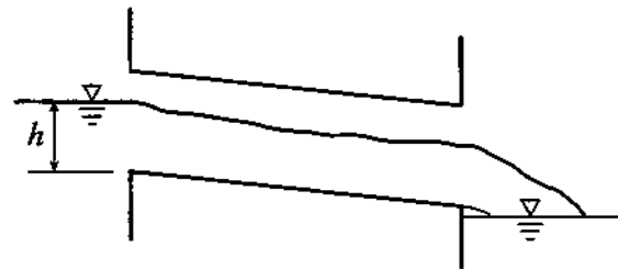
d. Inlet not submerged: conduit controls, open channel flows
