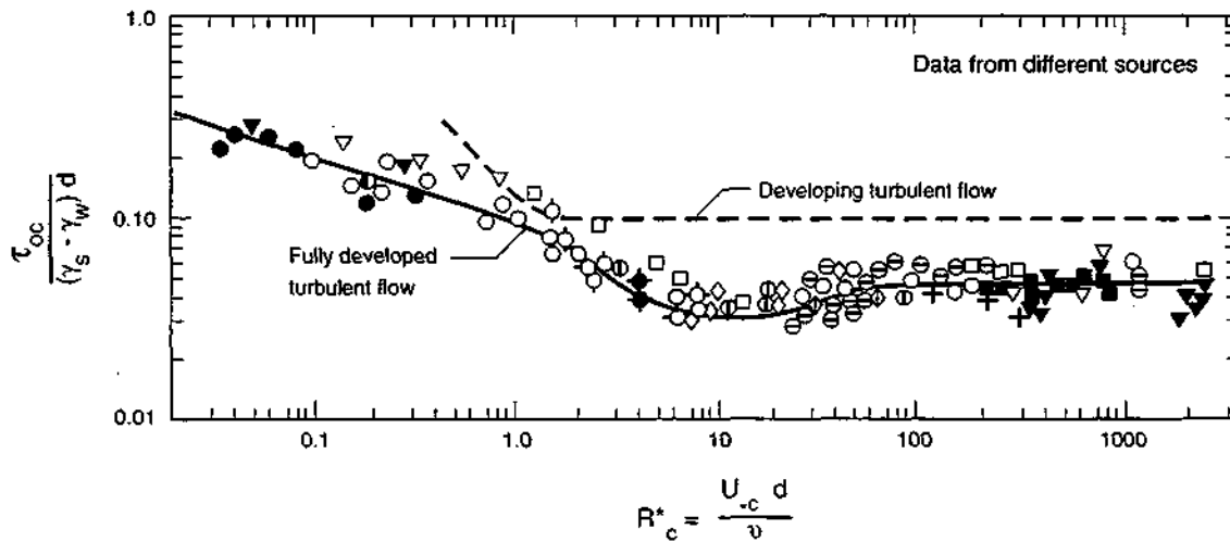
Figure 9. Variation of \frac{\tau_{oc}}{(\gamma_s - \gamma_w)d} with R_c^* obtained by Yalin and Karahan (1979)
