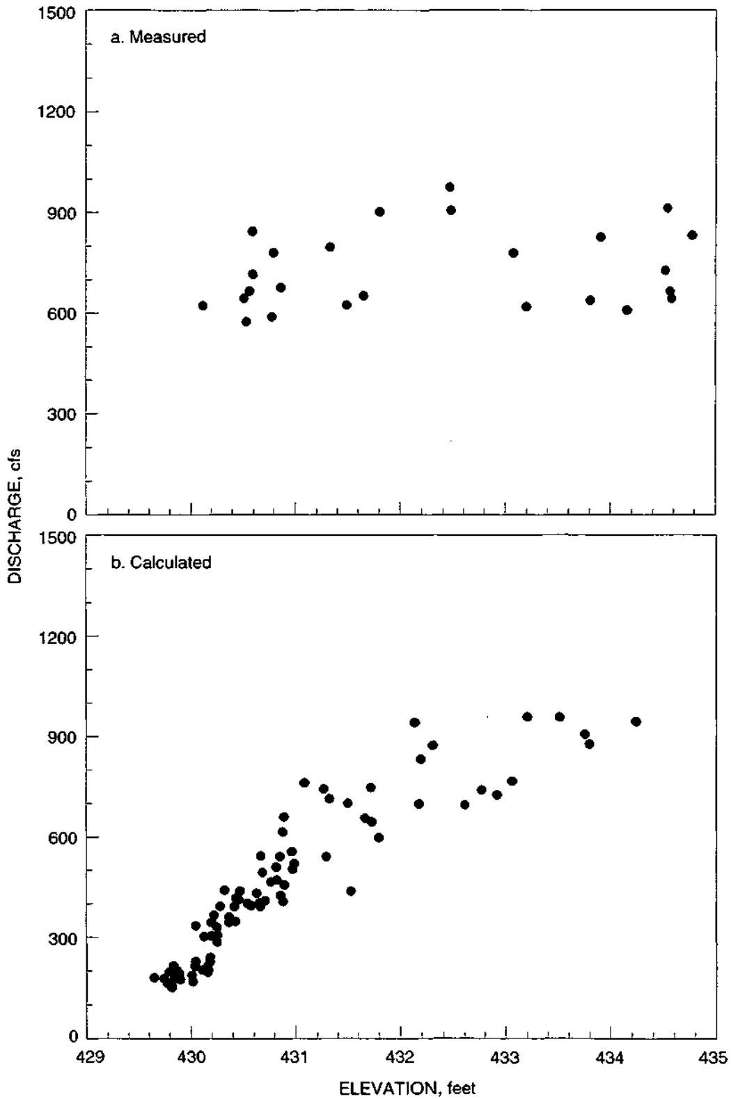
Figure 7. Relationship between water surface elevation at RM 98.8 and discharge measured by INHS (a) and discharge calculated by equation 2 (b)
