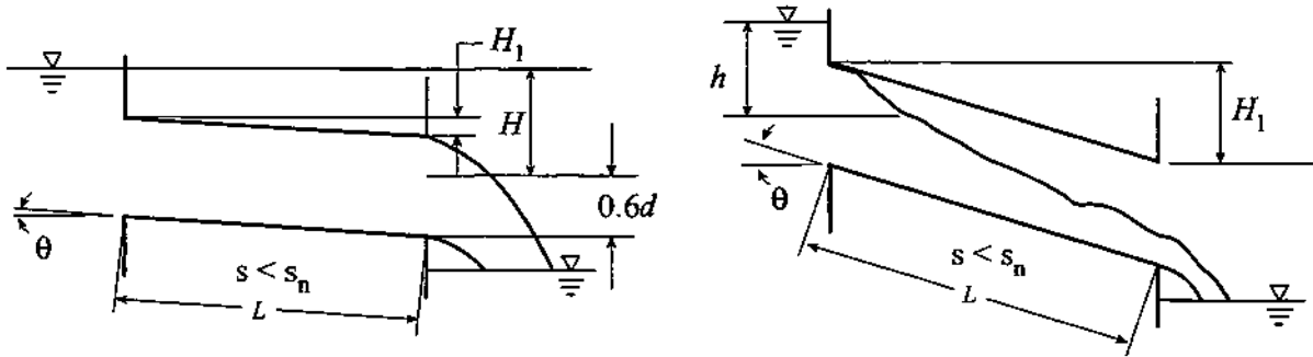
a. Full: free outfall, pipe flow
