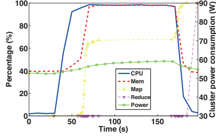
Figure 14: Estimate pi on Edison cluster.
