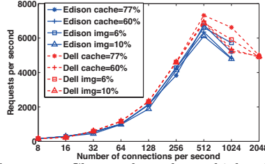
Figure 5: Cluster throughput, higher image percentage and lower cache hit ratio.
