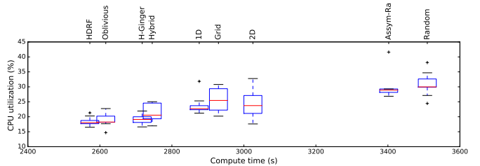
(b) K-core
