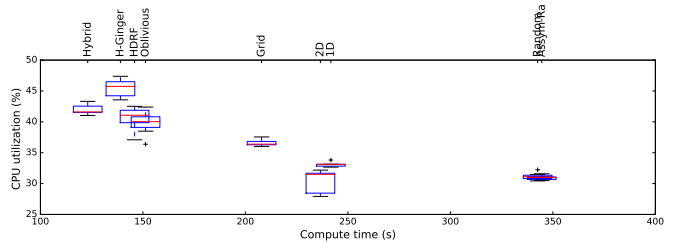
(a) PageRank
