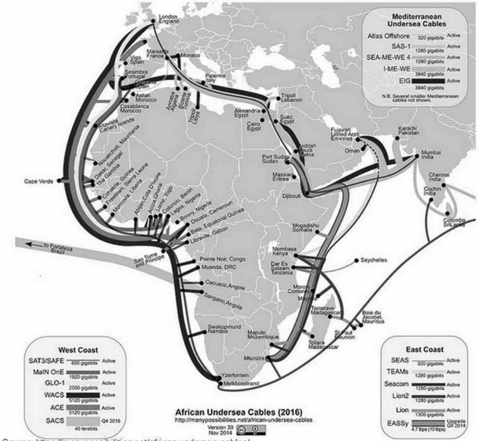
Figure 1. African undersea cables (2016). Map courtesy of Steve Song.
